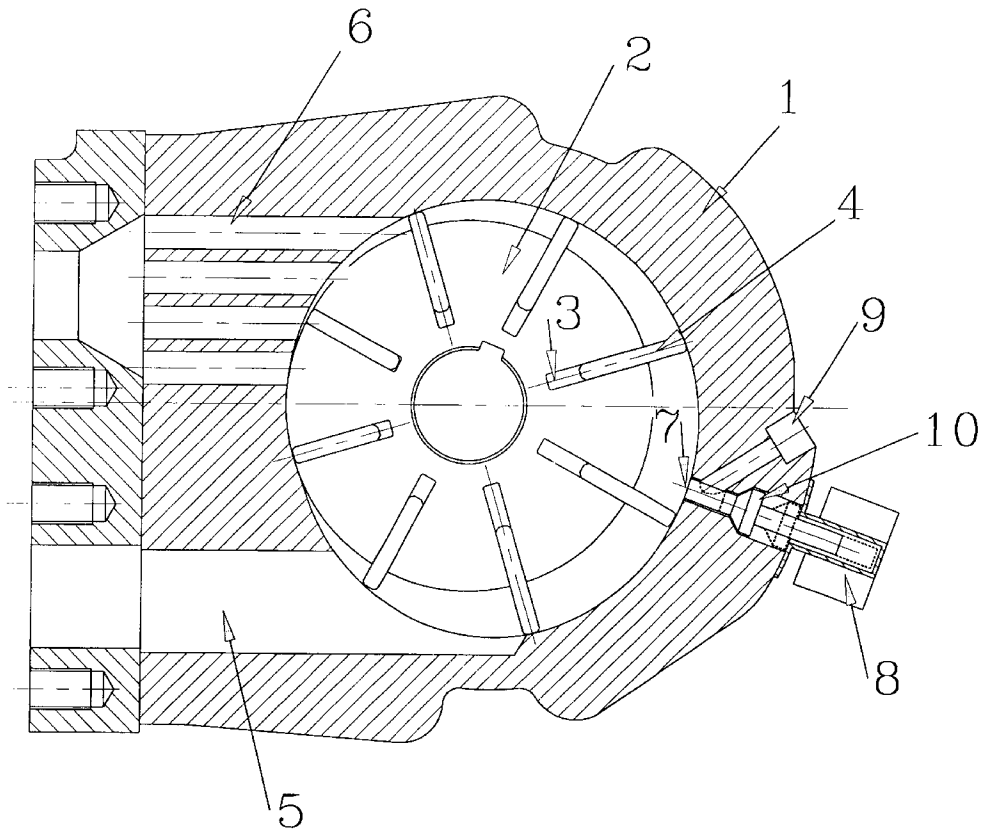
ROTARY VANE COMPRESSOR
