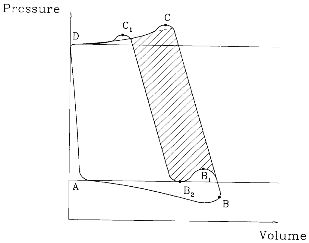
FIGURE 2: CYCLE OF ROTARY COMPRESSOR
