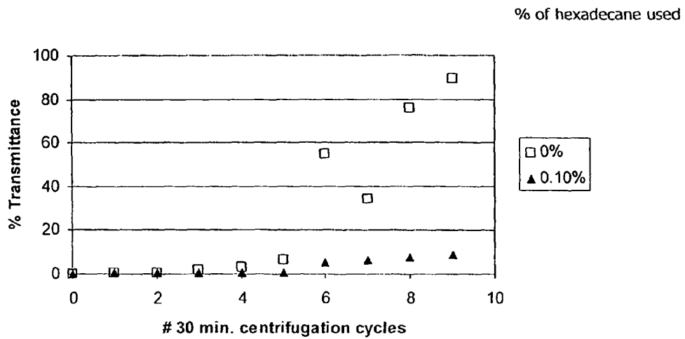
Figure 1. Effect of increasing levels of poly (1-vinylpyrrolidone)-graft 1-hexadecane on the stability of a titania suspension
