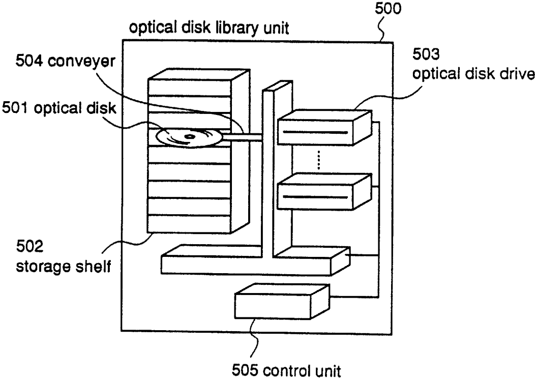
Fig.28 Prior Art
