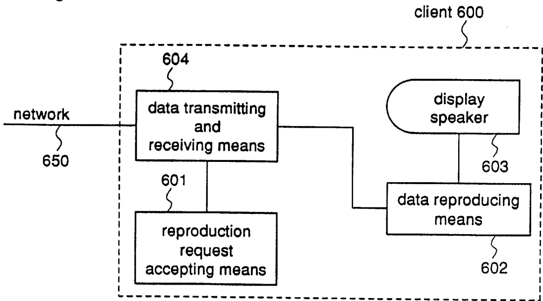
Fig.30 Prior Art
