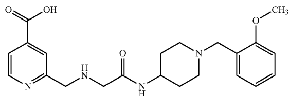
Synthetic Route E
