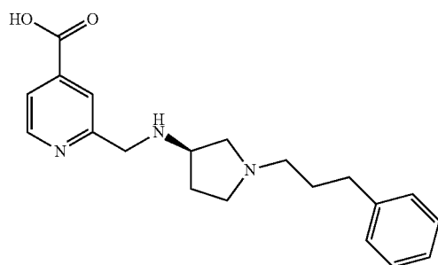
Synthetic Route D
