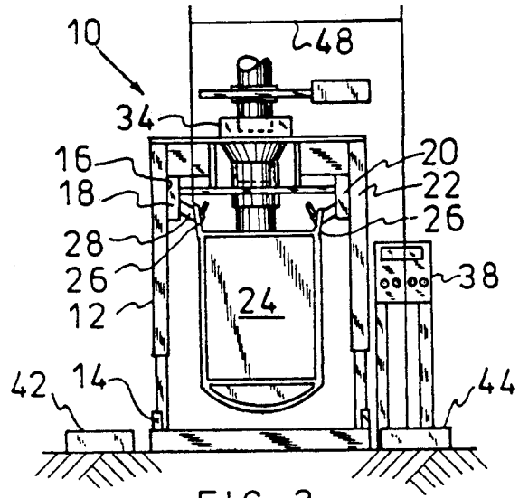
FIG-2 PRIOR ART
