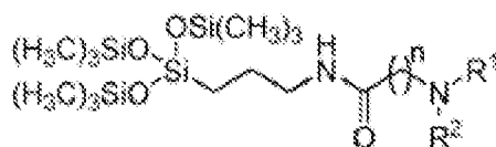
Formel I
