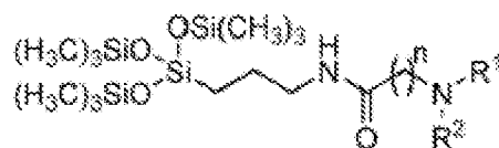
Formular I
