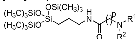
Formula Ib
