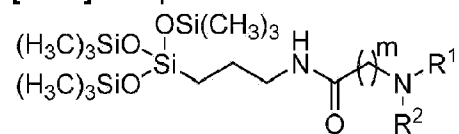
Formula Ia
