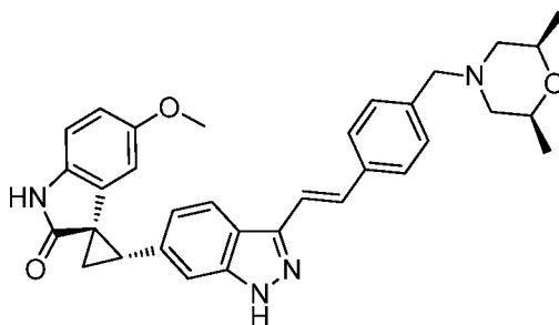
Compound (I)
