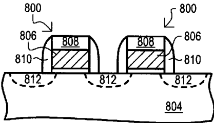
FIG. 8B BACKGROUND ART
