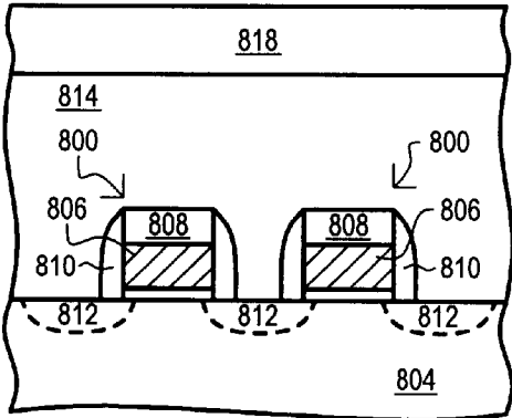
FIG. 8F BACKGROUND ART
