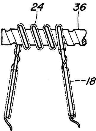
Fig. 3C (PRIOR ART)
