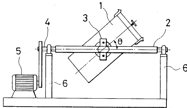
FIG. 1 PRIOR ART
