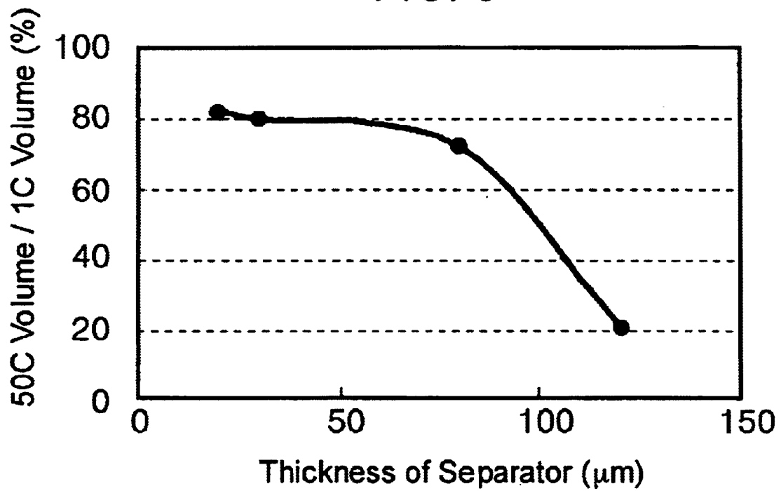
Separator thickness vs. High-rate Characteristics
