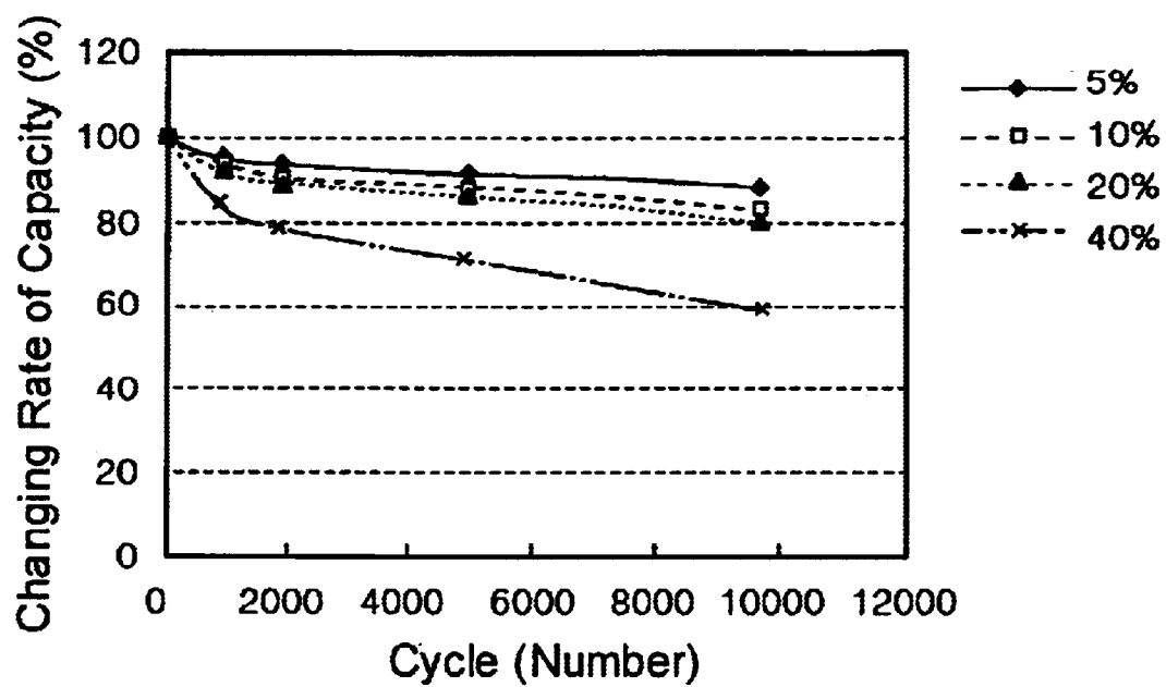
Electrolyte Concentration vs. Cycle Characteristic (Positive Electrode)
