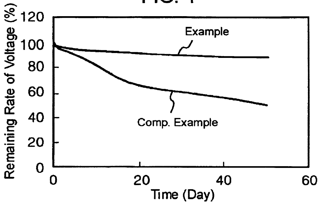
Self-discharge Characteristic
