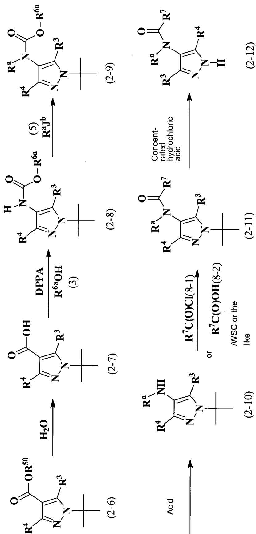
Reaction Scheme 2
