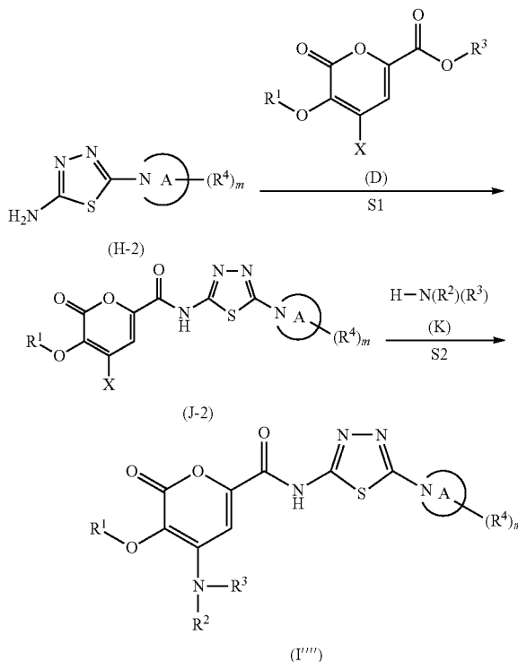
General Scheme 6.
