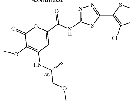
Compound 94 (R)-N-(5-(3-chlorothiophen-2-yl)-1,3,4-thiadiazol-2-yl)-3-methoxy-4-((1-methoxypropan-2-yl)amino)-2-oxo-2H-pyran-6-carboxamide
