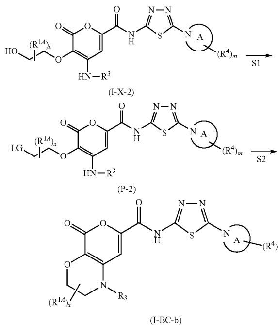
General Scheme 10.
