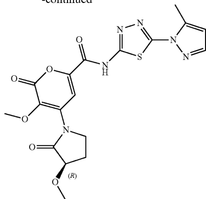
Compound 150 (R)-3-methoxy-4-(3-methoxy-2-oxopyrrolidin-1-yl)-N-(5-(5-methyl-1H-pyrazol-1-yl)-1,3,4-thiadiazol-2-yl)-2-oxo-2H-pyran-6-carboxamide
