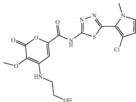
Compound 129 N-(5-(3-chloro-1-methyl-1H-pyrrol-2-yl)-1,3,4-thiadiazol-2-yl)-4-((2-hydroxyethyl)amino)-3-methoxy-2-oxo-2H-pyran-6-carboxamide
