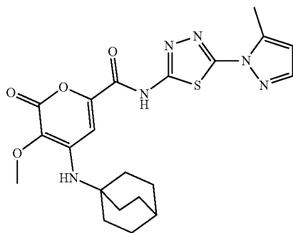
4-(bicyclo[2.2.2]octan-1-ylamino)-3-methoxy-N-(5-(5-methyl-1H-pyrazol-1-yl)-1,3,4-thiadiazol-2-yl)-2-oxo-2H-pyran-6-carboxamide
