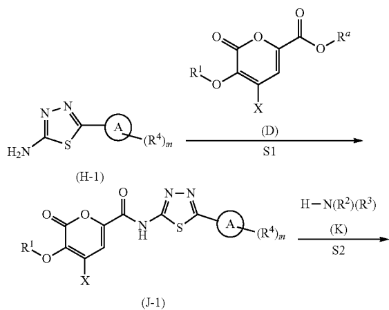
General Scheme 5.
