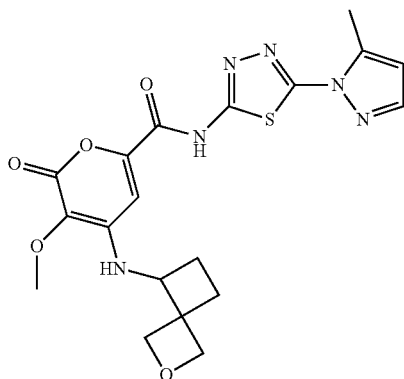
4-((2-oxaspiro[3.3]heptan-5-yl)amino)-3-methoxy-N-(5-(5-methyl-1H-pyrazol-1-yl)-1,3,4-thiadiazol-2-yl)-2-oxo-2H-pyran-6-carboxamide
