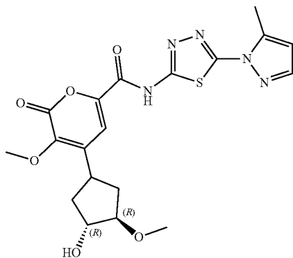
4-((3R,4R)-3-hydroxy-4-methoxypyrrolidin-1-yl)-3-methoxy-N-(5-(5-methyl-1H-pyrazol-1-yl)-1,3,4-thiadiazol-2-yl)-2-oxo-2H-pyran-6-carboxamide
