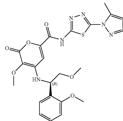
Compound 198* (R)-3-methoxy-4-((2-methoxy-1-(2-methoxyphenyl)ethyl)amino)-N-(5-(5-methyl-1H-pyrazol-1-yl)-1,3,4-thiadiazol-2-yl)-2-oxo-2H-pyran-6-carboxamide
