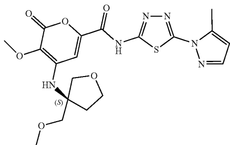
Compound 100* (S)-3-methoxy-4-((3-(methoxymethyl)tetrahydrofuran-3-yl)amino)-N-(5-(5-methyl-1H-pyrazol-1-yl)-1,3,4-thiadiazol-2-yl)-2-oxo-2H-pyran-6-carboxamide
