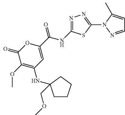
Compound 152 3-methoxy-4-((1-(methoxymethyl)cyclopentyl)amino)-N-(5-(5-methyl-1H-pyrazol-1-yl)-1,3,4-thiadiazol-2-yl)-2-oxo-2H-pyran-6-carboxamide
