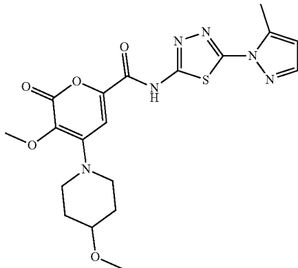
3-methoxy-4-(4-methoxypiperidin-1-yl)-N-(5-(5-methyl-1H-pyrazol-1-yl)-1,3,4-thiadiazol-2-yl)-2-oxo-2H-pyran-6-carboxamide
