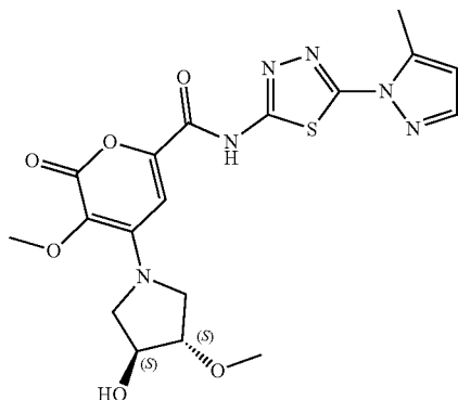
4-((3S,4S)-3-hydroxy-4-methoxypyrrolidin-1-yl)-3-methoxy-N-(5-(5-methyl-1H-pyrazol-1-yl)-1,3,4-thiadiazol-2-yl)-2-oxo-2H-pyran-6-carboxamide
