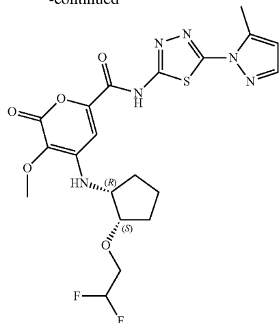
Compound 171 4-(((1R,2S)-2-(2,2-difluoroethoxy)cyclopentyl)amino)-3-methoxy-N-(5-(5-methyl-1H-pyrazol-1-yl)-1,3,4-thiadiazol-2-yl)-2-oxo-2H-pyran-6-carboxamide
