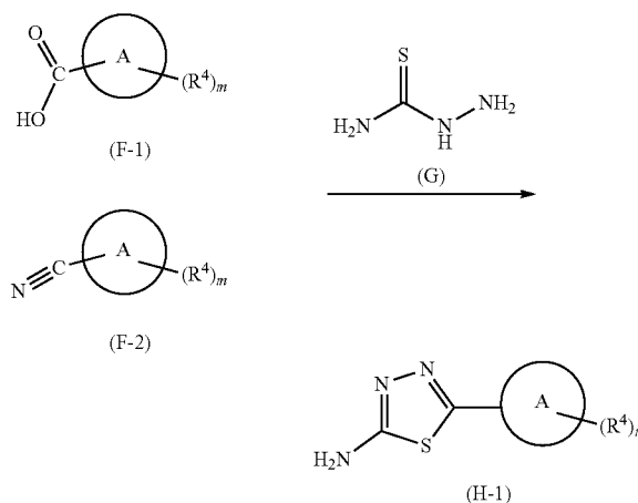
General Scheme 2.
