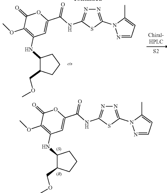
Compound 79* 3-methoxy-4-(((1S,2R)-2-(methoxymethyl)cyclopentyl)amino)-N-(5-(5-methyl-1H-pyrazol-1-yl)-1,3,4-thiadiazol-2-yl)-2-oxo-2H-pyran-6-carboxamide
