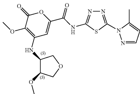
Compound 160 3-methoxy-4-(((3S,4S)-4-methoxytetrahydrofuran-3-yl)amino)-N-(5-(5-methyl-1H-pyrazol-1-yl)-1,3,4-thiadiazol-2-yl)-2-oxo-2H-pyran-6-carboxamide
