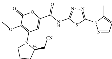
Compound 174 (R)-4-(2-(cyanomethyl)pyrrolidin-1-yl)-3-methoxy-N-(5-(5-methyl-1H-pyrazol-1-yl)-1,3,4-thiadiazol-2-yl)-2-oxo-2H-pyran-6-carboxamide
