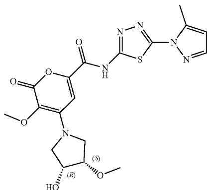
4-((3R,4S)-3-hydroxy-4-methoxypyrrolidin-1-yl)-3-methoxy-N-(5-(5-methyl-1H-pyrazol-1-yl)-1,3,4-thiadiazol-2-yl)-2-oxo-2H-pyran-6-carboxamide
