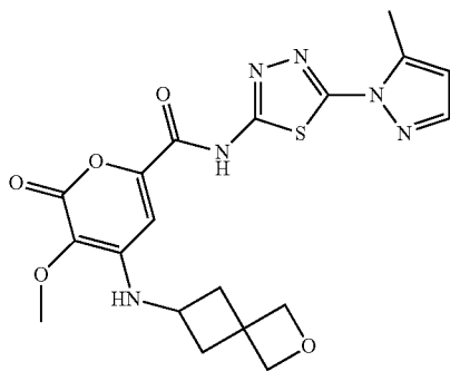
4-((2-oxaspiro[3.3]heptan-6-yl)amino)-3-methoxy-N-(5-(5-methyl-1H-pyrazol-1-yl)-1,3,4-thiadiazol-2-yl)-2-oxo-2H-pyran-6-carboxamide
