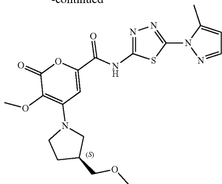
Compound 87 (S)-3-methoxy-4-(3-(methoxymethyl)pyrrolidin-1-yl)-N-(5-(5-methyl-1H-pyrazol-1-yl)-1,3,4-thiadiazol-2-yl)-2-oxo-2H-pyran-6-carboxamide
