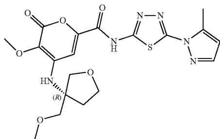
Compound 101* (R)-3-methoxy-4-((3-(methoxymethyl)tetrahydrofuran-3-yl)amino)-N-(5-(5-methyl-1H-pyrazol-1-yl)-1,3,4-thiadiazol-2-yl)-2-oxo-2H-pyran-6-carboxamide
