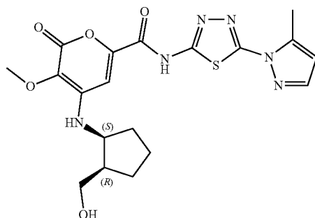
4-(((1S,2R)-2-(hydroxymethyl)cyclopentyl)amino)-3-methoxy-N-(5-(5-methyl-1H-pyrazol-1-yl)-1,3,4-thiadiazol-2-yl)-2-oxo-2H-pyran-6-carboxamide
