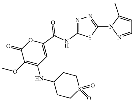
4-((1,1-dioxido-2,3,4,5-tetrahydrothiopyran-4-yl)amino)-3-methoxy-N-(5-(5-methyl-1H-pyrazol-1-yl)-1,3,4-thiadiazol-2-yl)-2-oxo-2H-pyran-6-carboxamide
