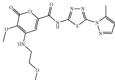
Compound 75 3-methoxy-4-((2-methoxyethyl)amino)-N-(5-(5-methyl-1H-pyrazol-1-yl)-1,3,4-thiadiazol-2-yl)-2-oxo-2H-pyran-6-carboxamide
