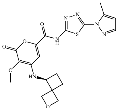
(S)-4-((2-oxaspiro[3.3]heptan-5-yl)amino)-3-methoxy-N-(5-(5-methyl-1H-pyrazol-1-yl)-1,3,4-thiadiazol-2-yl)-2-oxo-2H-pyran-6-carboxamide
