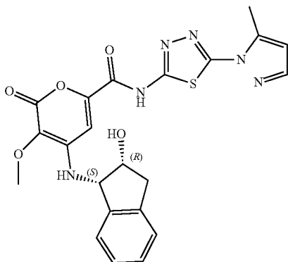
4-(((1S,2R)-2-hydroxy-2,3-dihydro-1H-inden-1-yl)amino)-3-methoxy-N-(5-(5-methyl-1H-pyrazol-1-yl)-1,3,4-thiadiazol-2-yl)-2-oxo-2H-pyran-6-carboxamide
