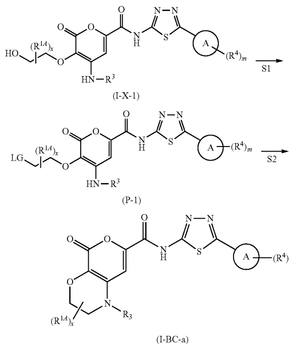
General Scheme 9.
