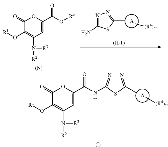
General Scheme 7.
