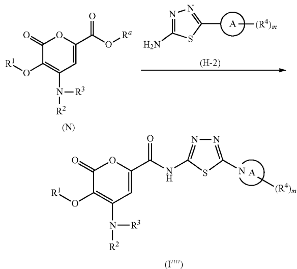
General Scheme 8.
