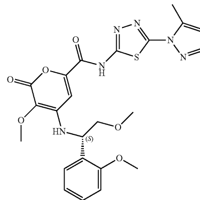
Compound 199* (S)-3-methoxy-4-((2-methoxy-1-(2-methoxyphenyl)ethyl)amino)-N-(5-(5-methyl-1H-pyrazol-1-yl)-1,3,4-thiadiazol-2-yl)-2-oxo-2H-pyran-6-carboxamide
