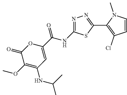
Compound 131 N-(5-(3-chloro-1-methyl-1H-pyrrol-2-yl)-1,3,4-thiadiazol-2-yl)-4-(isopropylamino)-3-methoxy-2-oxo-2H-pyran-6-carboxamide
