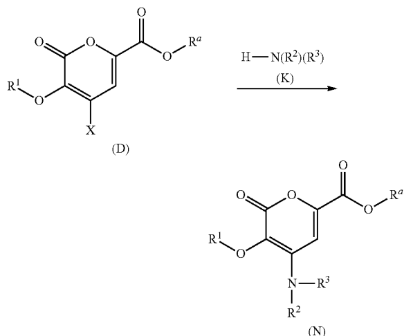
General Scheme 4.
