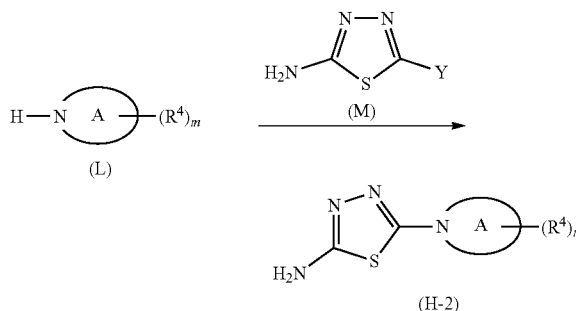
General Scheme 3.
