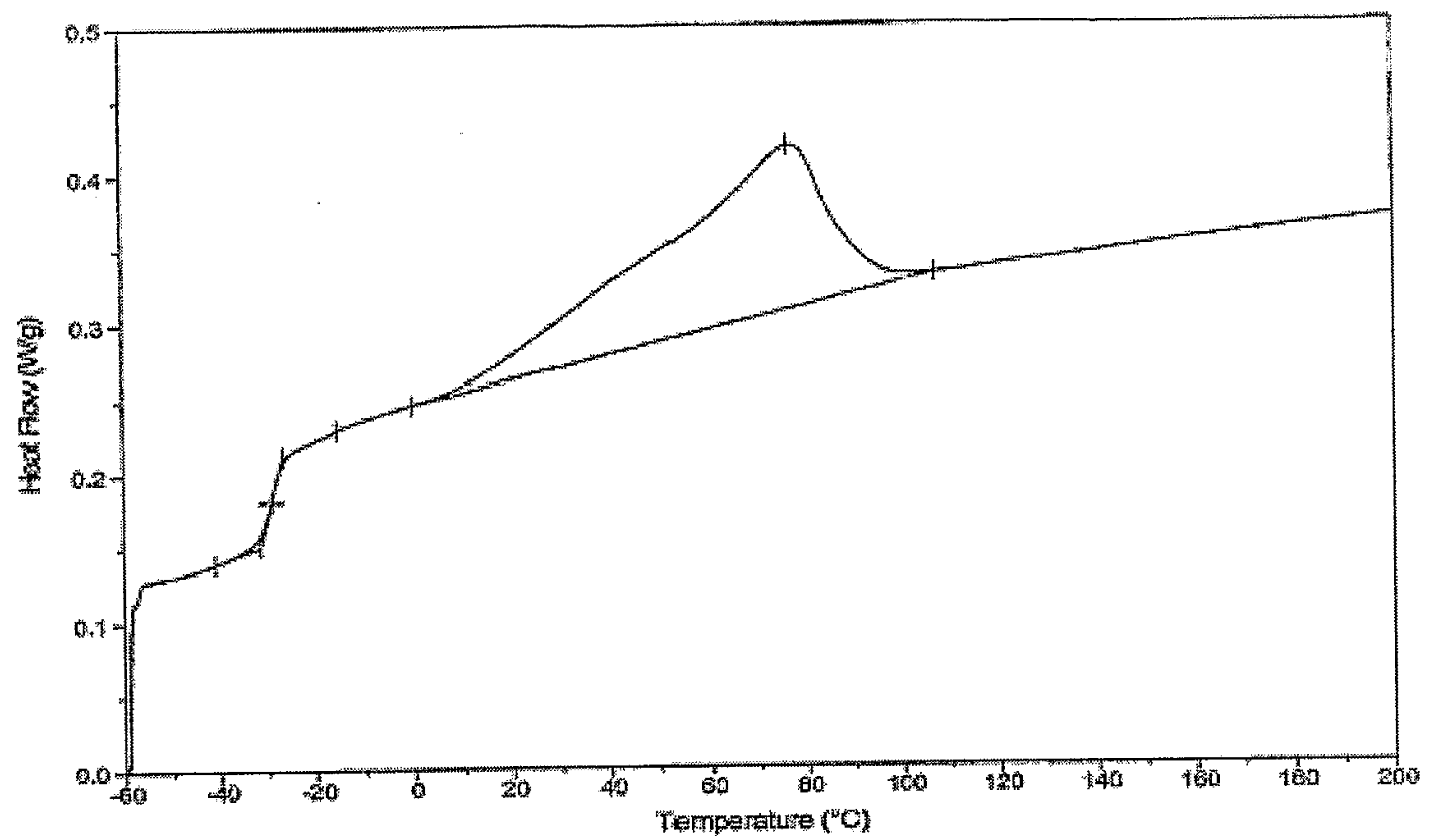
Figure 2 DSC Plot of Sample 11
