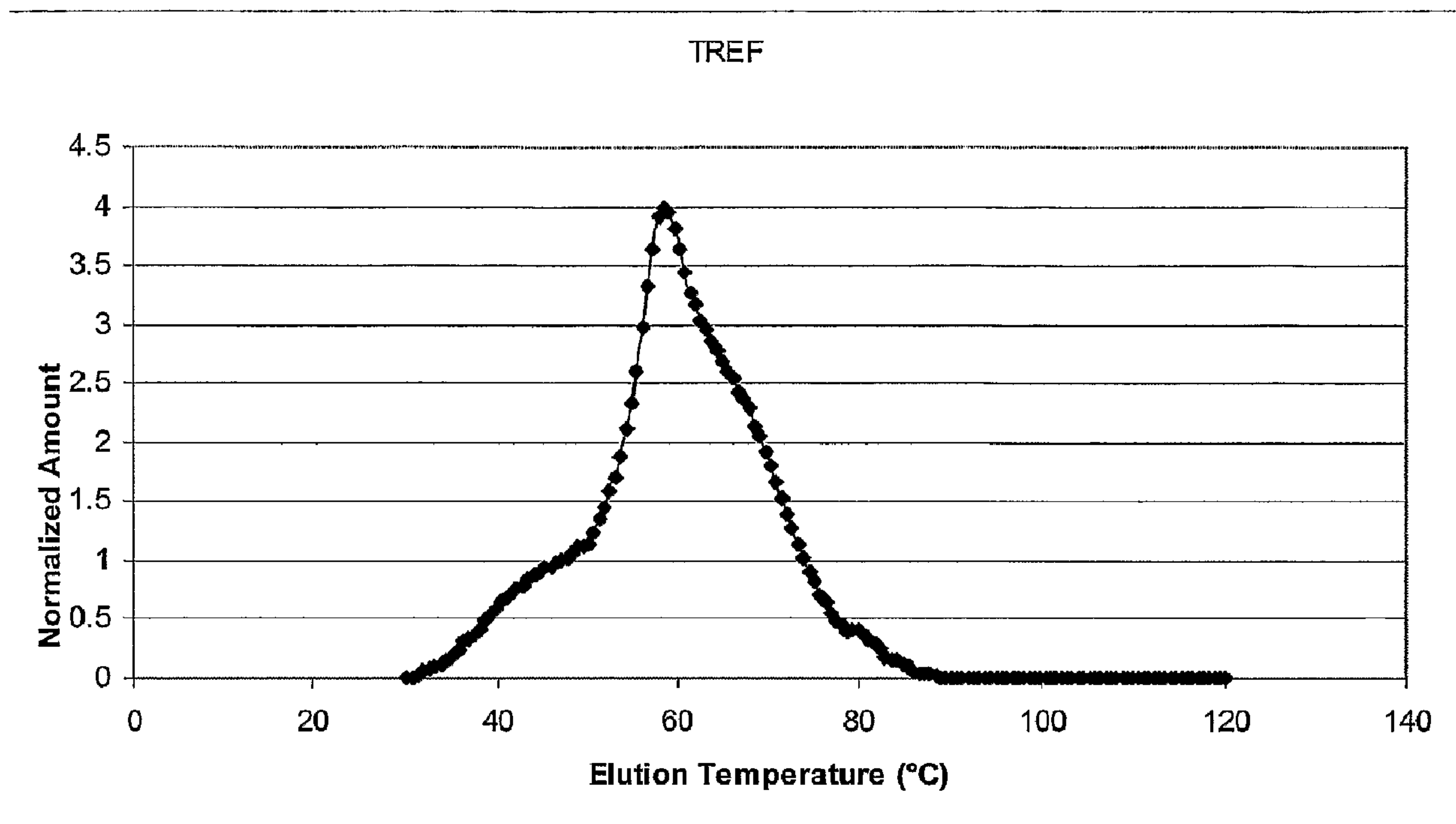
TREF Curve for a P/E* copolymer
