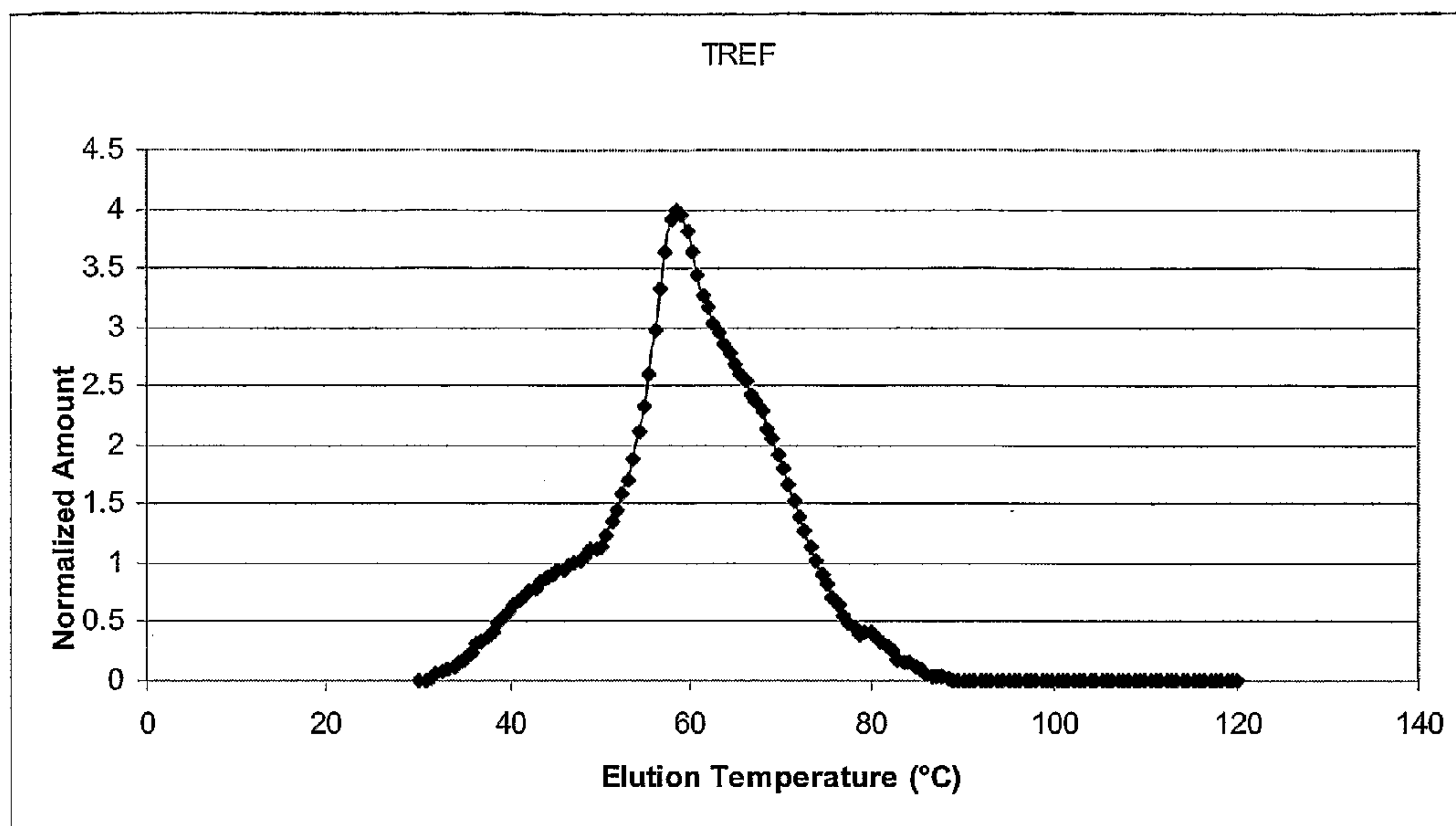
TREF Curve for a P/E* copolymer
