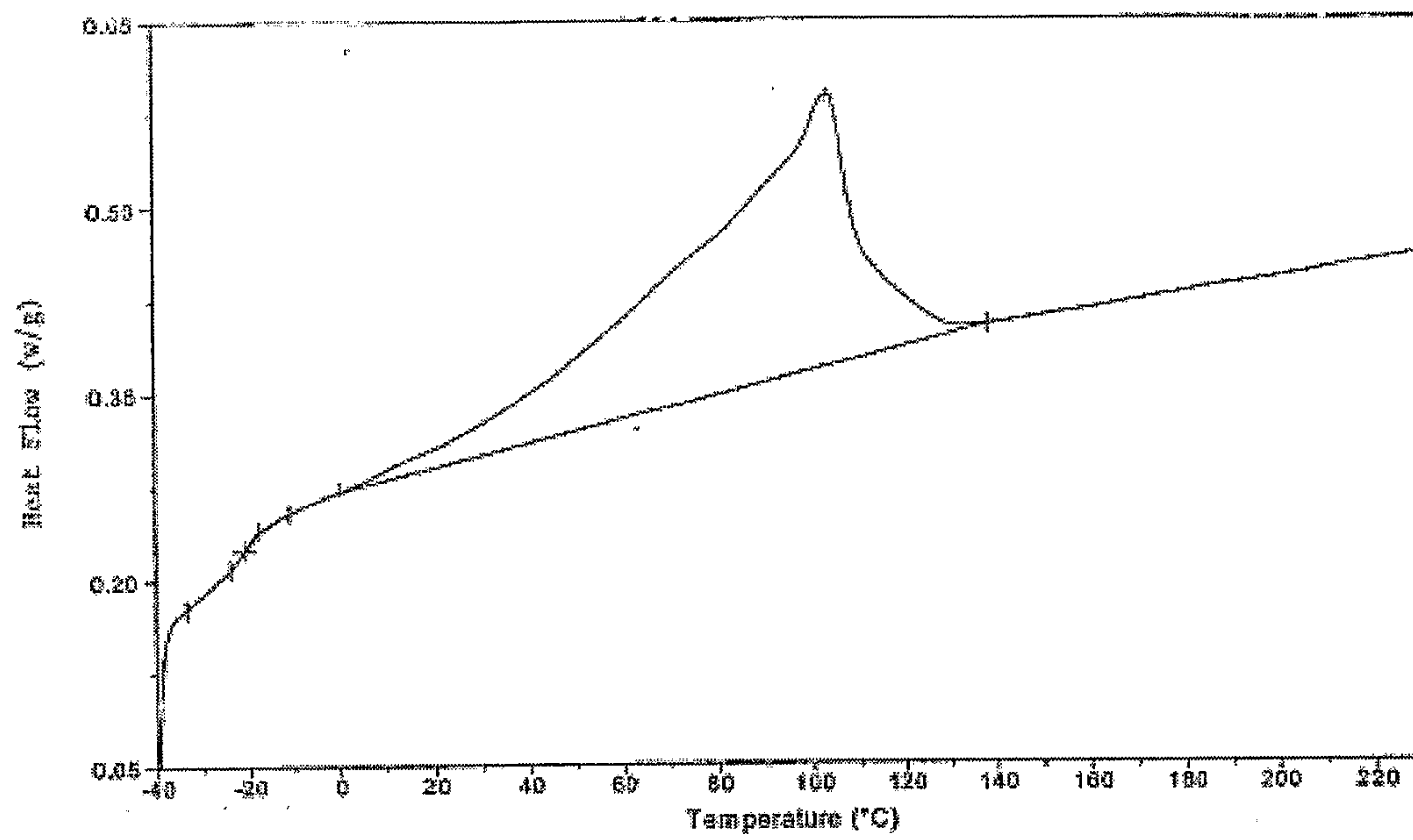
Figure 5 DSC Plot of Sample 31
