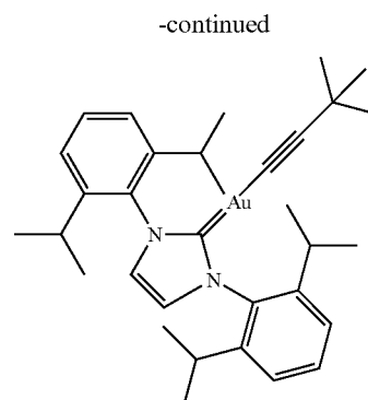
Au(IPr)(t-BuE)
