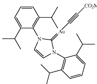
Au(IPr)(MCE)
