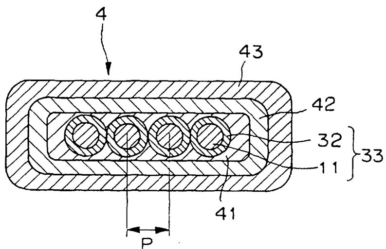
FIG. 21 (PRIOR ART)
