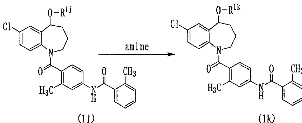
Reaction Scheme-10
