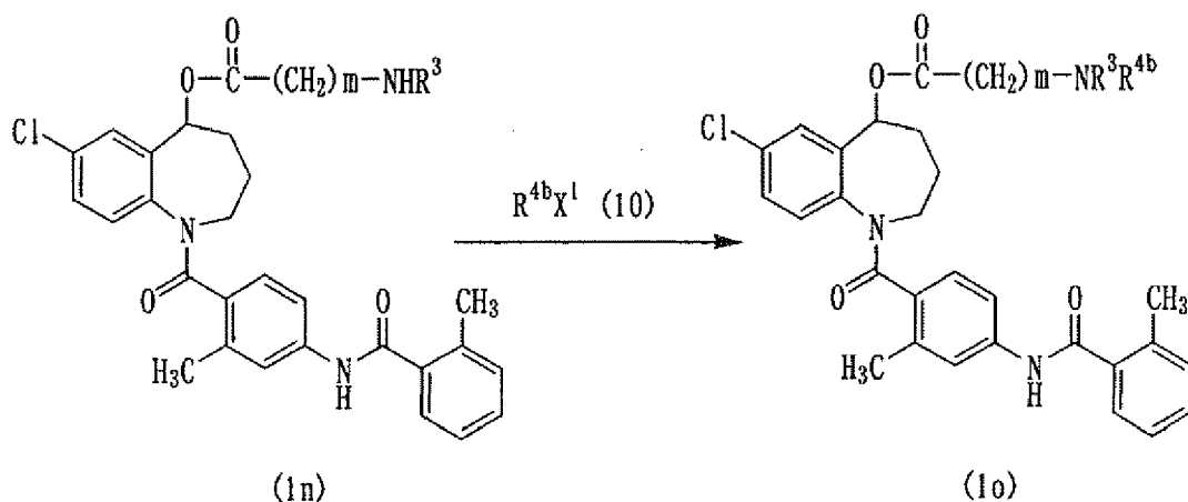
Reaction Scheme-12
