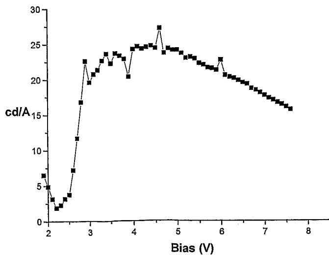
External efficiency
