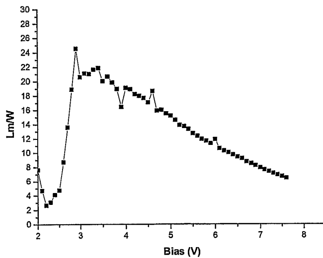
Power efficiency
