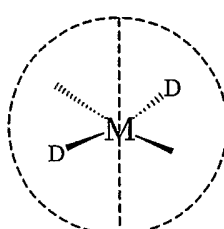
trans
