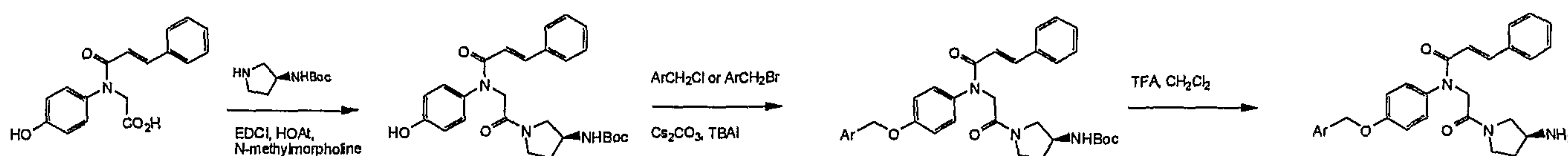
Scheme 3
