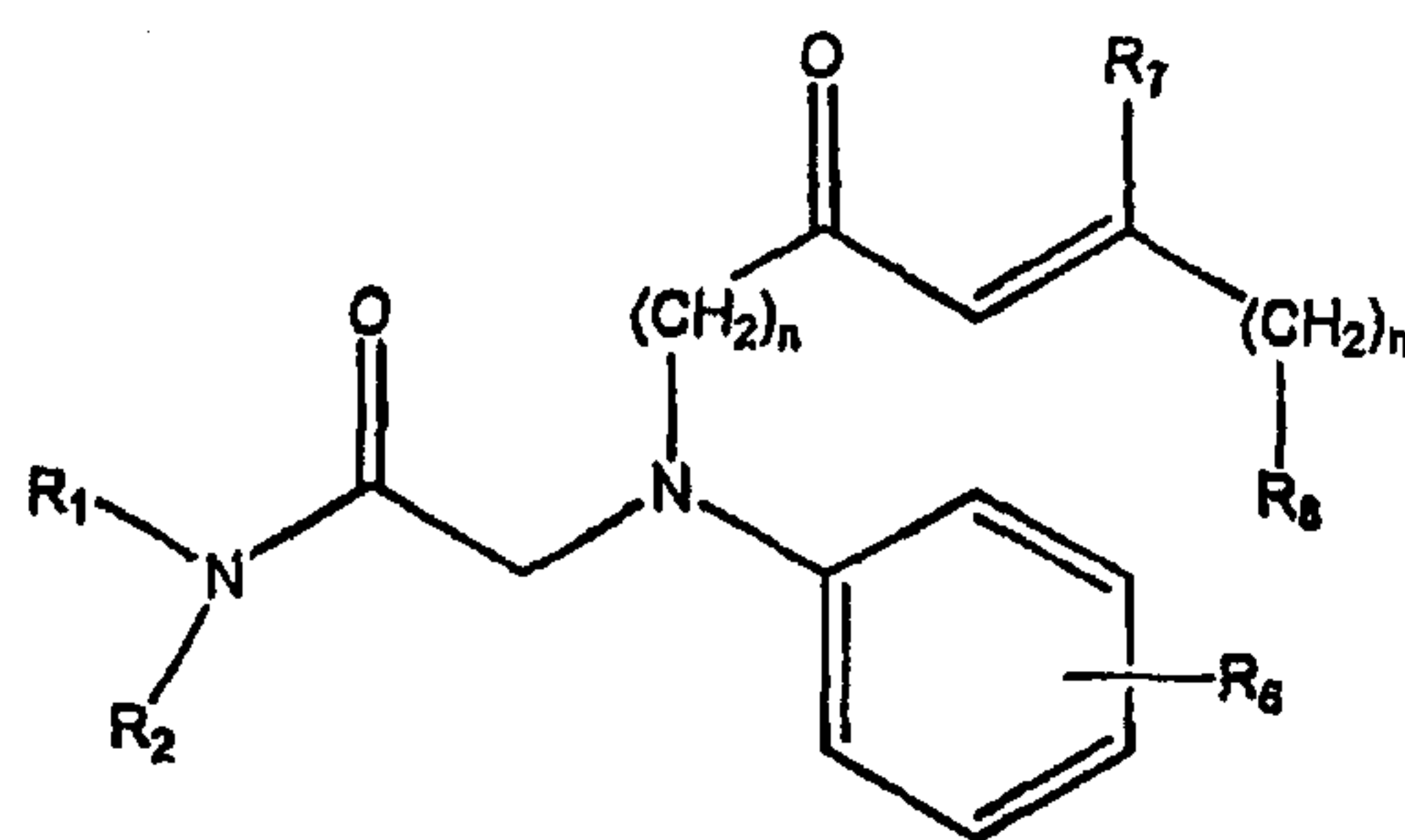
Formula VII
