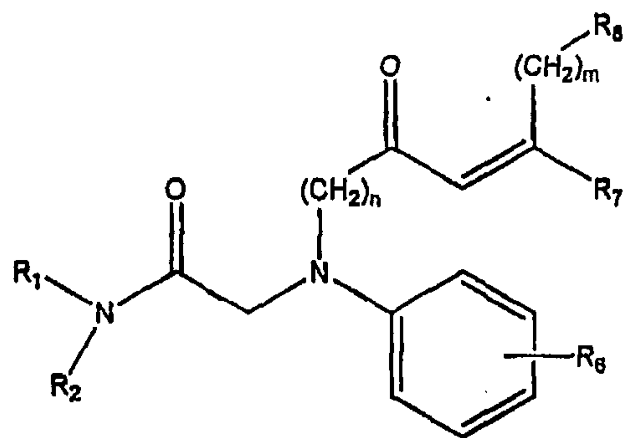
Formula VI
