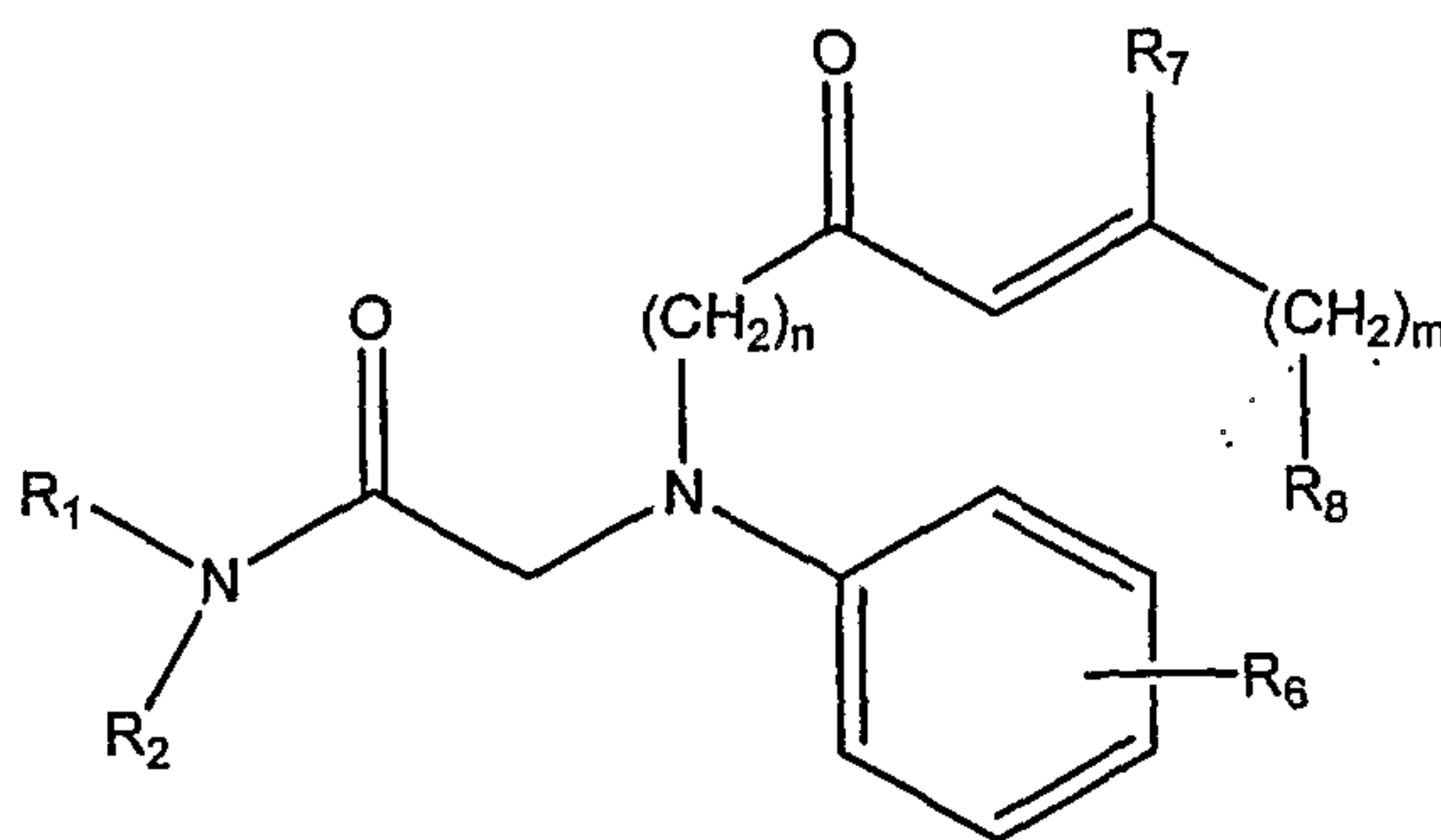
Formula VII
