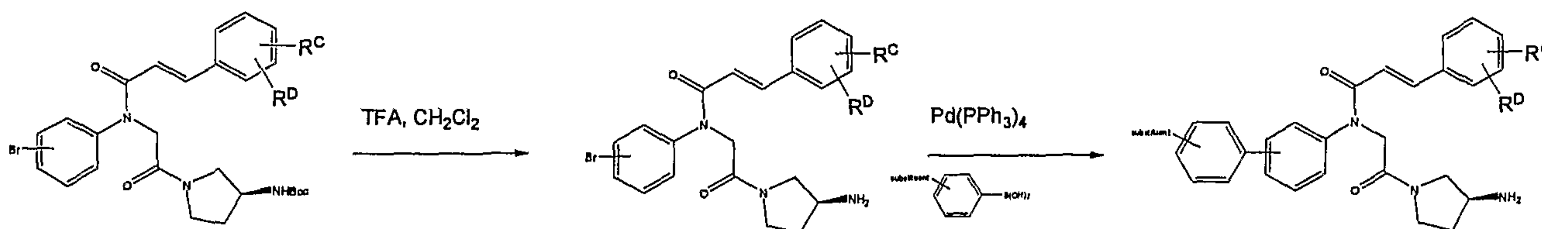
Scheme 2
