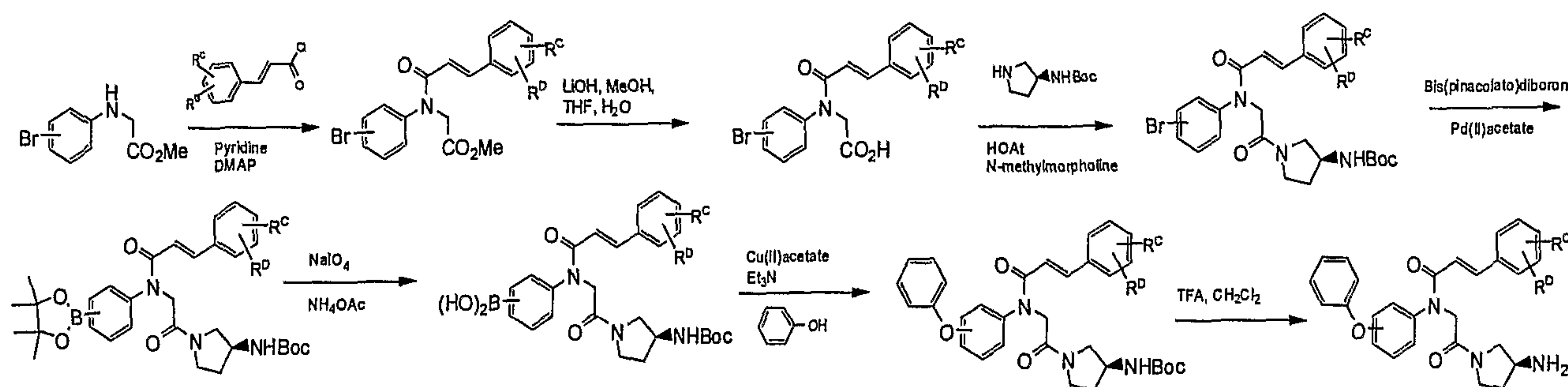
Scheme 1
