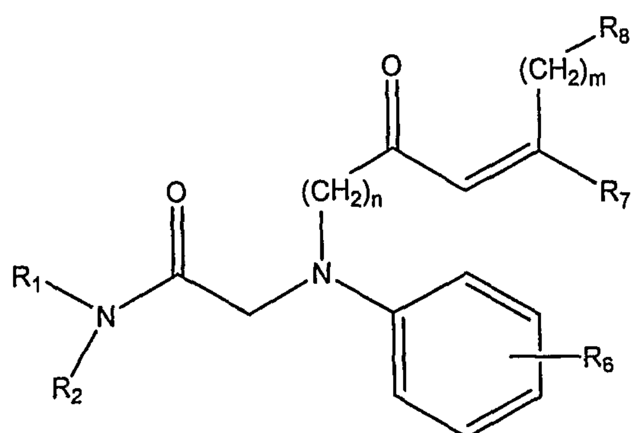
Formula VI
