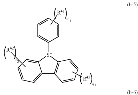
[Chemical Formula 37]
