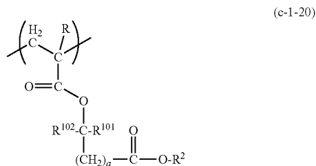
[Chemical Formula 49]
