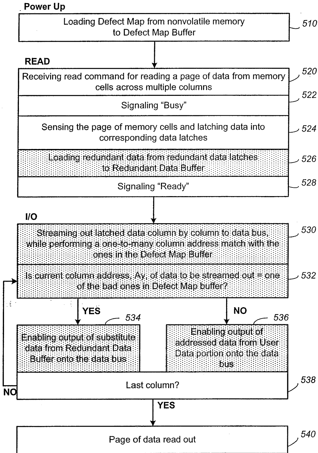
READ WITH REDUNDANT DATA BUFFER
