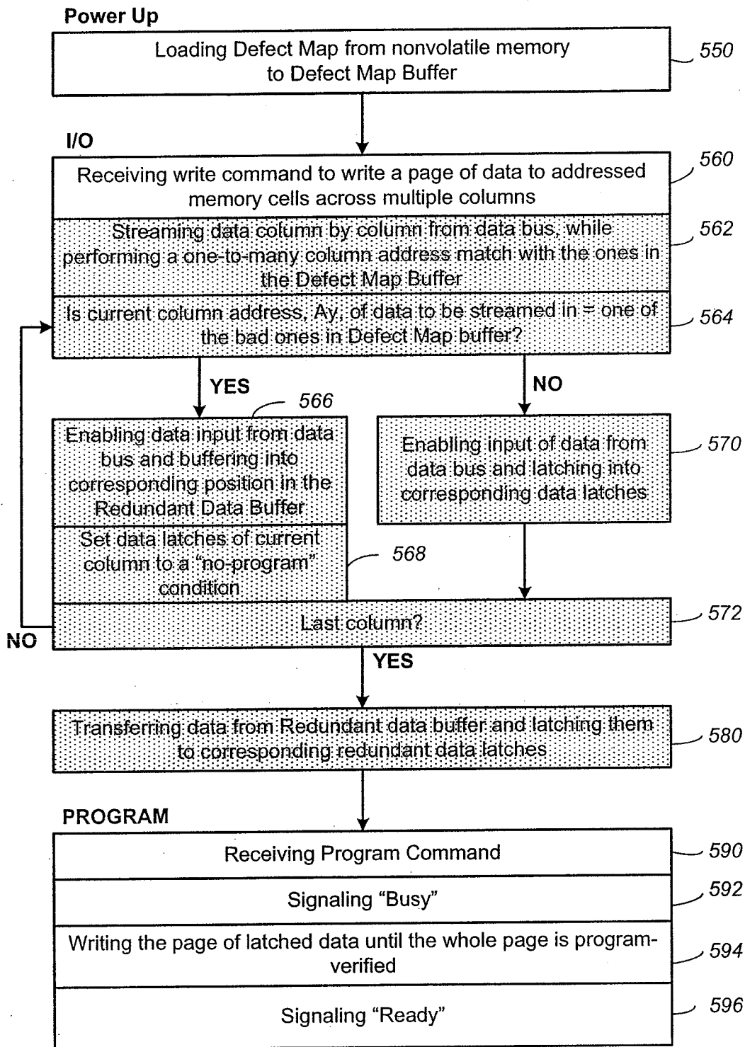
PROGRAM WITH REDUNDANT DATA BUFFER
