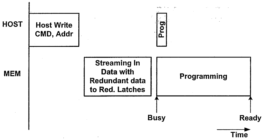
PROGRAM TIMING (Prior Art)
