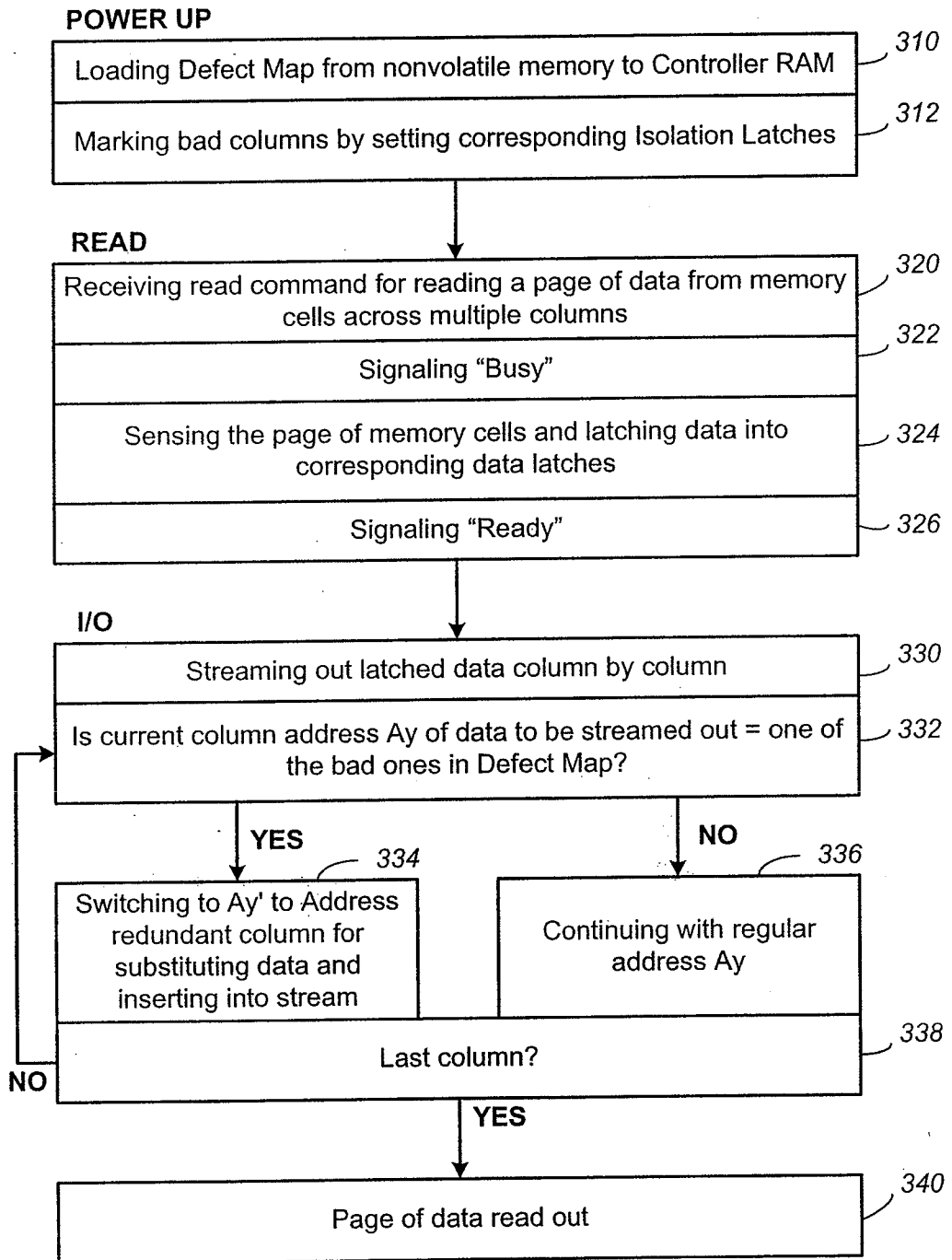
READ OPERATION (Prior Art)
