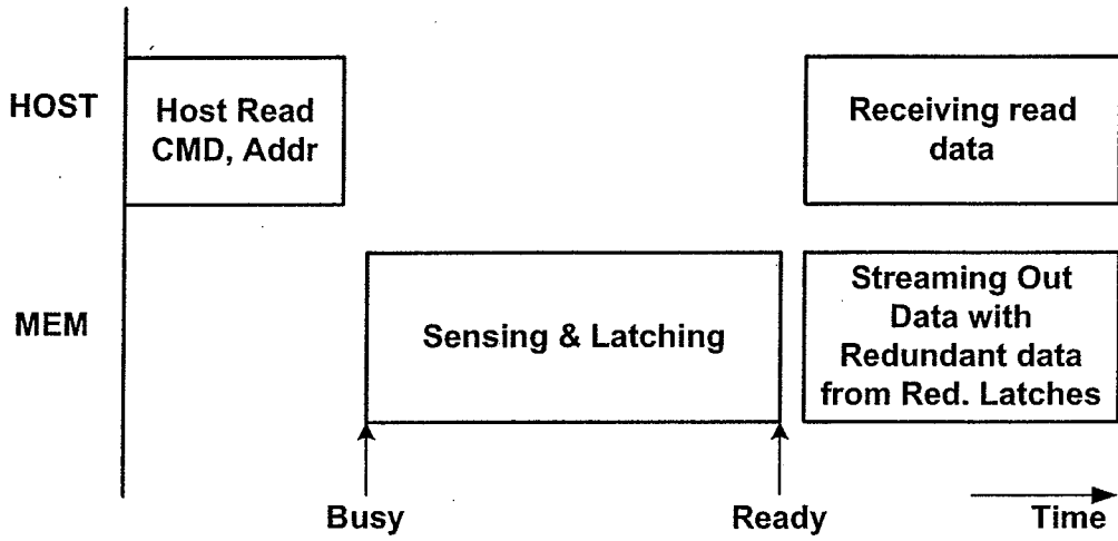
READ TIMING (Prior Art)
