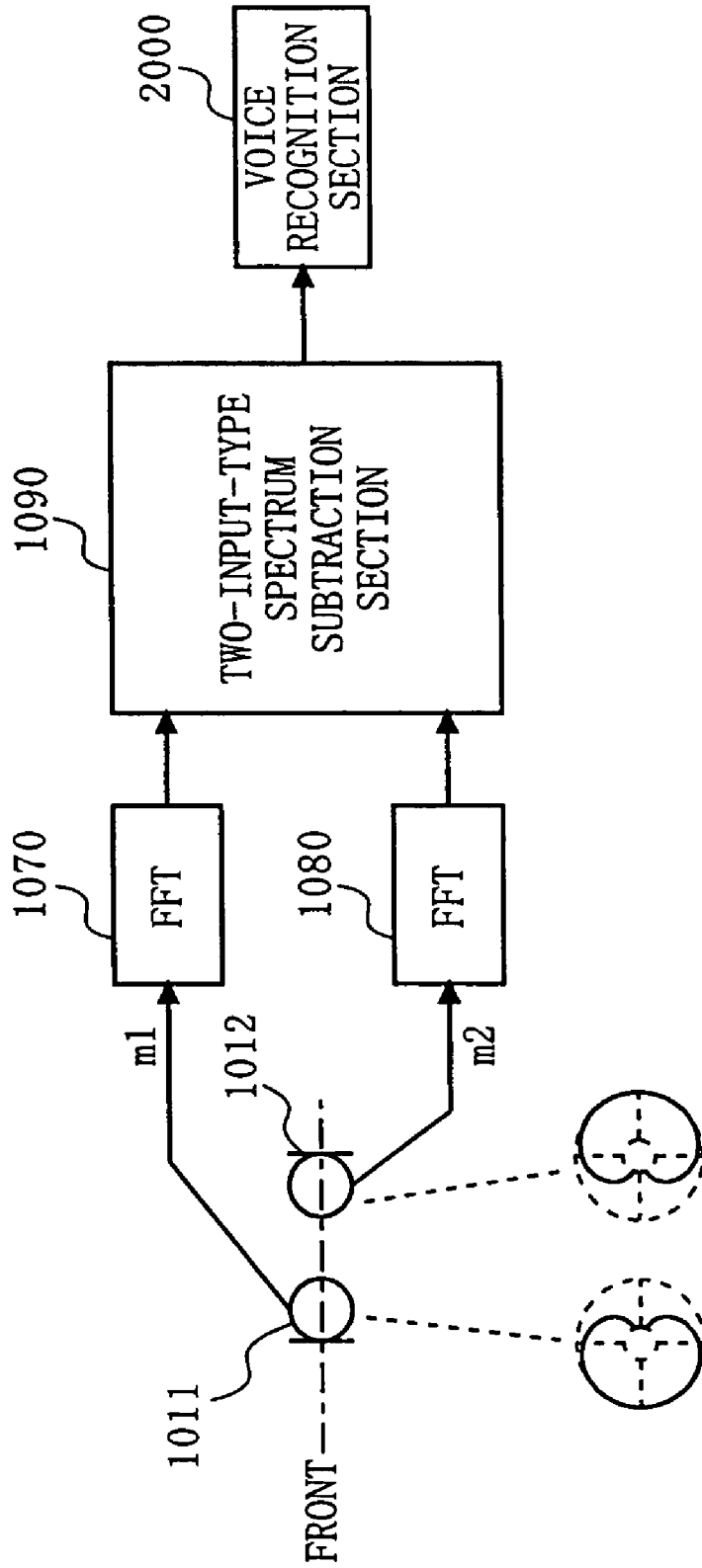
FIG. 26 PRIOR ART
