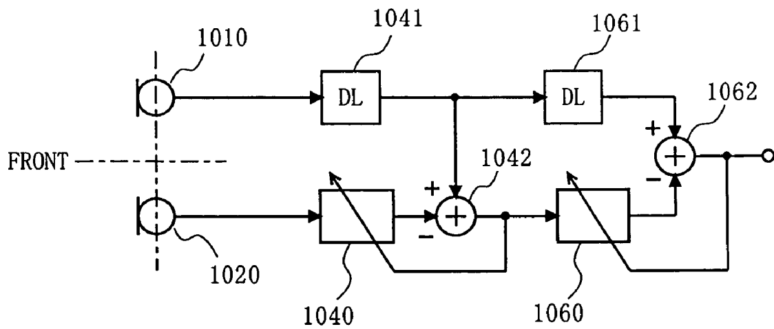
FIG. 25 PRIOR ART
