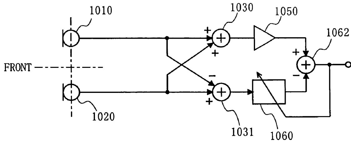
FIG. 24 PRIOR ART
