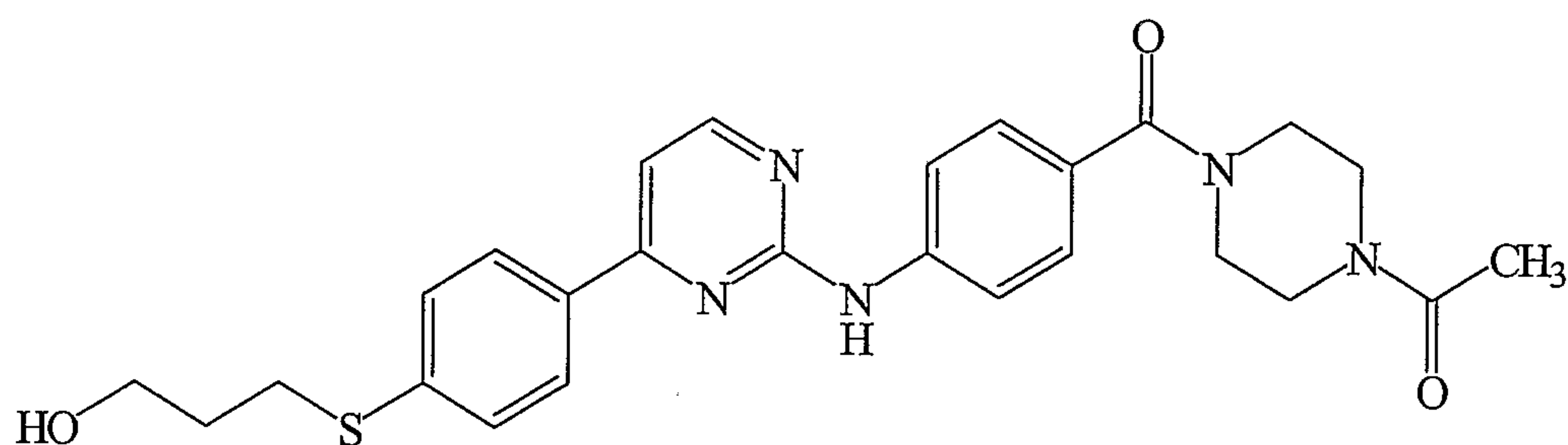
1-[4-(4-{4-[4-(3-Hydroxy-propylsulfanyl)-phenyl]-pyrimidin-2-ylamino}-benzoyl)- piperazin-1-yl]-ethanone ;
