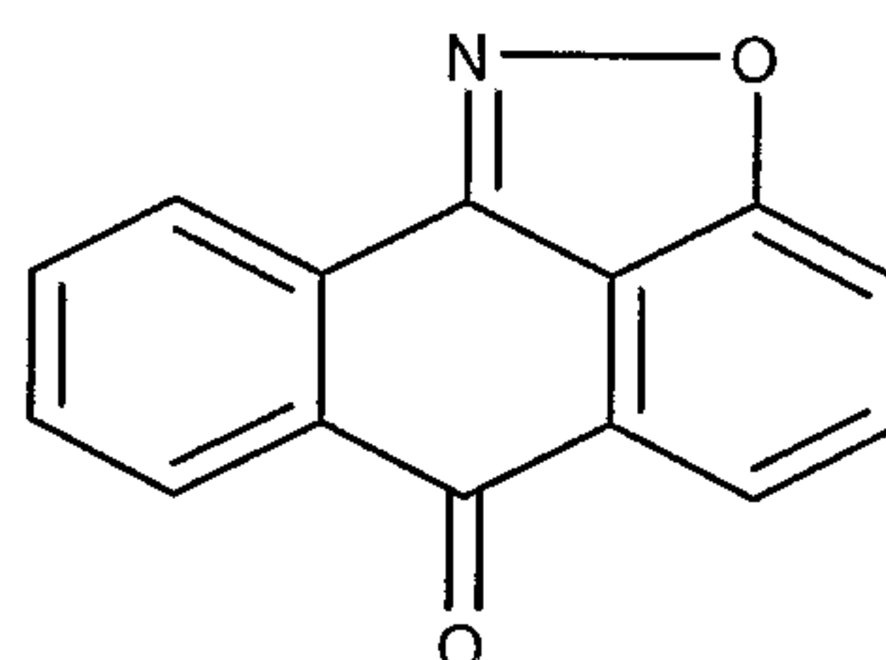
2-Oxa-1-aza-aceanthrylen-6-one;
