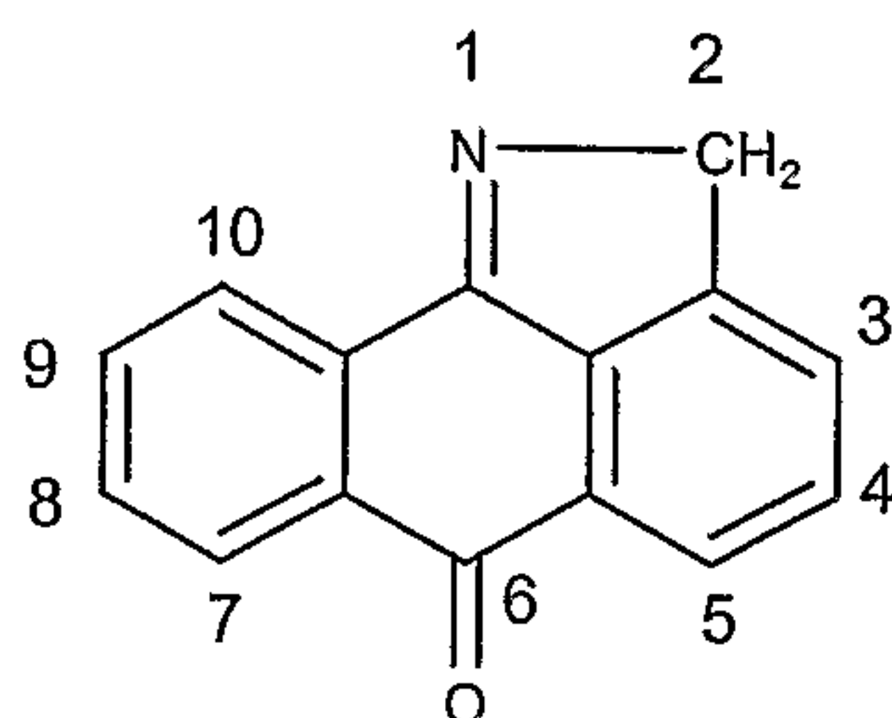
2H-Dibenzo[cd,g]indol-6-one (IIIA)
