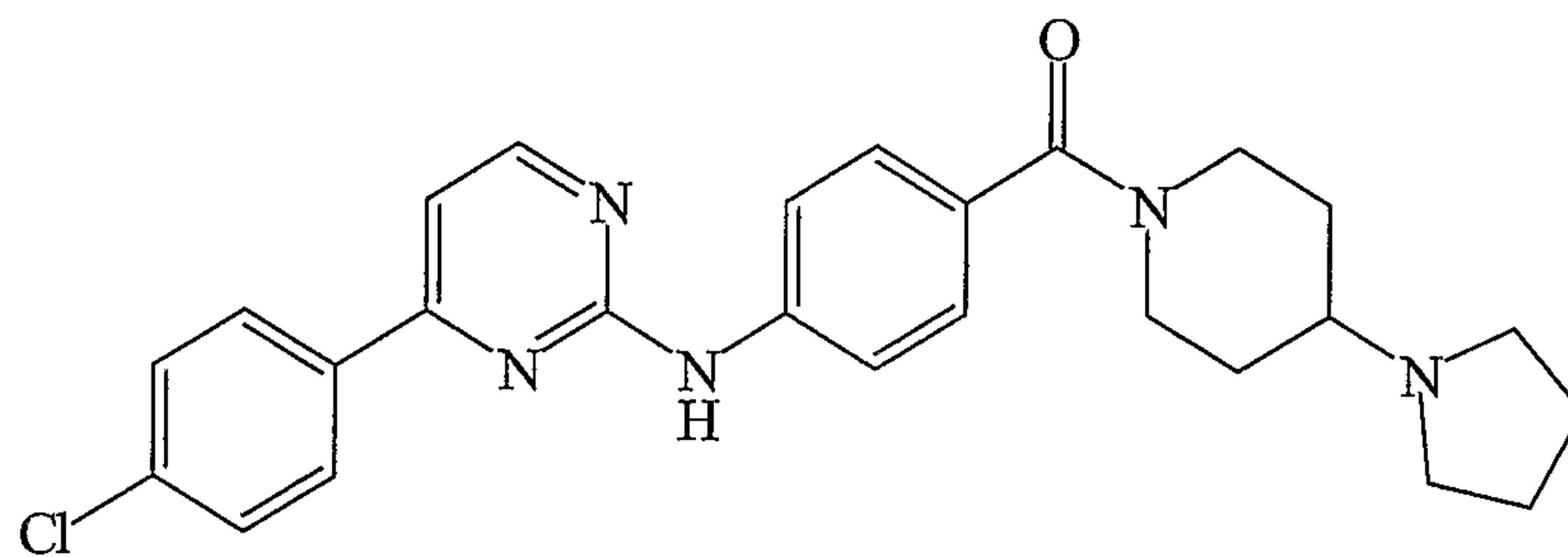
{4-[4-(4-Chloro-phenyl)-pyrimidin-2-ylamino]-phenyl}-(4-pyrrolidin-1-yl- piperidin-1-yl)-methanone ;
