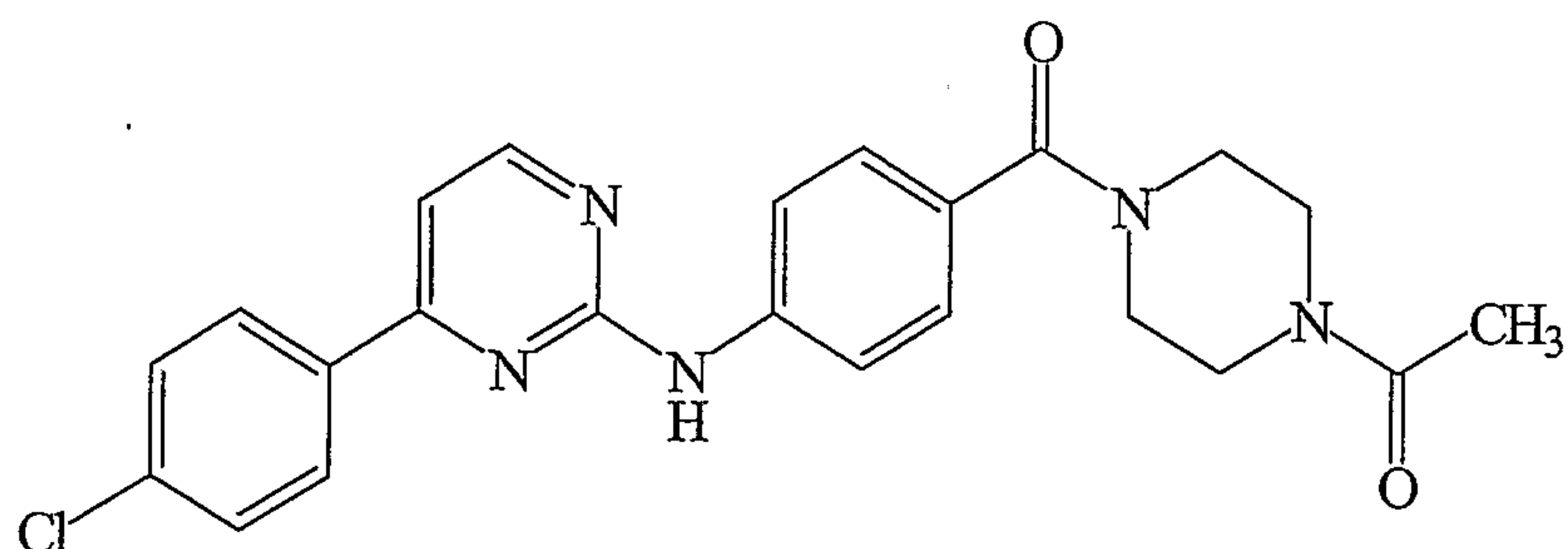
1-(4-{4-[4-(4-Chloro-phenyl)-pyrimidin-2-ylamino]-benzoyl}- piperazin-1-yl)-ethanone ;
