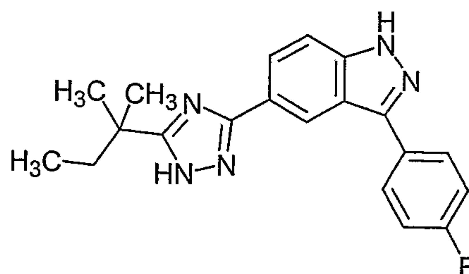
5- [5-(1,1\text{-Dimethyl-propyl})\text{-}1H\text{-}[1,2,4]\text{triazol-}3\text{-yl}] -3-(4-fluoro-phenyl)- 1H -indazole ;
