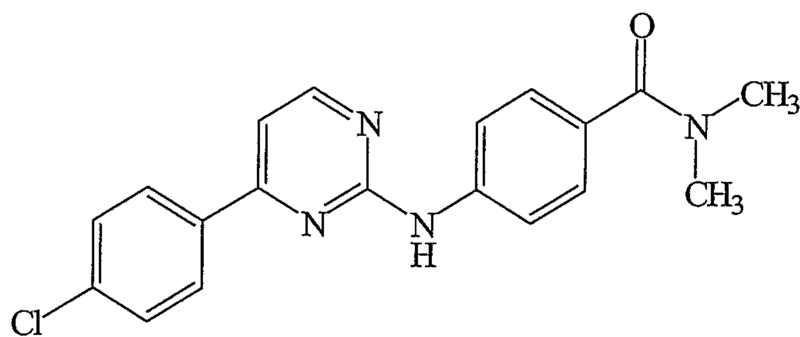
4-[4-(4-Chloro-phenyl)-pyrimidin-2-ylamino]- N,N -dimethyl- benzamide
