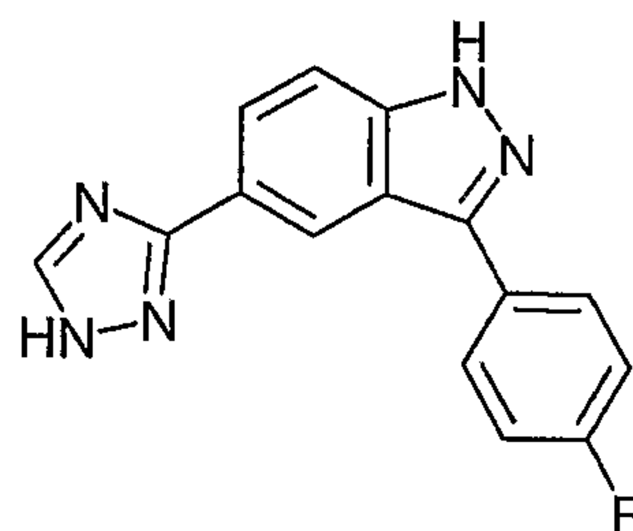
3-(4-Fluoro-phenyl)-5-(1 H - [1,2,4]triazol-3-yl)-1 H -indazole;
