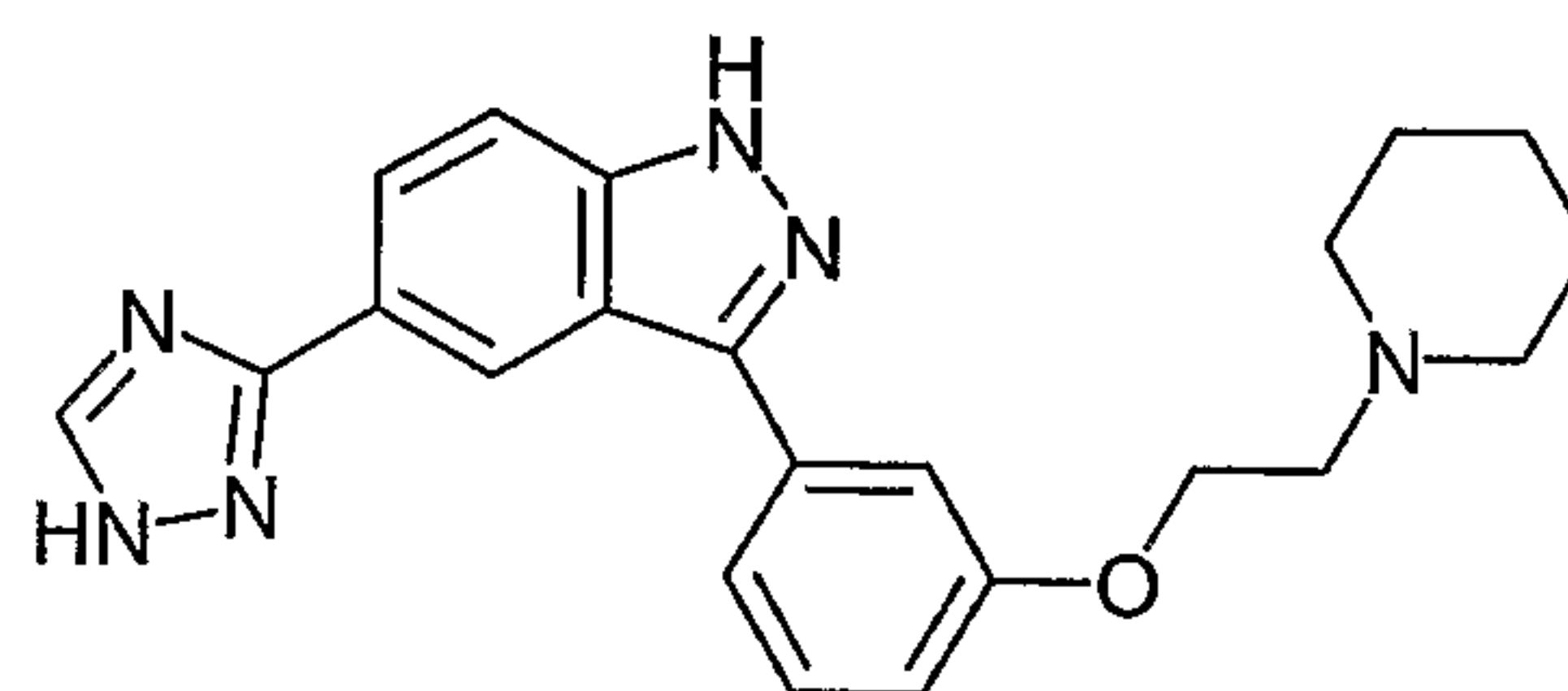
3-[3-(2-Piperidin-1-yl-ethoxy)-phenyl]-5-(1 H - [1,2,4]triazol-3-yl)-1 H -indazole ;
