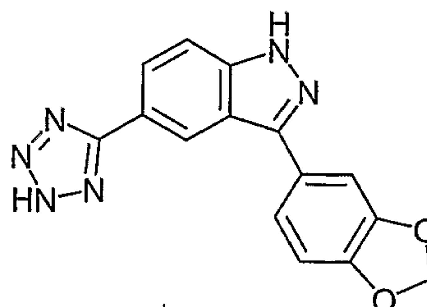
3-Benzo[1,3]dioxol-5-yl-5-(2 H -tetrazol- 5-yl)-1 H -indazole ;
