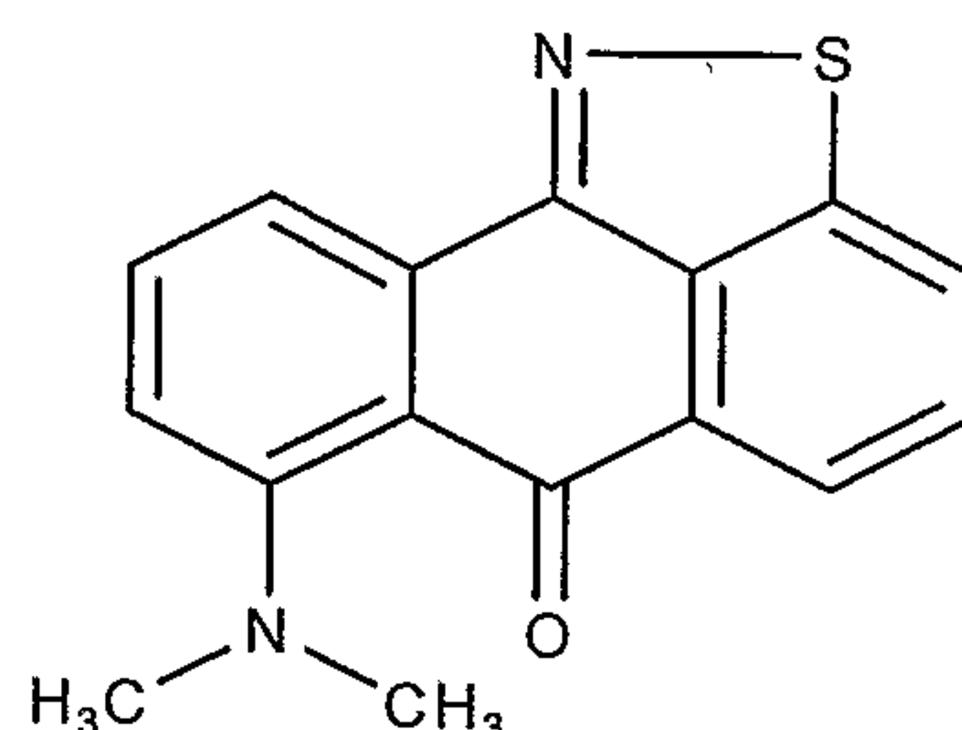
7-Dimethylamino-anthra[9,1- cd]isothiazol-6-one ;
