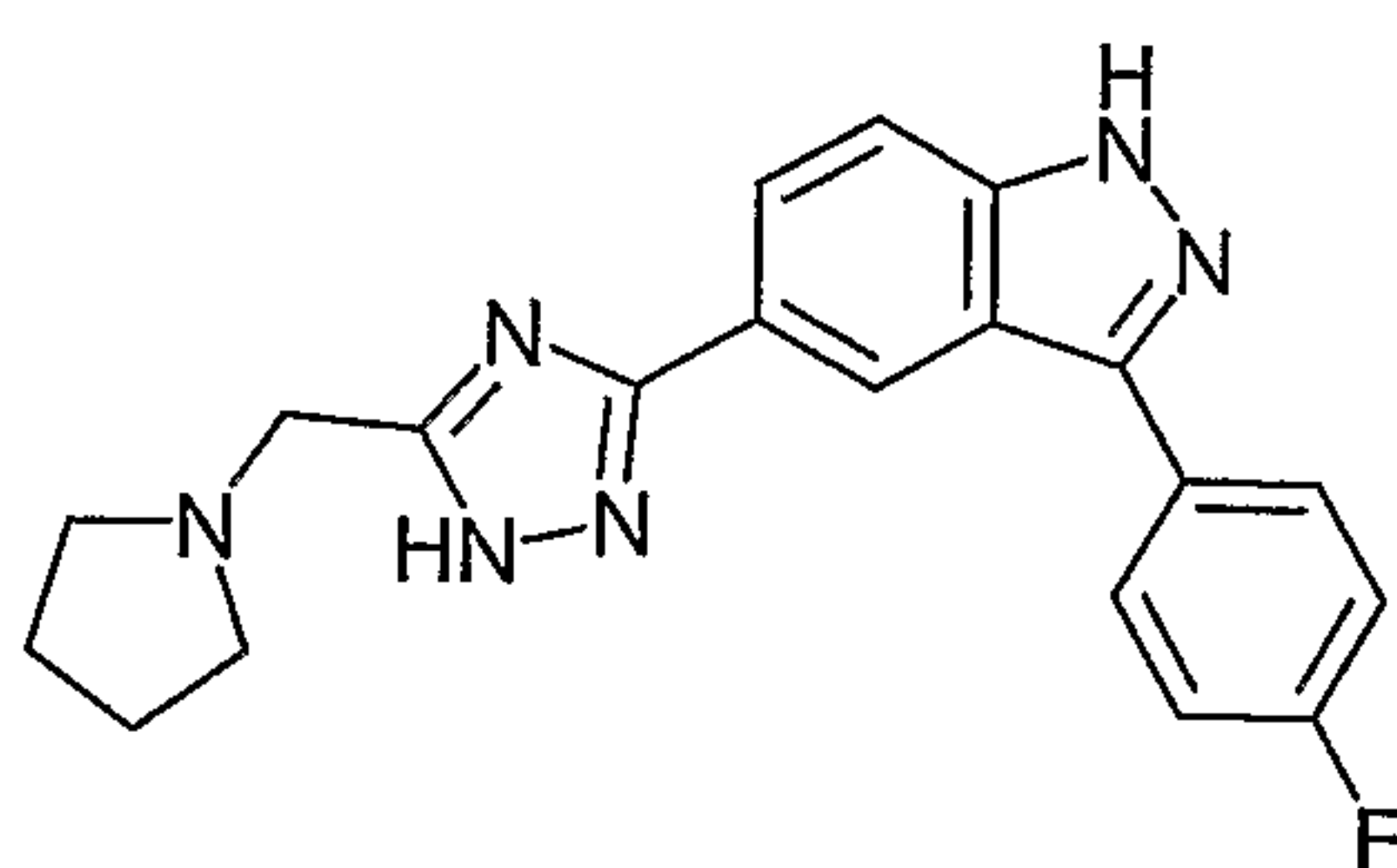
3-(4-Fluoro-phenyl)-5-(5-pyrrolidin-1-ylmethyl- 1H\text{-}[1,2,4]\text{triazol-}3\text{-yl}) - 1H -indazole ;
