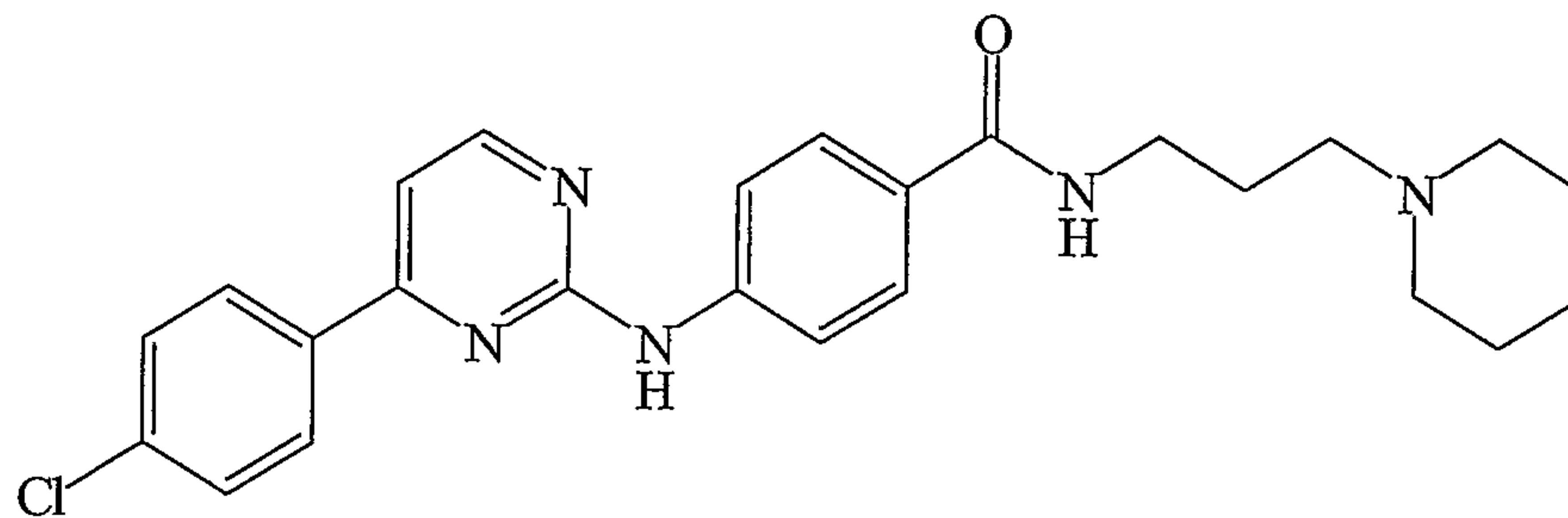
4-[4-(4-Chloro-phenyl)-pyrimidin-2-ylamino]- N -(3-piperidin-1-yl-propyl)- benzamide
