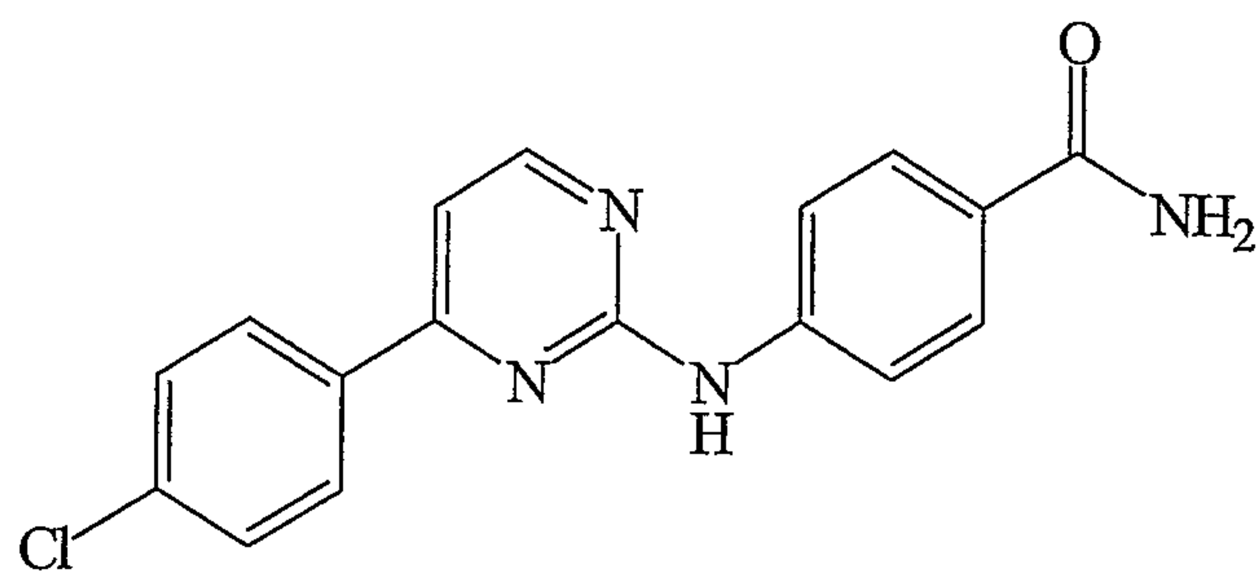
4-[4-(4-Chloro-phenyl)-pyrimidin-2-ylamino]- benzamide
