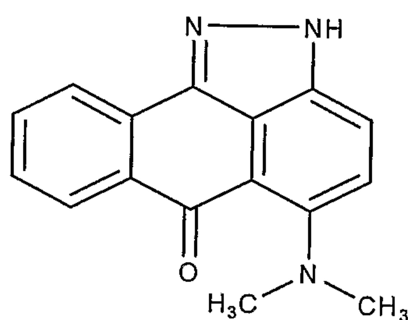
5-Dimethylamino-2 H - dibenzo[ cd,g ]indazol-6-one;
