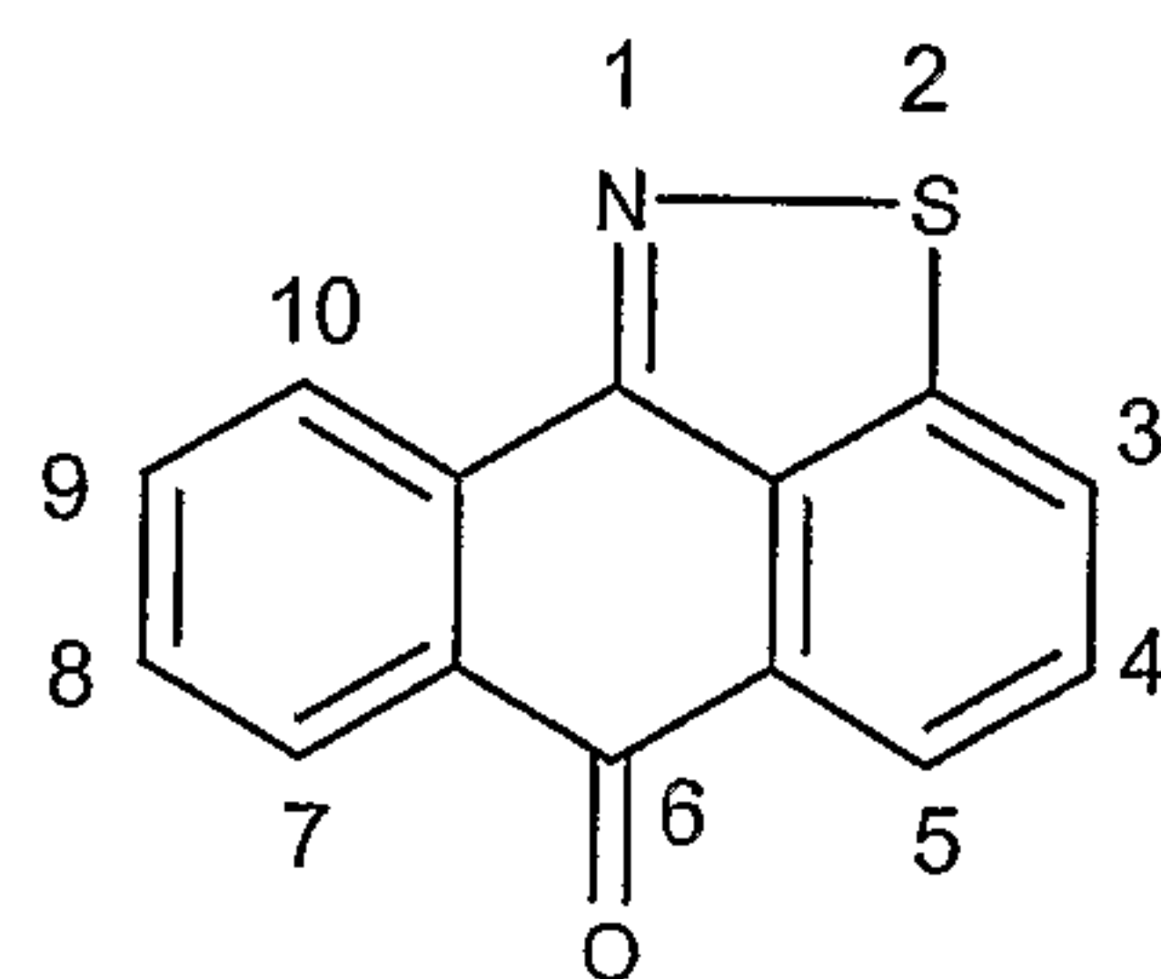
Anthra[9,1-cd]isothiazol-6-one (IIIE)
