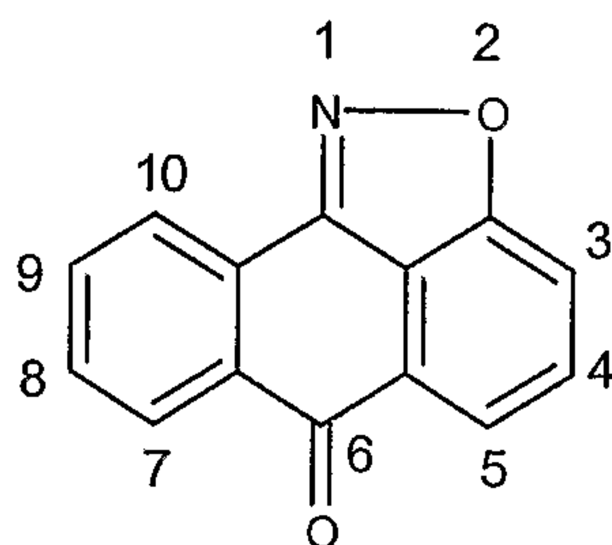
2-Oxa-1-aza-acanthrylen-6-one (IIC)
