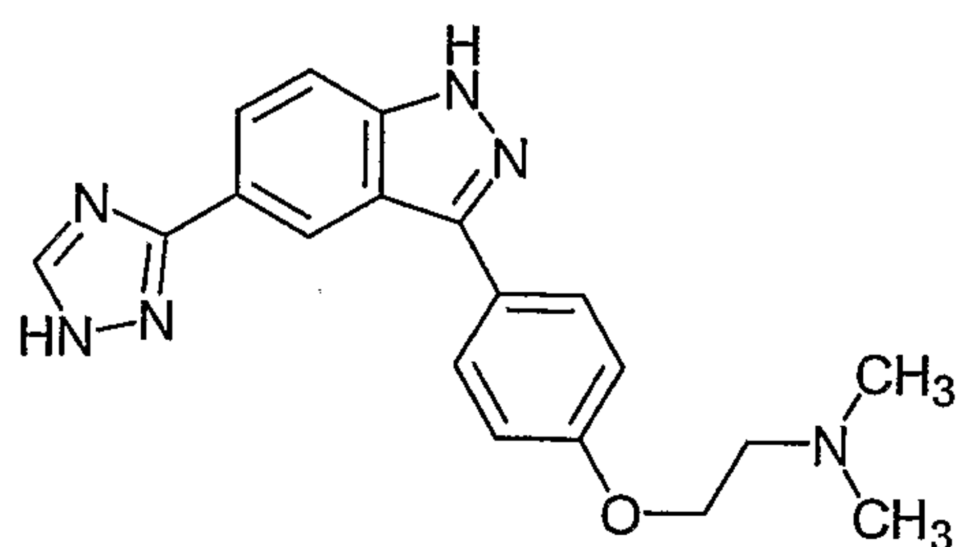
Dimethyl-(2-{4-[5-(1 H -[1,2,4]triazol-3-yl)-1 H -indazol-3-yl]-phenoxy}-ethyl)-amine ;
