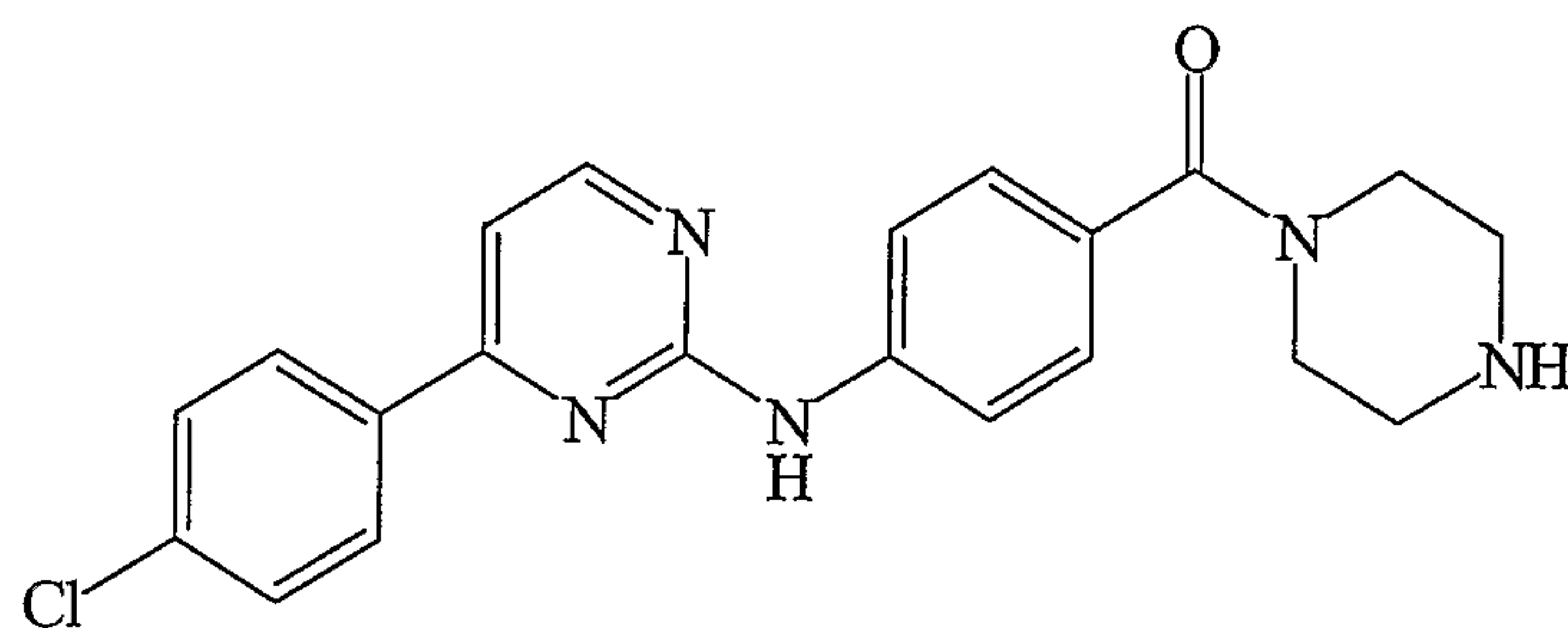
{4-[4-(4-Chloro-phenyl)-pyrimidin-2-ylamino]-phenyl}- piperazin-1-yl-methanone
