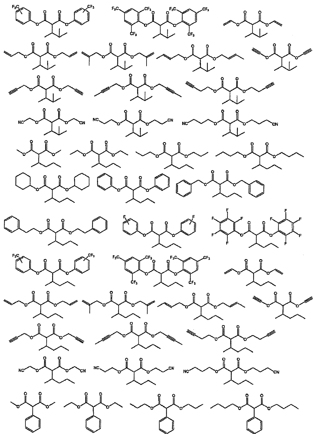
[Chemical formula 13]
