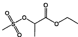
Compound 11: Ethyl 2-(methanesulfonyloxy)propionate
