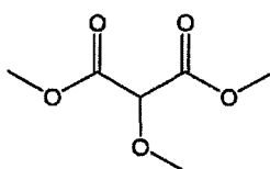
Compound 9: Dimethyl methoxymalonate
