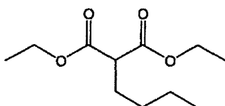
Compound 2: Diethyl butylmalonate
