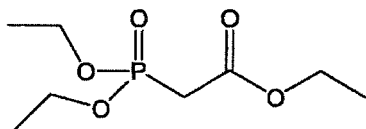
Compound 28: Triethyl phosphonoacetate
