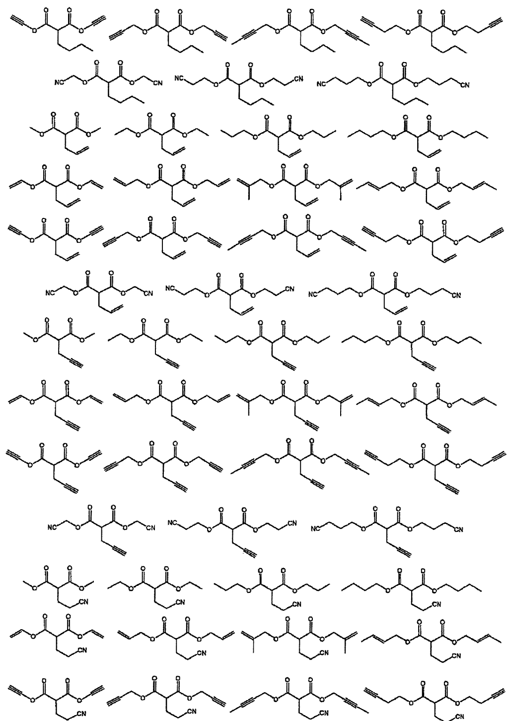
[Chemical formula 21]
