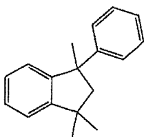
Compound 29: 1-Phenyl-1,3,3-trimethylindan
