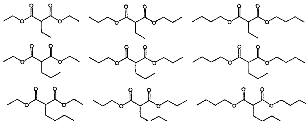
[Chemical formula 26]
