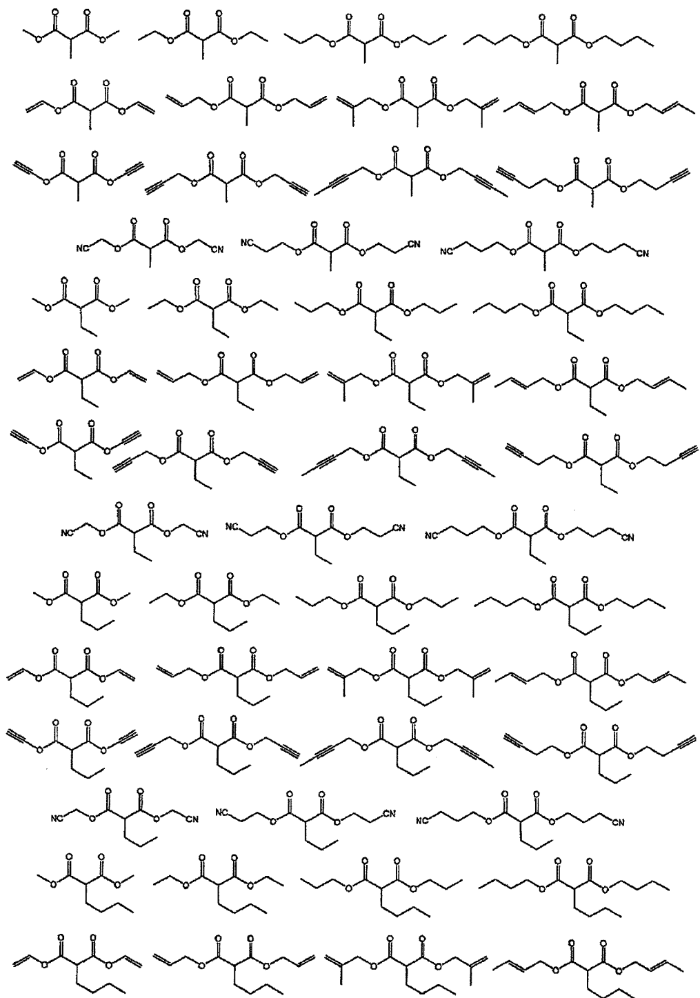
[Chemical formula 15]
