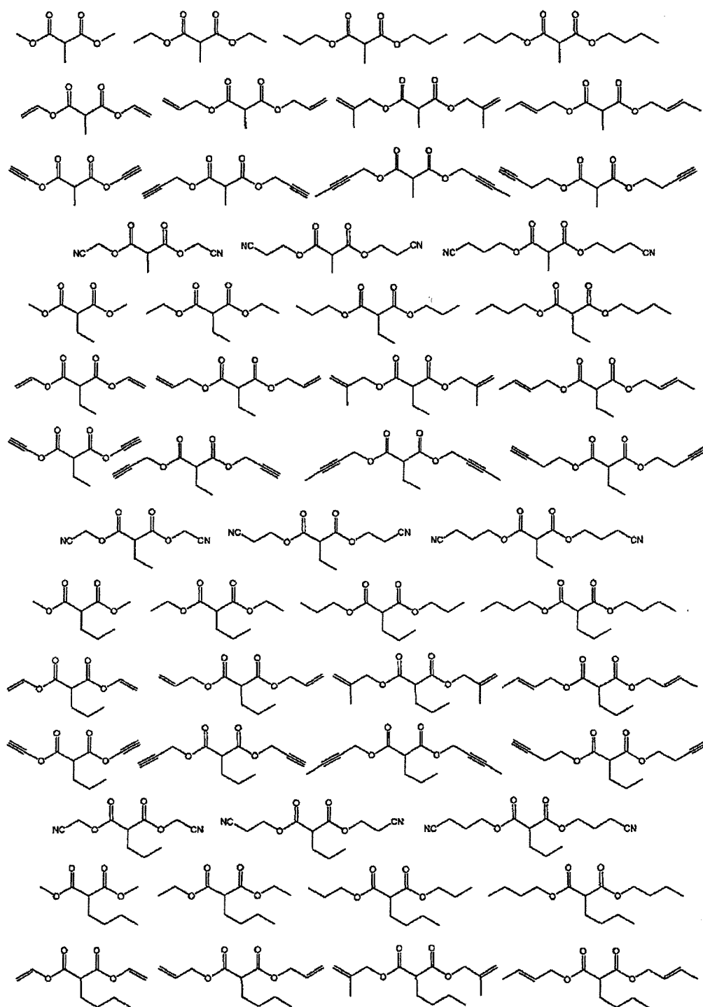
[Chemical formula 19]
