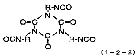
[Chemical formula 29]
