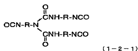
[Chemical formula 27]
