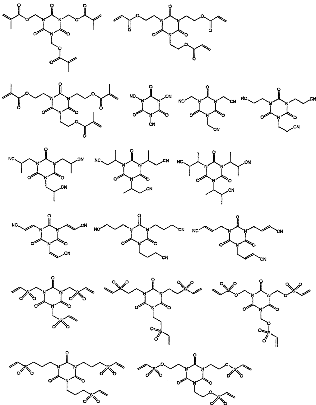
[Chemical formula 34]
