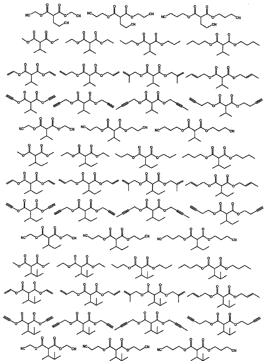
[Chemical formula 22]
