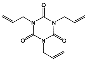
[Chemical formula 50]
