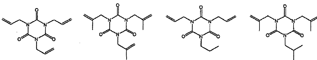
[Chemical formula 39]
