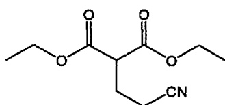
Compound 7: Diethyl 2-(2-cyanoethyl)malonate
