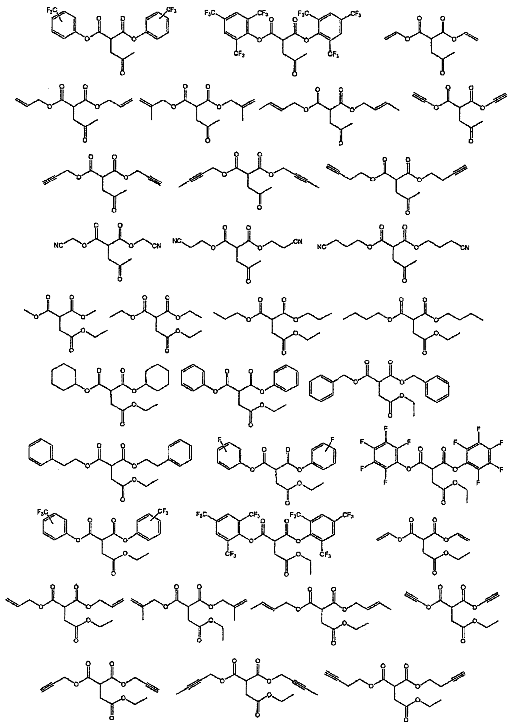
[Chemical formula 10]
