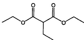
Compound 1: Diethyl ethylmalonate
