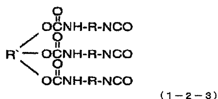
[Chemical formula 29]
