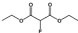
Compound 10: Diethyl fluoromalonate
