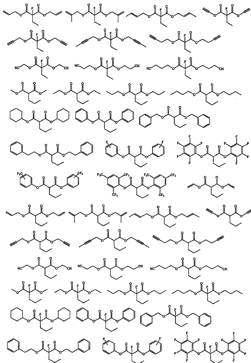
[Chemical formula 6]
