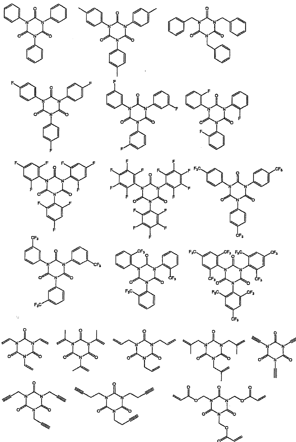
[Chemical formula 33]
