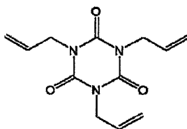
[Chemical formula 40]
