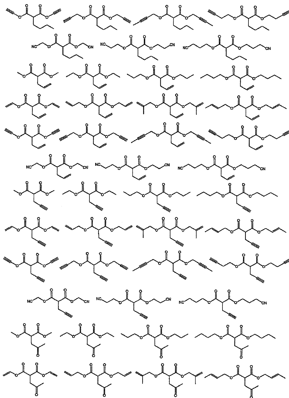
[Chemical formula 16]
