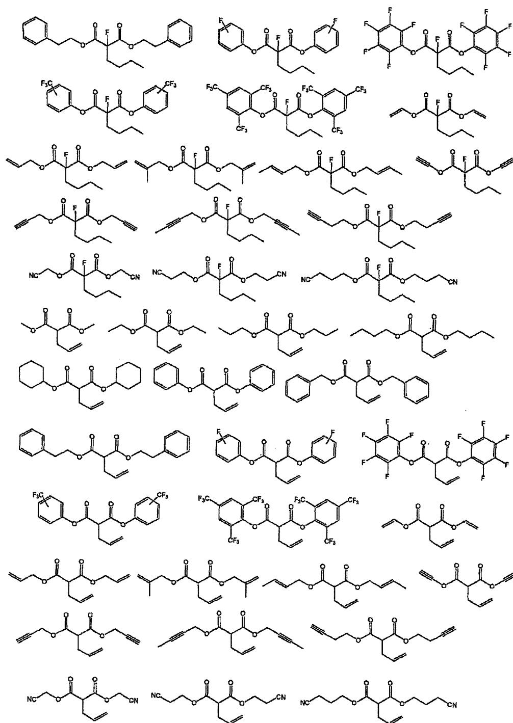
[Chemical formula 8]
