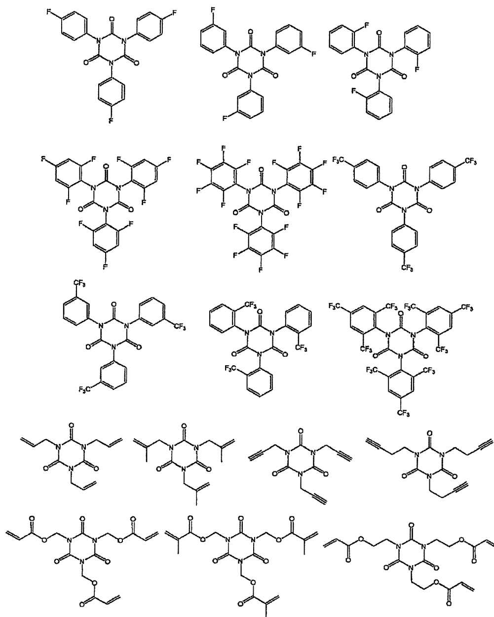
[Chemical formula 36]
