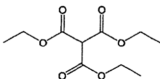
Compound 8: Triethyl methanetricarboxylate
