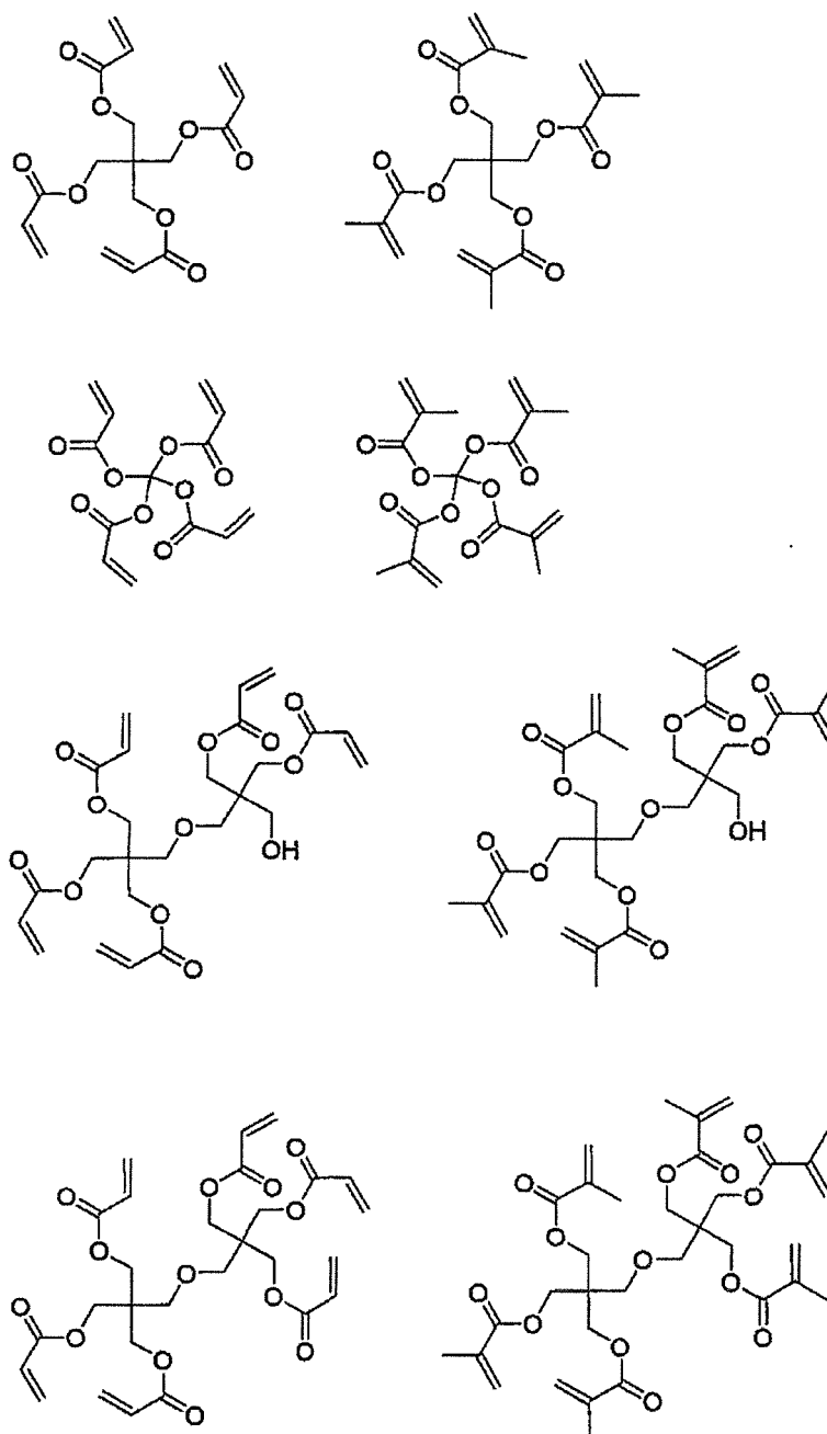
[Chemical formula 42]
