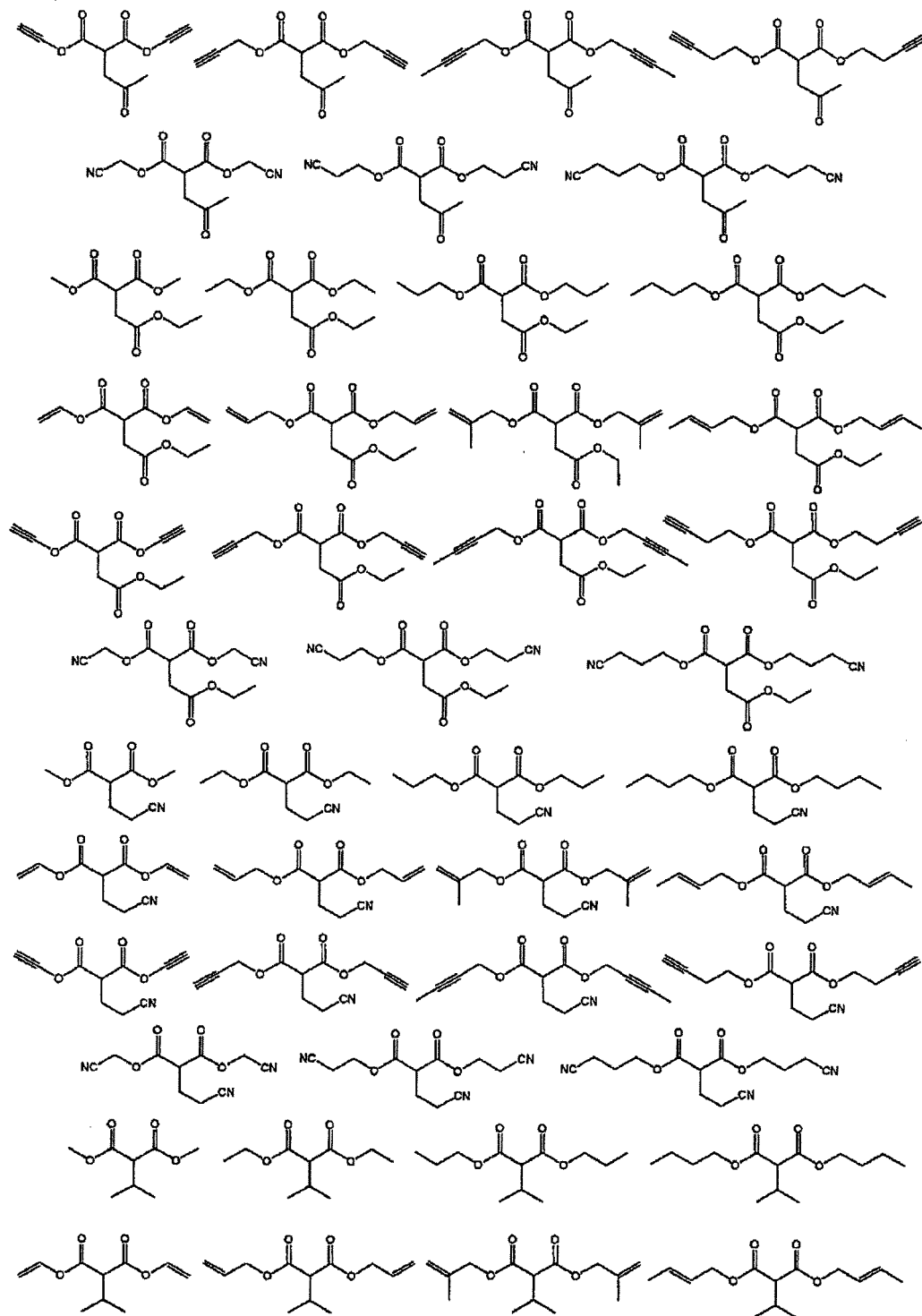
[Chemical formula 17]
