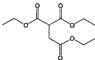
Compound 6: Triethyl 1,1,2-ethanetricarboxylate
