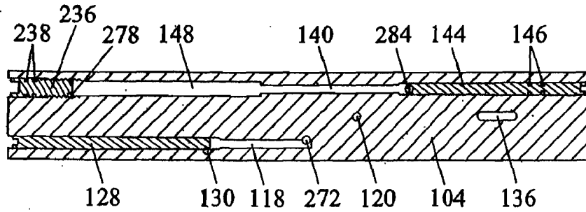
Top Sectional View
