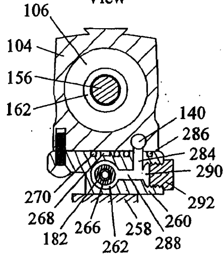
Rear Sectional View
