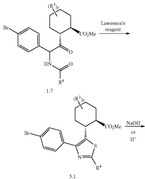
SCHEME 5
