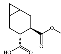
(3R,4R)-4-(methoxycarbonyl)bicyclo[4.1.0]heptane-3-carboxylic acid
