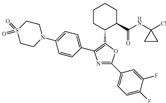
(1R,2R)—N-(1-Cyanocyclopropyl)-2-(2-(3,4-difluorophenyl)-4-(4-(1,1-dioxidothiomorpholino)phenyl)oxazol-5-yl)cyclohexanecarboxamide (Compound 1)
