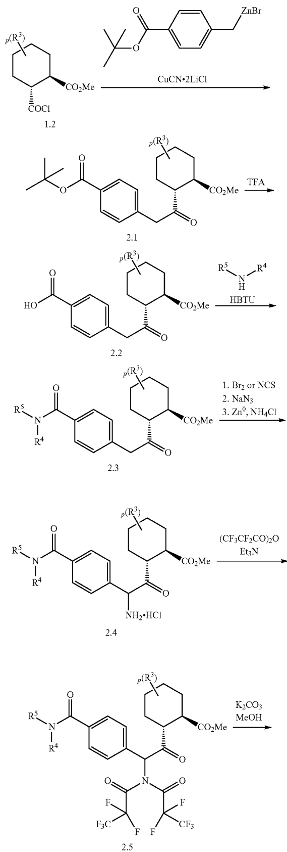
SCHEME 2
