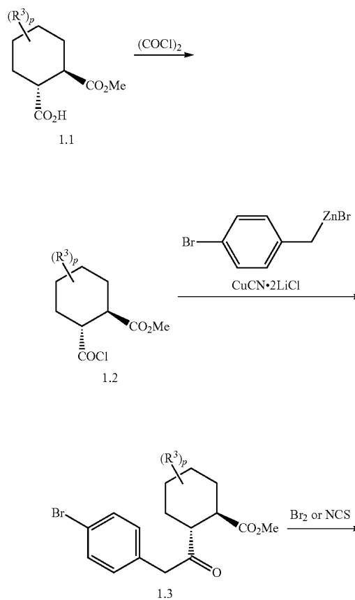
SCHEME 1
