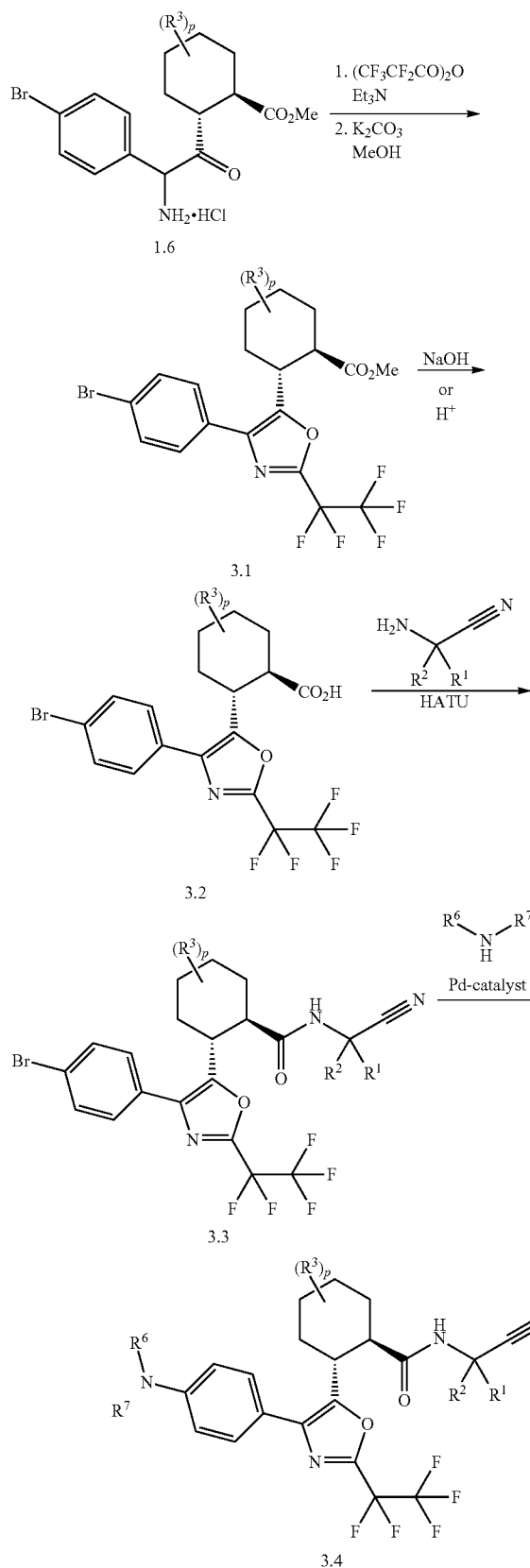
SCHEME 3
