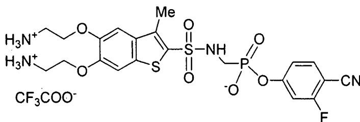
4-cyano-3-fluorophenyl [({[5,6-bis(2-ammonioethoxy)-3-methyl-1-benzothien-2-yl]sulfonyl}-amino)methyl]phosphonate trifluoroacetate
