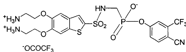
4-cyano-3-(trifluoromethyl)phenyl [({[5,6-bis(2-ammonioethoxy)-1-benzothien-2-yl]-sulfonyl}amino)methyl]phosphonate trifluoroacetate
