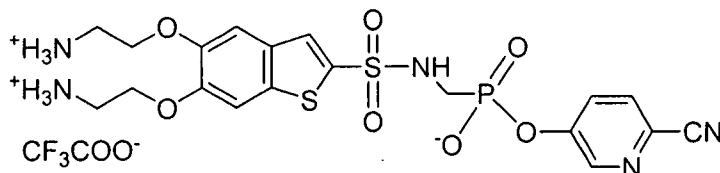
6-cyanopyridin-2-yl-[({[5,6-bis(2-ammonioethoxy)-1-benzothien-2-yl]sulfonyl}amino)-methyl]-phosphonate trifluoroacetate
