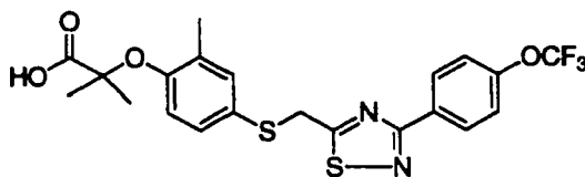
2-Methyl-2-{2-methyl-4-[3-(4-trifluoromethoxy-phenyl)-[1,2,4]thiadiazol-5-ylmethylsulfanyl]-phenoxy}-propionic acid
