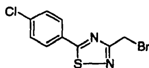
F13 3-Bromomethyl-5-(4-chloro-phenyl)-[1,2,4]thiadiazole
