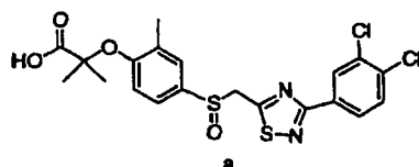
2-(4-(3-(3,4-Dichloro-phenyl)-[1,2,4]thiadiazol-5-ylmethanesulfonyl)-2-methyl-phenoxy)-2-methyl-propanoic acid
