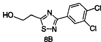
2-[3-(3,4-Dichloro-phenyl)-[1,2,4]thiadiazol-5-yl]-ethanol
