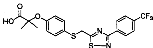
2-Methyl-2-(4-[3-(4-trifluoromethyl-phenyl)-[1,2,4]thiadiazol-5-ylmethylsulfanyl]-phenoxy)-propionic acid
