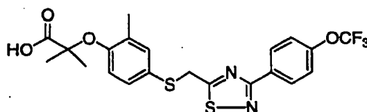
2-Methyl-2-(2-methyl-4-[3-(4-trifluoromethoxy-phenyl)-[1,2,4]thiadiazol-5-ylmethylsulfanyl]-phenoxy)-propionic acid
