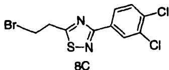
5-(2-Bromo-ethyl)-3-(3,4-dichloro-phenyl)-[1,2,4]thiadiazole
