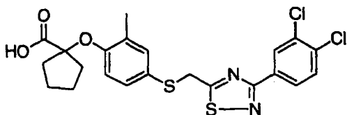
1-(4-[3-(3,4-Dichloro-phenyl)-[1,2,4]thiadiazol-5-ylmethylsulfanyl]-2-methyl-phenoxy)-cyclopentanecarboxylic acid
