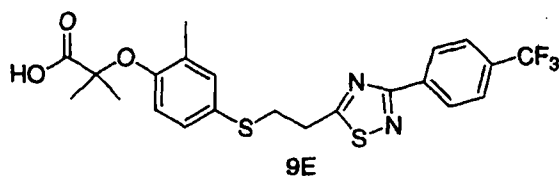
2-Methyl-2-(2-methyl-4-(2-[3-(4-trifluoromethyl-phenyl)-[1,2,4]thiadiazol-5-yl]-ethylsulfanyl)-phenoxy)-propionic acid
