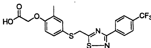
{2-Methyl-4-[3-(4-trifluoromethyl-phenyl)-[1,2,4]thiadiazol-5-ylmethylsulfanyl]-phenoxy}-acetic acid
