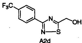
[3-(4-Trifluoromethyl-phenyl)-[1,2,4]thiadiazol-5-yl]-methanol
