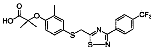
2-Methyl-2-(2-methyl-4-[3-(4-trifluoromethyl-phenyl)-[1,2,4]thiadiazol-5-ylmethylsulfanyl]-phenoxy)-propionic acid
