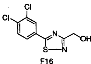
F16 [5-(3,4-Dichloro-phenyl)-[1,2,4]thiadiazol-3-yl]-methanol
