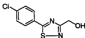
F12 [5-(4-Chloro-phenyl)-[1,2,4]thiadiazol-3-yl]-methanol
