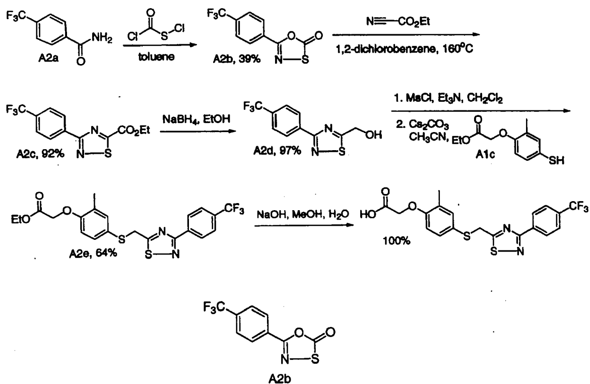
5-(4-Trifluoromethyl-phenyl)-[1,3,4]oxathiazol-2-one
