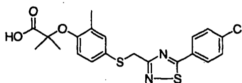
2-{4-[5-(4-Chloro-phenyl)-[1,2,4]thiadiazol-3-ylmethylsulfanyl]-2-methyl-phenoxy}-2-methyl-propionic acid
