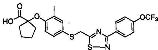
1-(2-Methyl-4-[3-(4-trifluoromethoxy-phenyl)-[1,2,4]thiadiazol-5-ylmethylsulfanyl]-phenoxy)-cyclopentanecarboxylic acid
