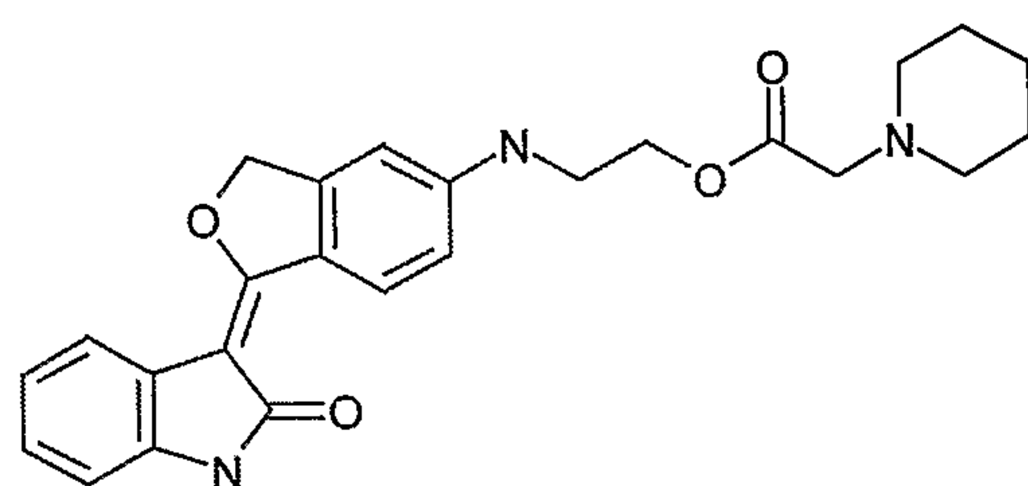
Piperidin-1-yl-acetic acid 2-[1-(2-oxo-1,2-dihydro-indol-3-ylidene)-1,3-dihydro-isobenzofuran-5-ylamino]-ethyl ester
