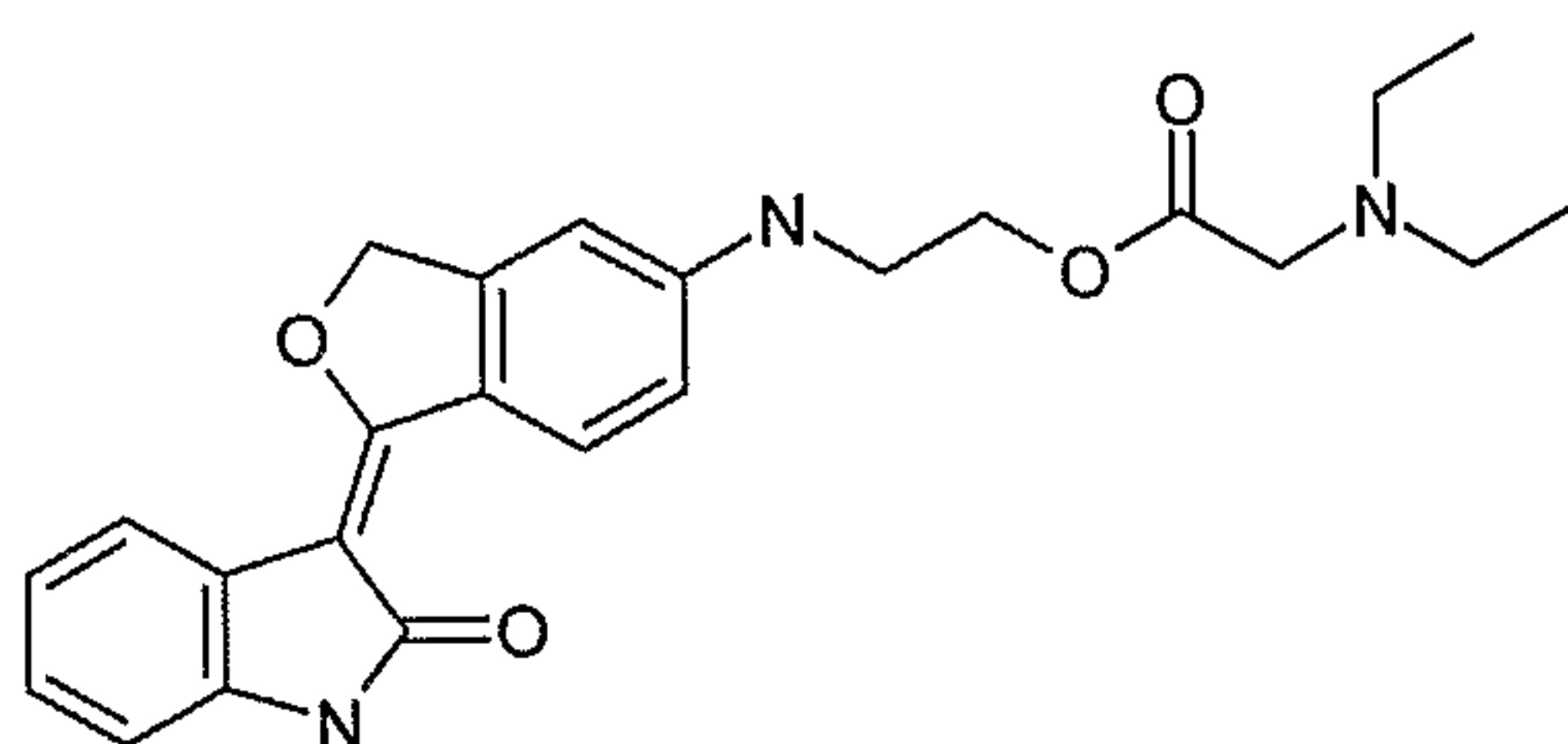
Diethylamino-acetic acid 2-[1-(2-oxo-1,2-dihydro-indol-3-ylidene)-1,3-dihydro-isobenzofuran-5-ylamino]-ethyl ester
