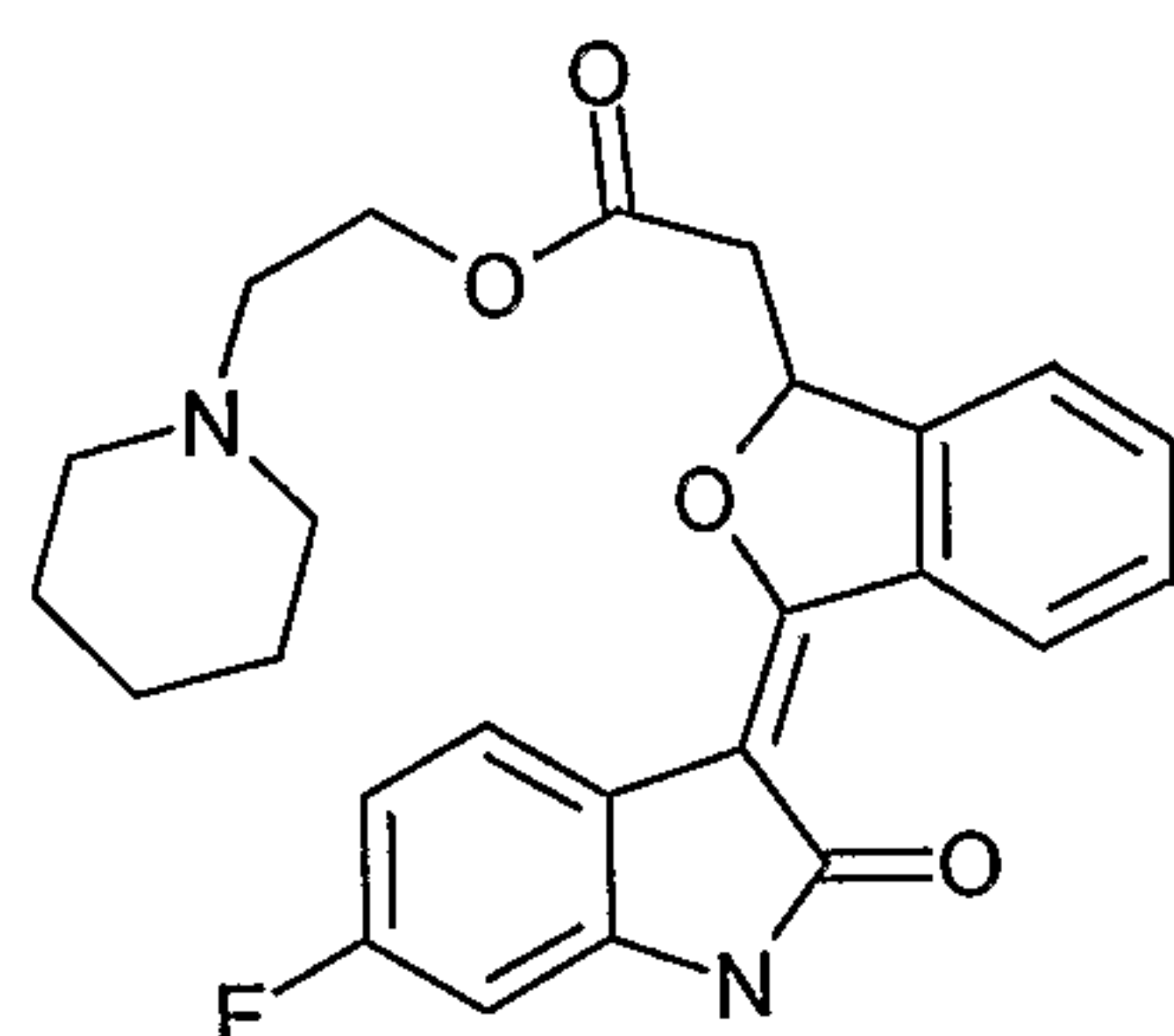
[3-(6-Fluoro-2-oxo-1,2-dihydro-indol-3-ylidene)-1,3-dihydro-isobenzofuran-1-yl]-acetic acid 2-piperidin-1-yl-ethyl ester
