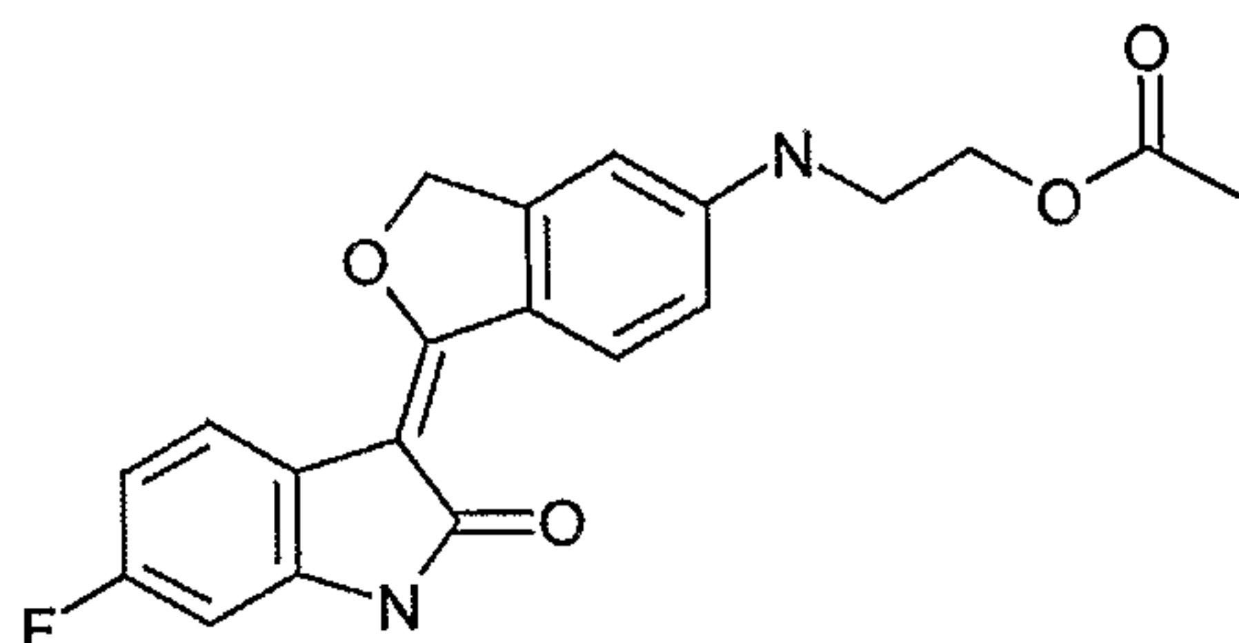
Acetic acid 2-[1-(6-fluoro-2-oxo-1,2-dihydro-indol-3-ylidene)-1,3-dihydro-isobenzofuran-5-ylamino]-ethyl ester
