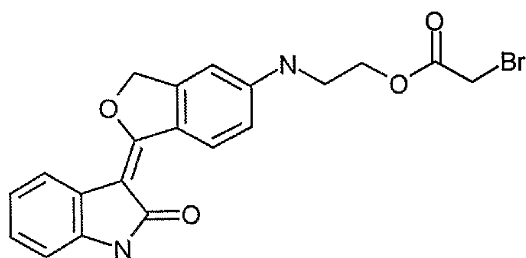
Bromo-acetic acid 2-[1-(2-oxo-1,2-dihydro-indol-3-ylidene)-1,3-dihydro-isobenzofuran-5-ylamino]-ethyl ester
