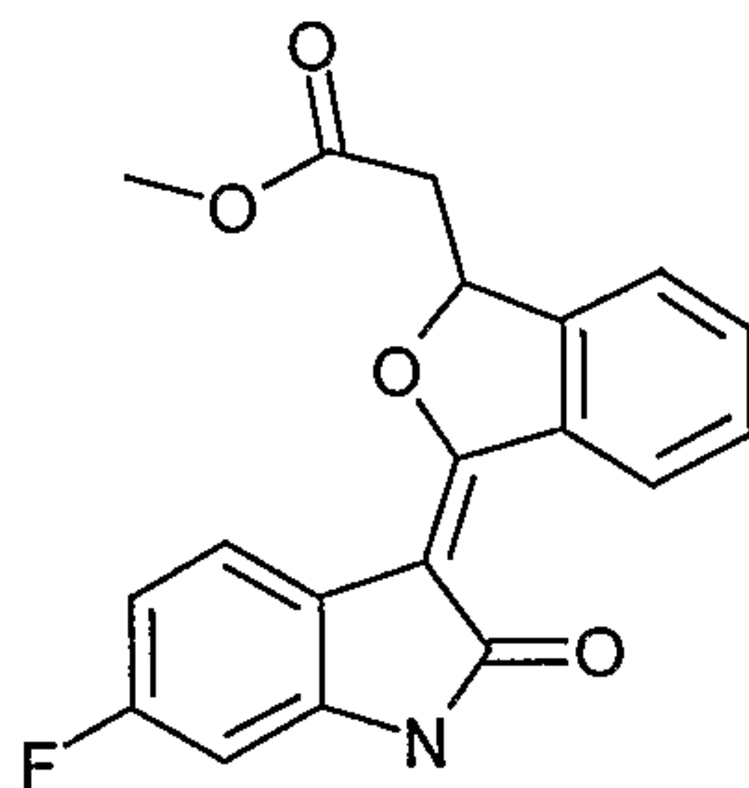
[3-(6-Fluoro-2-oxo-1,2-dihydro-indol-3-ylidene)-1,3-dihydro-isobenzofuran-1-yl]-acetic acid methyl ester
