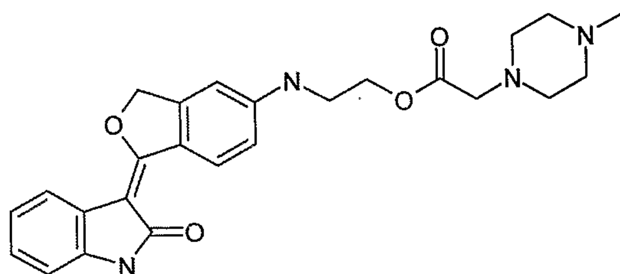
(4-Methyl-piperazin-1-yl)-acetic acid 2-[1-(2-oxo-1,2-dihydro-indol-3-ylidene)-1,3-dihydro-isobenzofuran-5-ylamino]-ethyl ester
