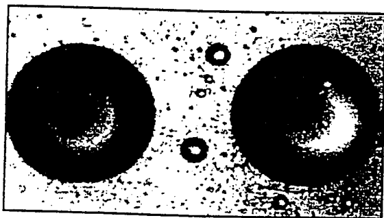
No UV, 24 hr. growth
