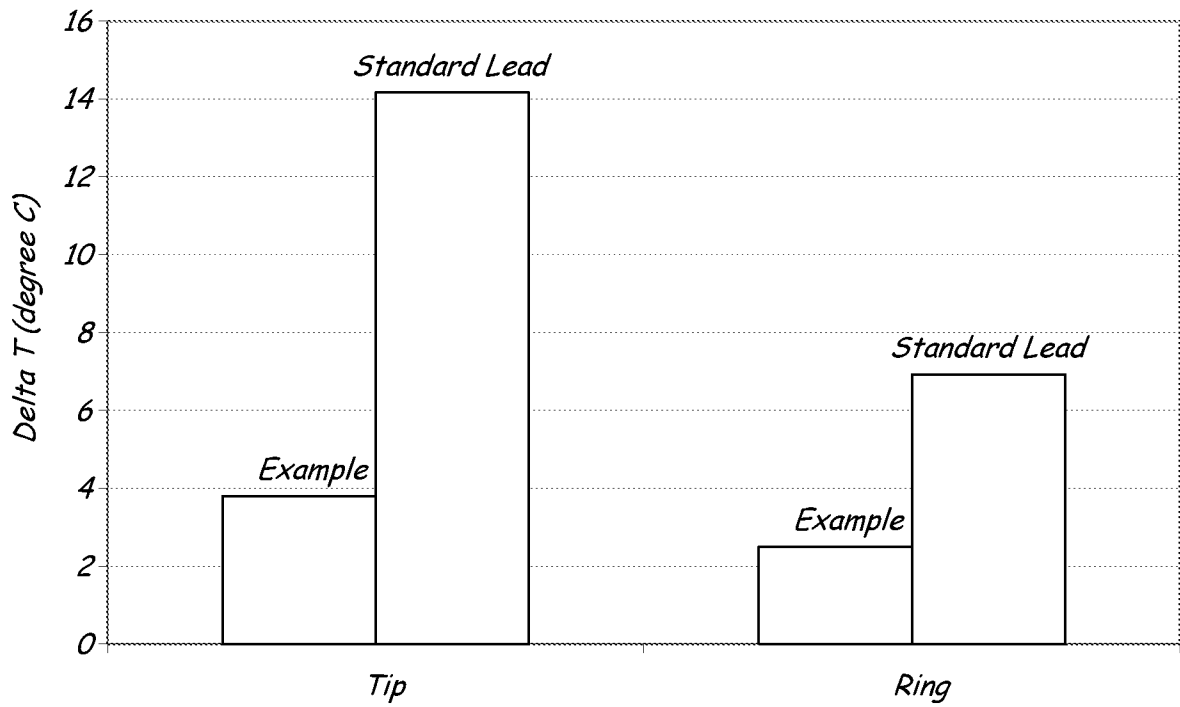
Comparison of Example to Standard Defibrillation Lead
