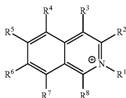
ISOQUINOLINIUM
