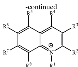
QUINOLINIUM
