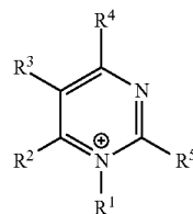
PYRAMIDIUM
