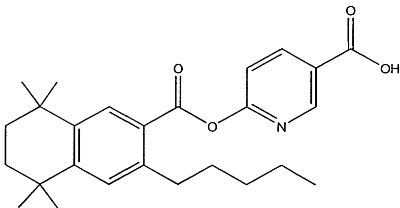
Compound I
