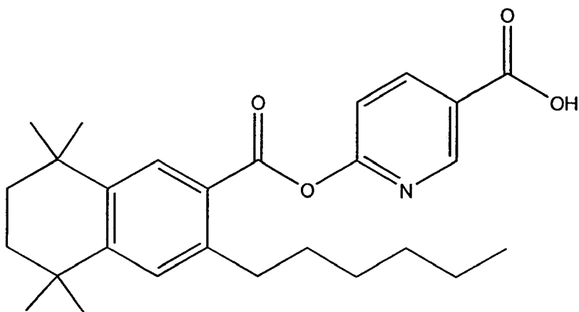
Compound III
