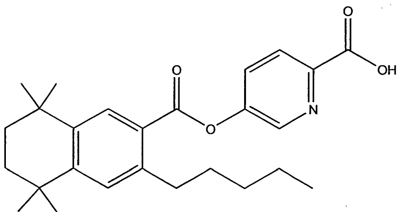
Compound II
