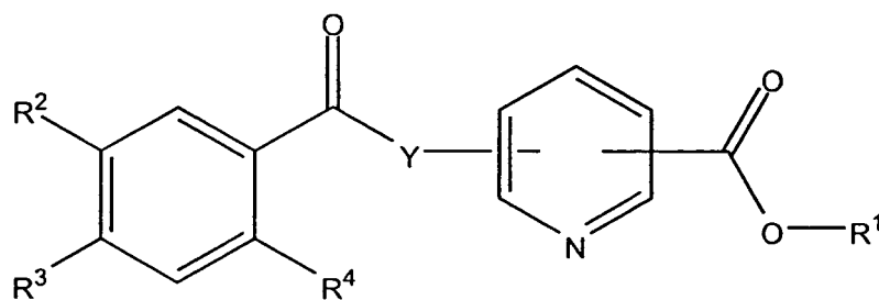
Formula I
