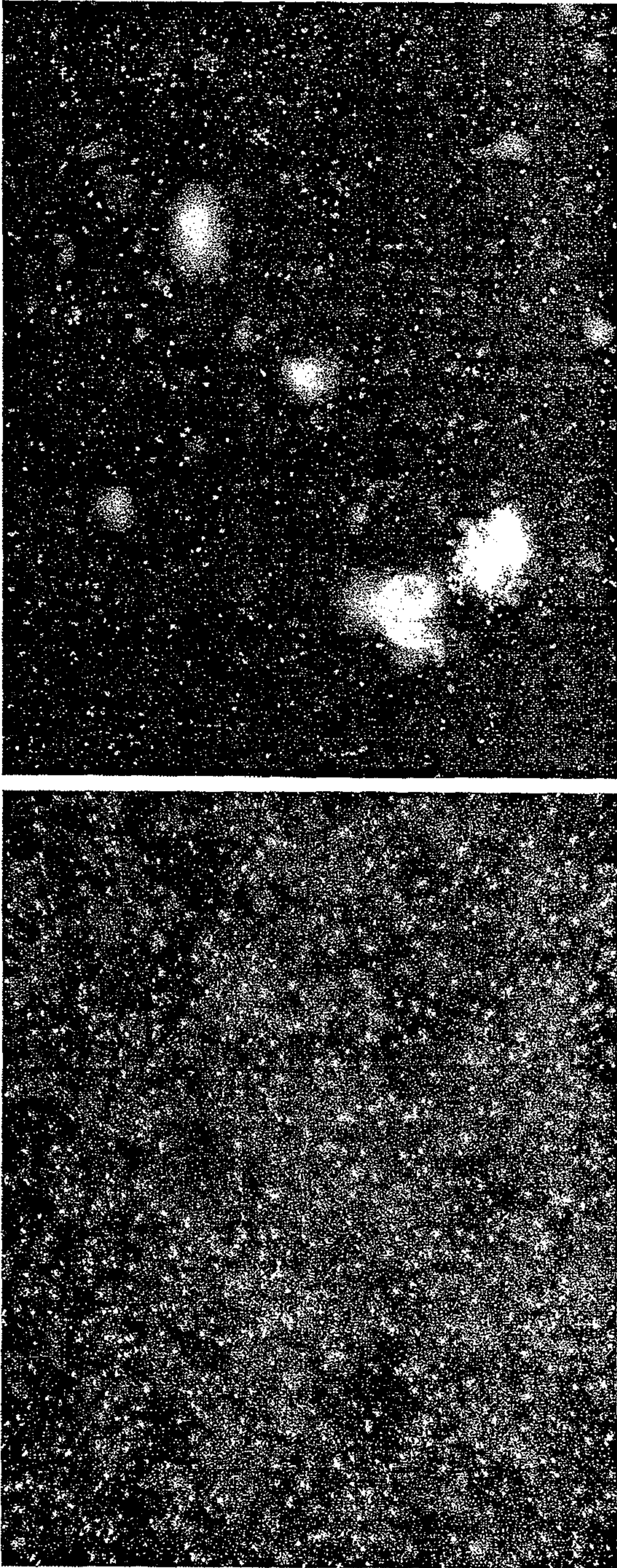
Salmonella
