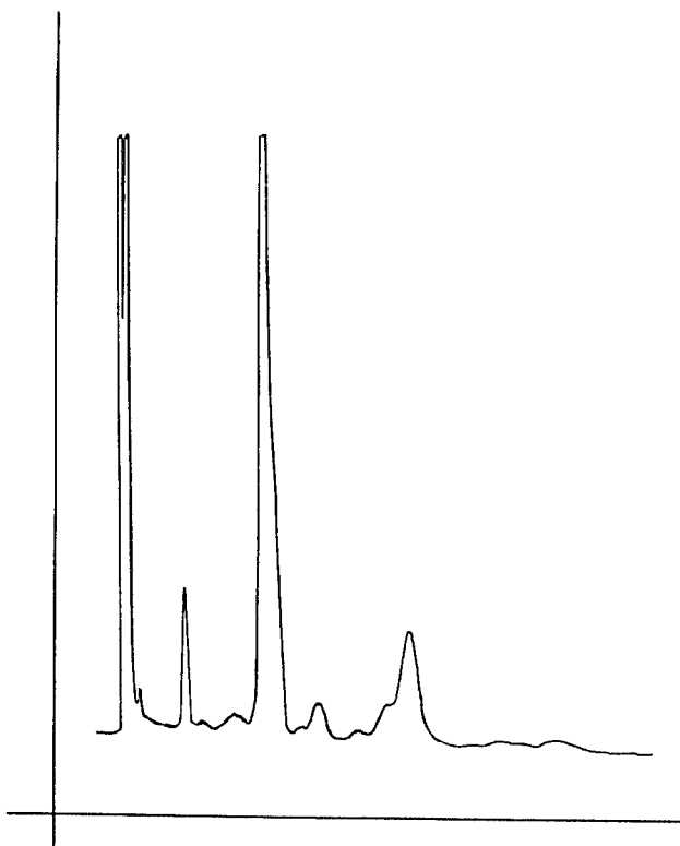
GLC PROFILE FOR EXAMPLE IX
