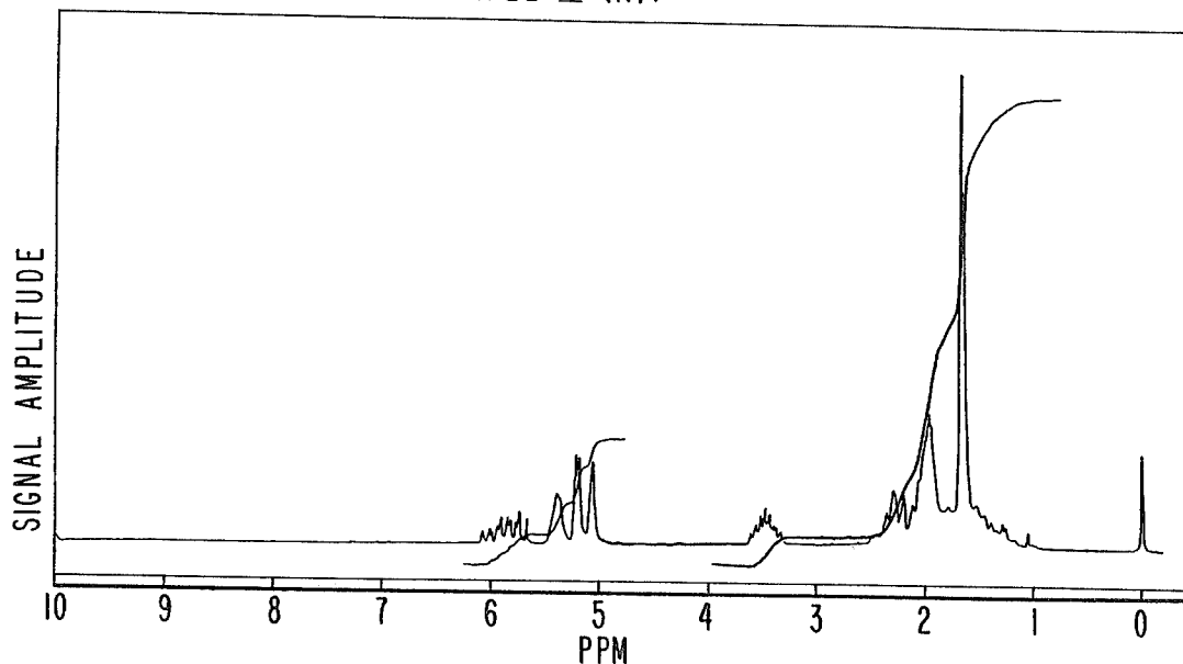
NMR SPECTRUM FOR EXAMPLE V (A).
