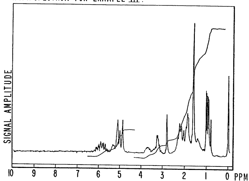
NMR SPECTRUM FOR EXAMPLE III.
