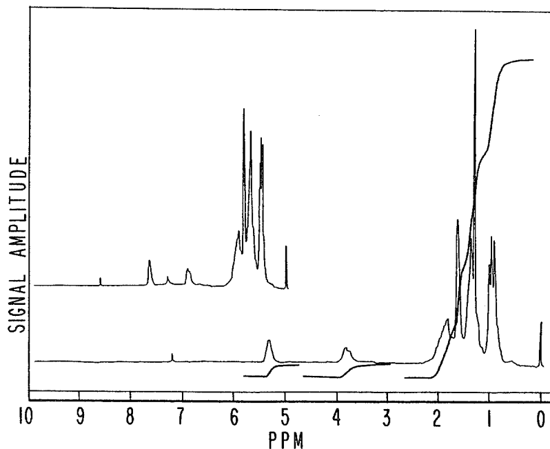
N M R SPECTRUM FOR EXAMPLE VII(A).
