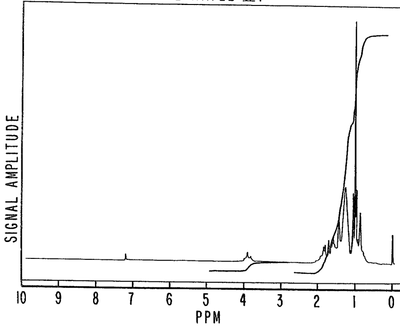
NMR SPECTRUM FOR EXAMPLE X.
