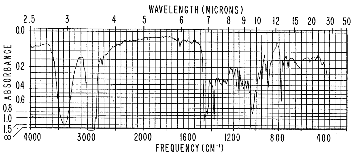
I R SPECTRUM FOR EXAMPLE VII(A).
