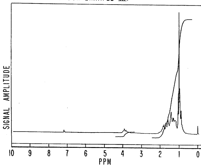
NMR SPECTRUM FOR EXAMPLE IX.
