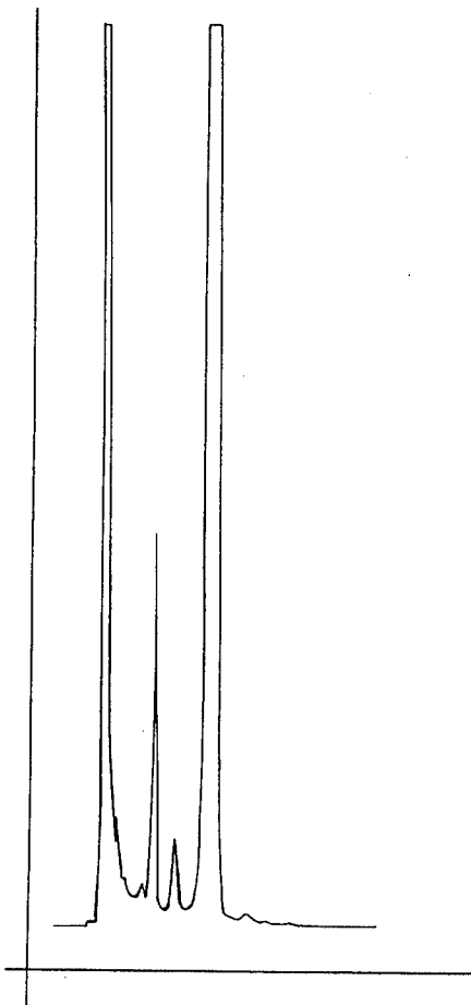
GLC PROFILE FOR EXAMPLE XXXIV
