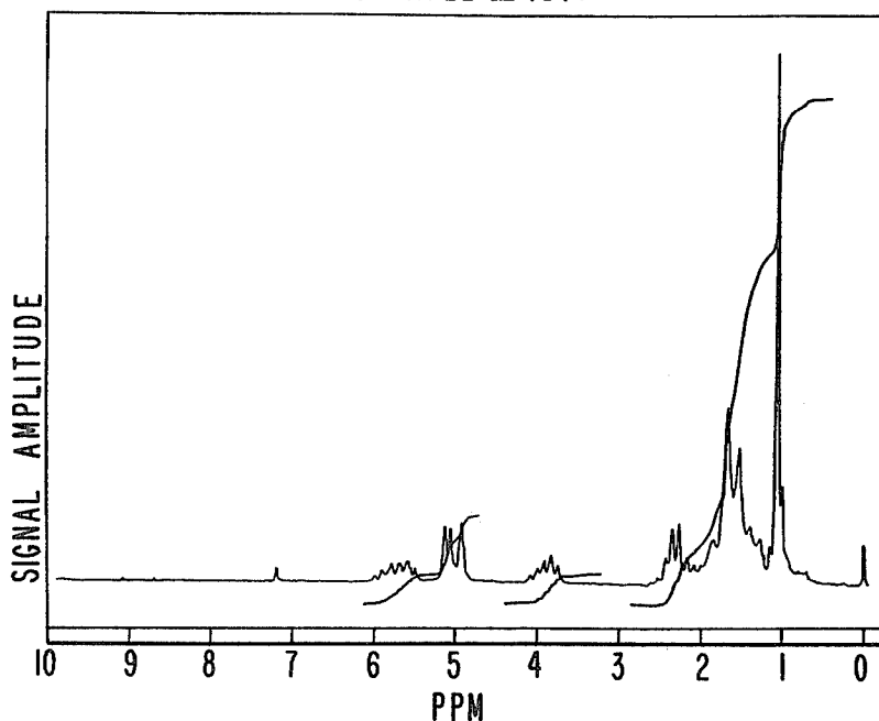
NMR SPECTRUM FOR EXAMPLE V(B).
