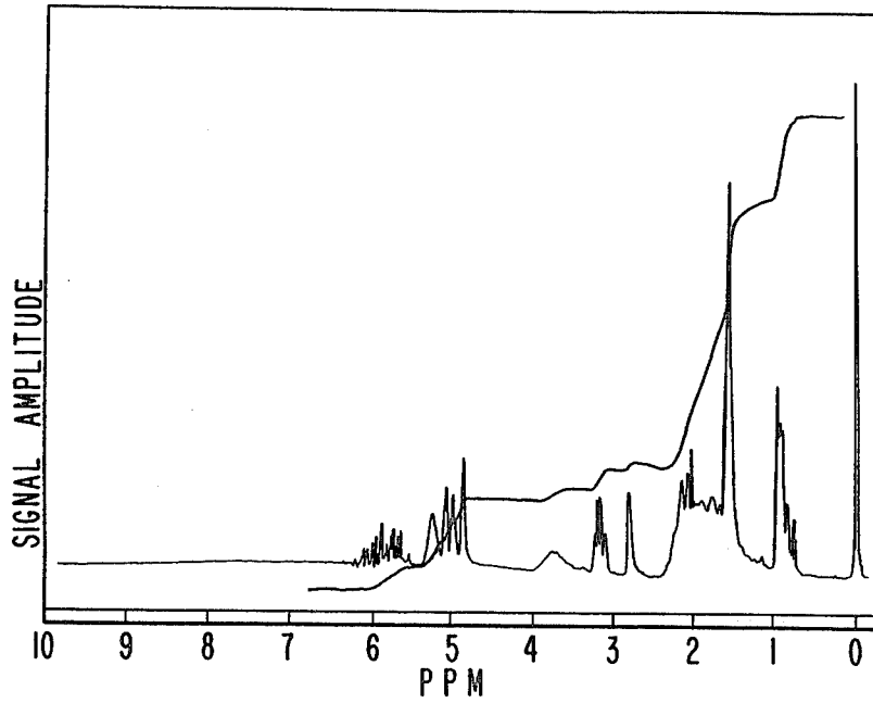
NMR SPECTRUM FOR EXAMPLE IV.
