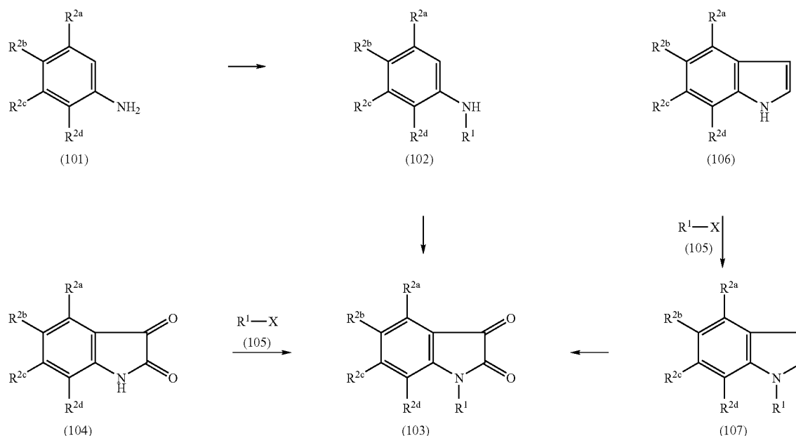
REACTION SCHEME 1
