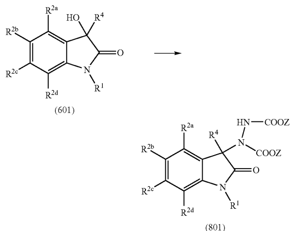
REACTION SCHEME 8
