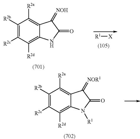
REACTION SCHEME 7
