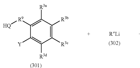
REACTION SCHEME 3
