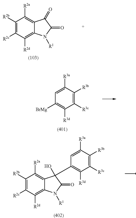
REACTION SCHEME 4
