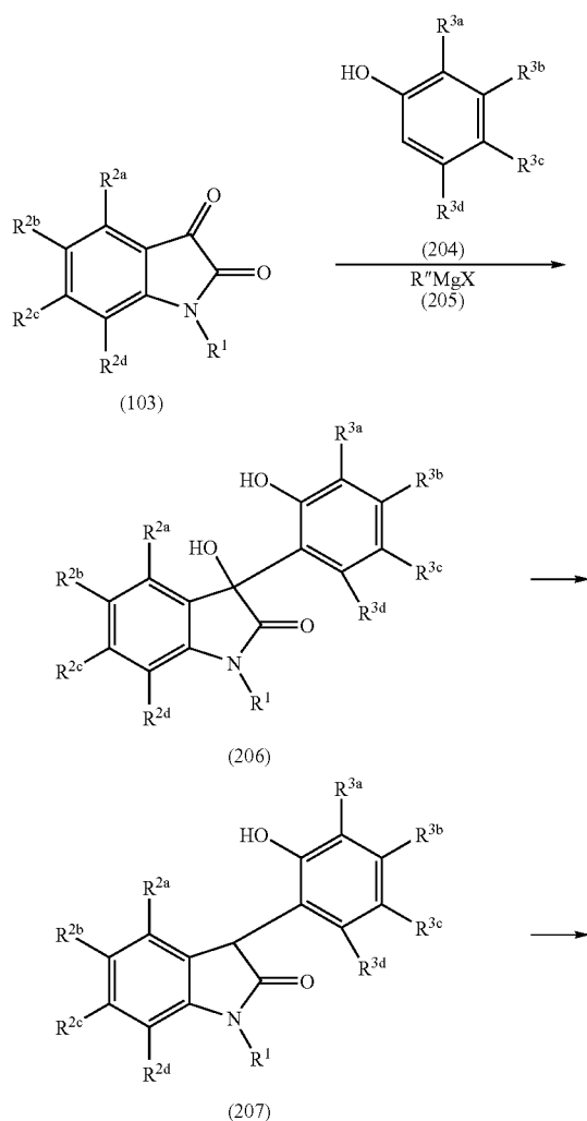
REACTION SCHEME 2
