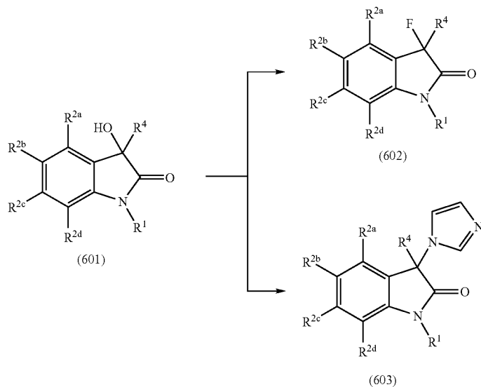
REACTION SCHEME 6
