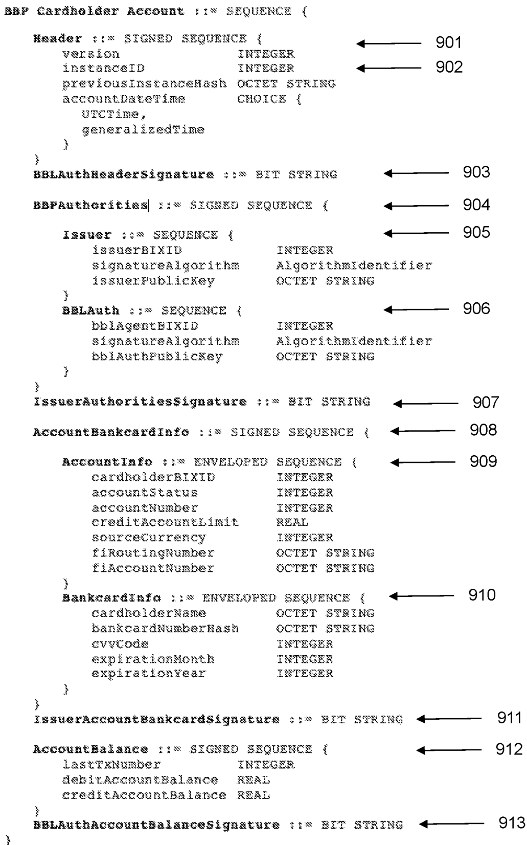
FIG 9: Permitted Version of the Cardholder Virtual Account
