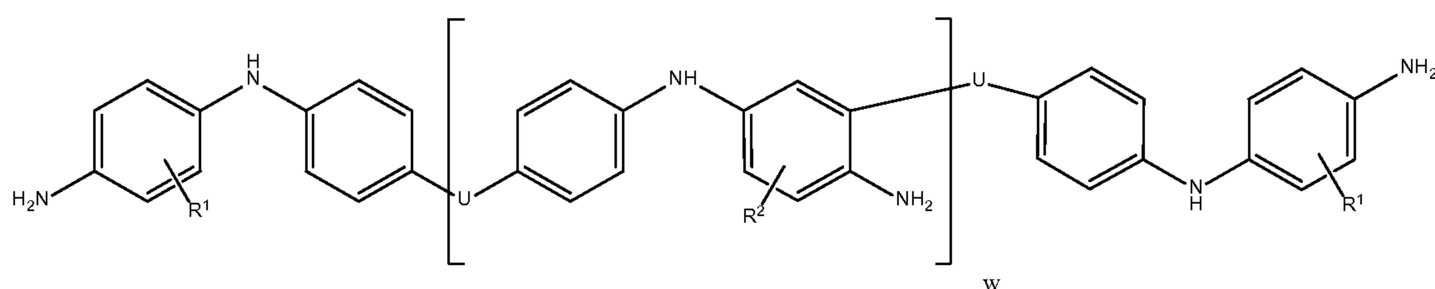
Formula (1)
