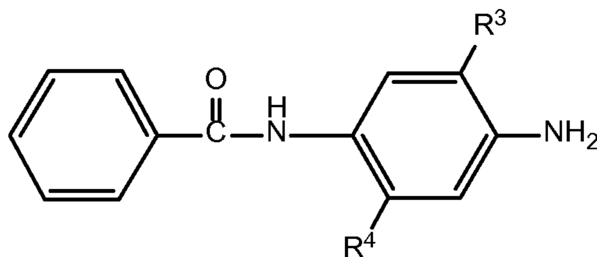
Formula (4)
