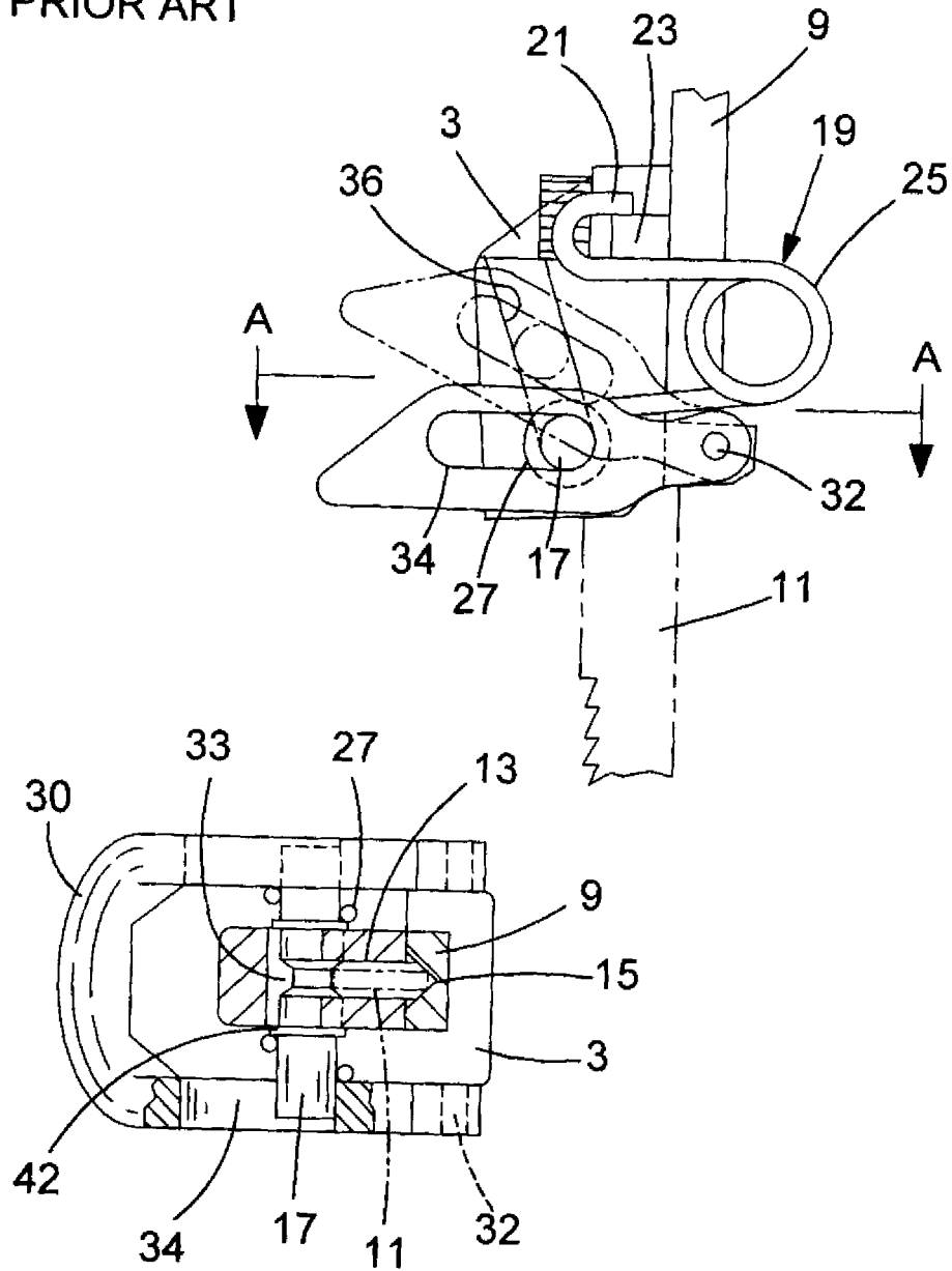
FIG.2 PRIOR ART
