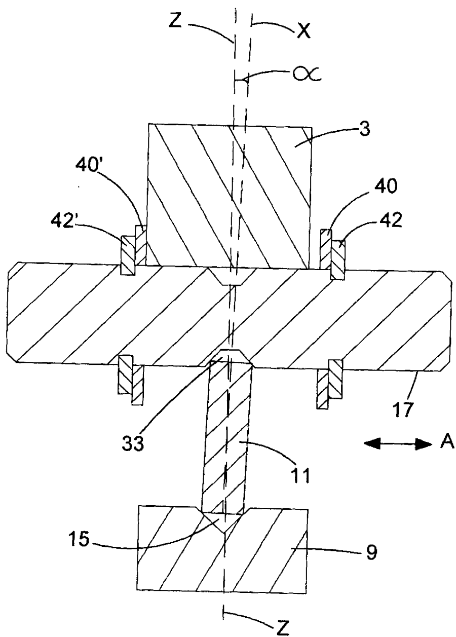
FIG.3 PRIOR ART
