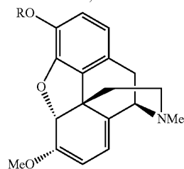
thebaine, R = Me oripavine, R = H
