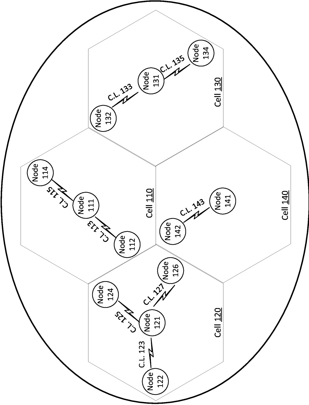
WLAN 100
