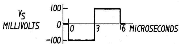
FIG. 8B SECONDARY OUTPUT VOLTAGE
