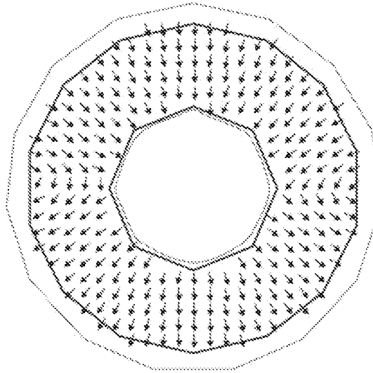
HE11, Horizontal Polarization
