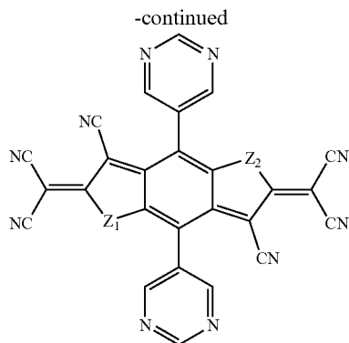
Z_1 = Z_2 = \text{O} Compound O-135 Z_1 = Z_2 = \text{S} Compound S-135 Z_1 = Z_2 = \text{Se} Compound Se-135
