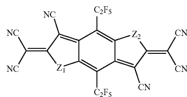
Z_1 = Z_2 = \text{O} Compound O-141 Z_1 = Z_2 = \text{S} Compound S-141 Z_1 = Z_2 = \text{Se} Compound Se-141
