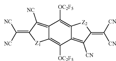
Z_1 = Z_2 = \text{O} Compound O-142 Z_1 = Z_2 = \text{S} Compound S-142 Z_1 = Z_2 = \text{Se} Compound Se-142
