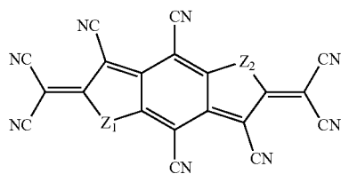
Z_1 = Z_2 = \text{O} Compound O-138 Z_1 = Z_2 = \text{S} Compound S-138 Z_1 = Z_2 = \text{Se} Compound Se-138
