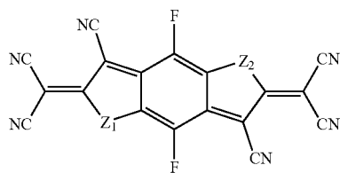
Z_1 = Z_2 = \text{O} Compound O-137 Z_1 = Z_2 = \text{S} Compound S-137 Z_1 = Z_2 = \text{Se} Compound Se-137
