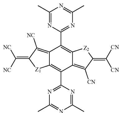
Z_1 = Z_2 = \text{O} Compound O-136 Z_1 = Z_2 = \text{S} Compound S-136 Z_1 = Z_2 = \text{Se} Compound Se-136
