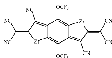
Z_1 = Z_2 = \text{O} Compound O-140 Z_1 = Z_2 = \text{S} Compound S-140 Z_1 = Z_2 = \text{Se} Compound Se-140
