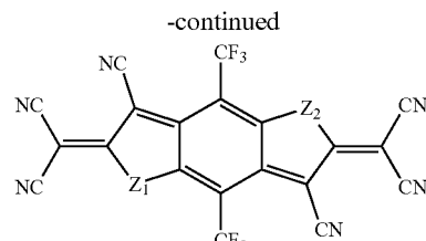
Z_1 = Z_2 = \text{O} Compound O-139 Z_1 = Z_2 = \text{S} Compound S-139 Z_1 = Z_2 = \text{Se} Compound Se-139
