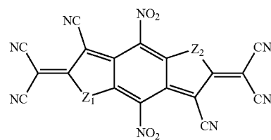
Z_1 = Z_2 = \text{O} Compound O-143 Z_1 = Z_2 = \text{S} Compound S-143 Z_1 = Z_2 = \text{Se} Compound Se-143
