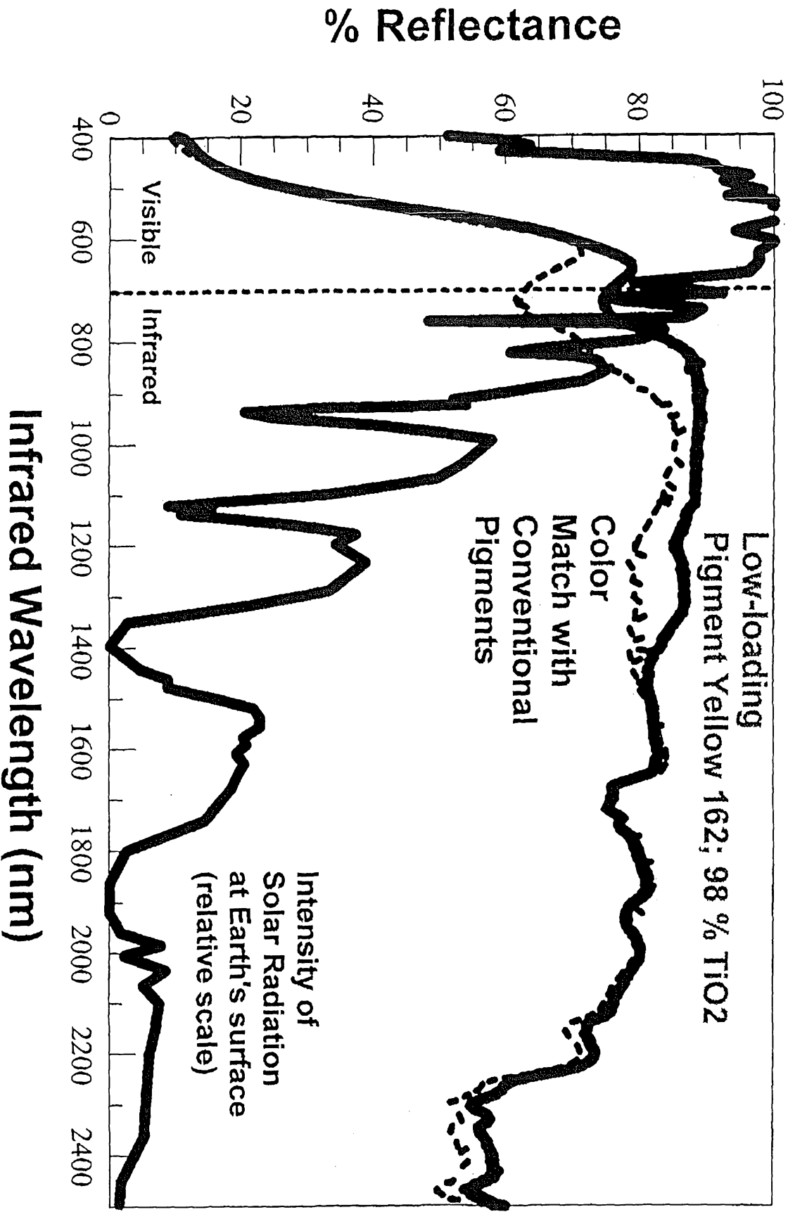
Figure 2. Color and IR Comparison Low-loading Pigment Yellow 162 vs. Color Match
