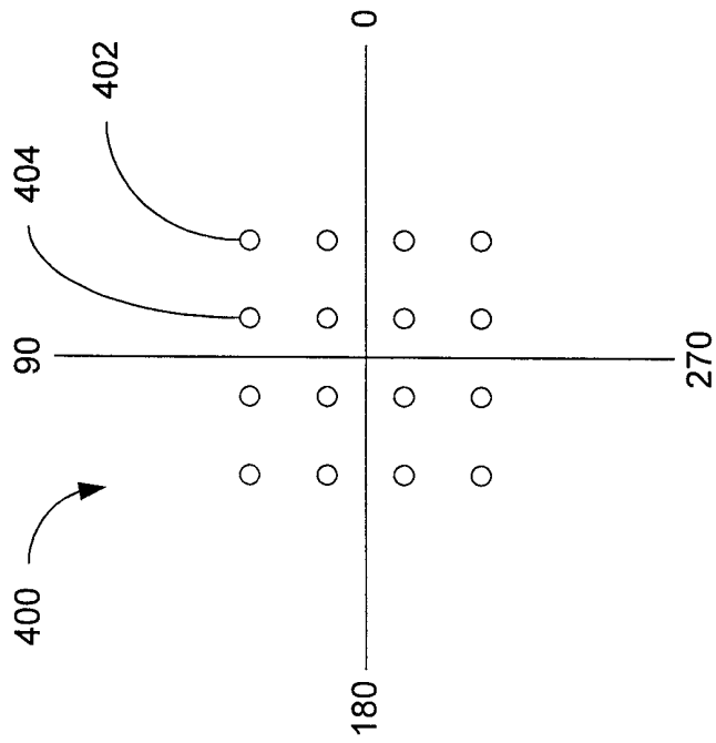
4 - BIT CONSTELLATION
