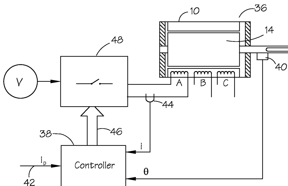
Fig 2 Prior Art
