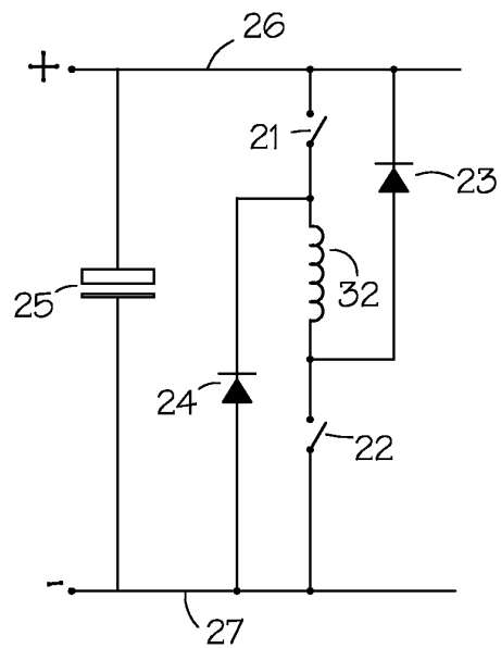
Fig 3 Prior Art
