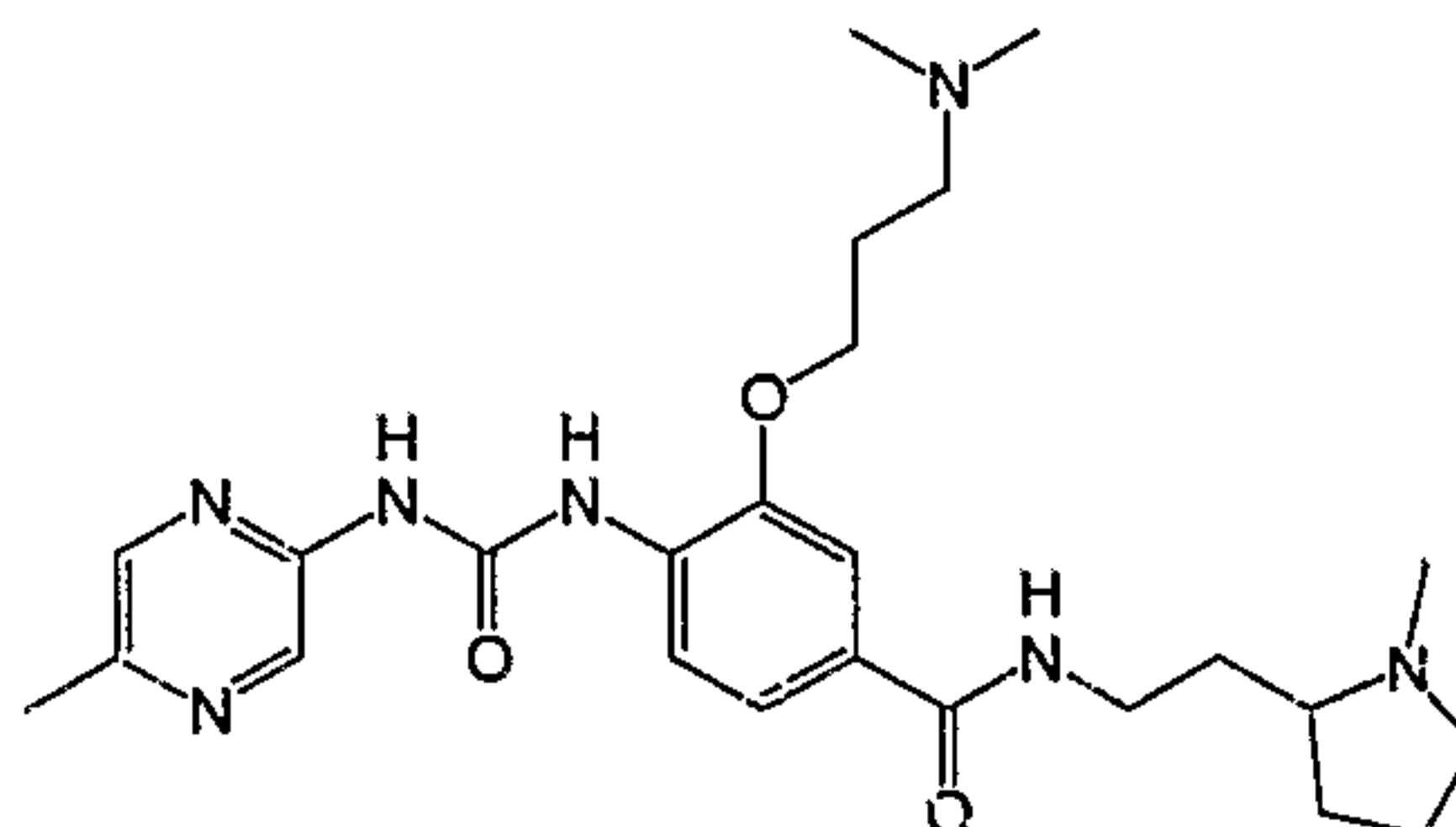
3-(3-Dimethylamino-propoxy)-4-[3-(5-methyl-pyrazin-2-yl)-ureido]-N-[2-(1-methyl-pyrrolidin-2-yl)-ethyl]-benzamide
