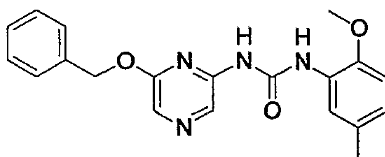
1-(6-Benzyloxy-pyrazin-2-yl)-3-(2-methoxy-5-methyl-phenyl)-urea
