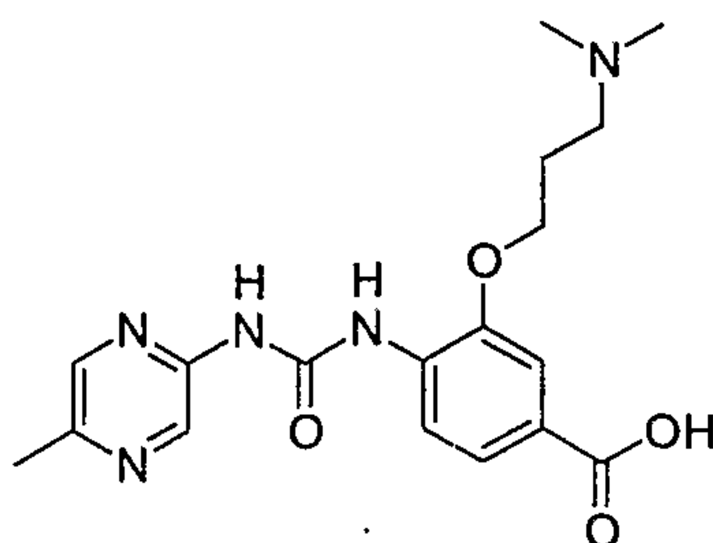
3-(3-Dimethylamino-propoxy)-4-[3-(5-methyl-pyrazin-2-yl)-ureido]-benzoic acid
