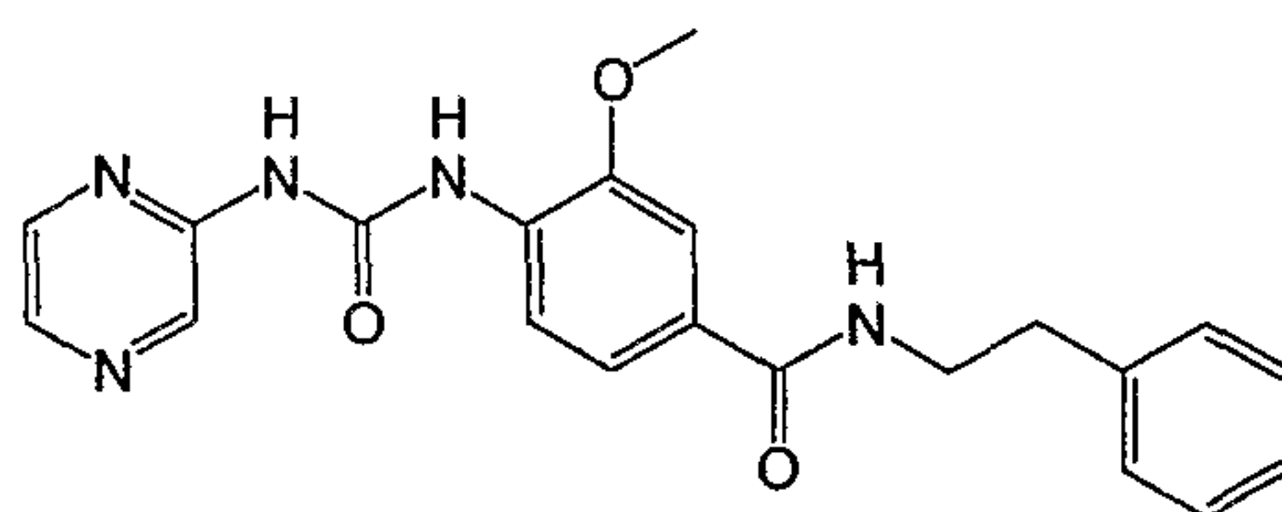
3-Methoxy-N-phenethyl-4-(3-pyrazin-2-yl-ureido)-benzamide
