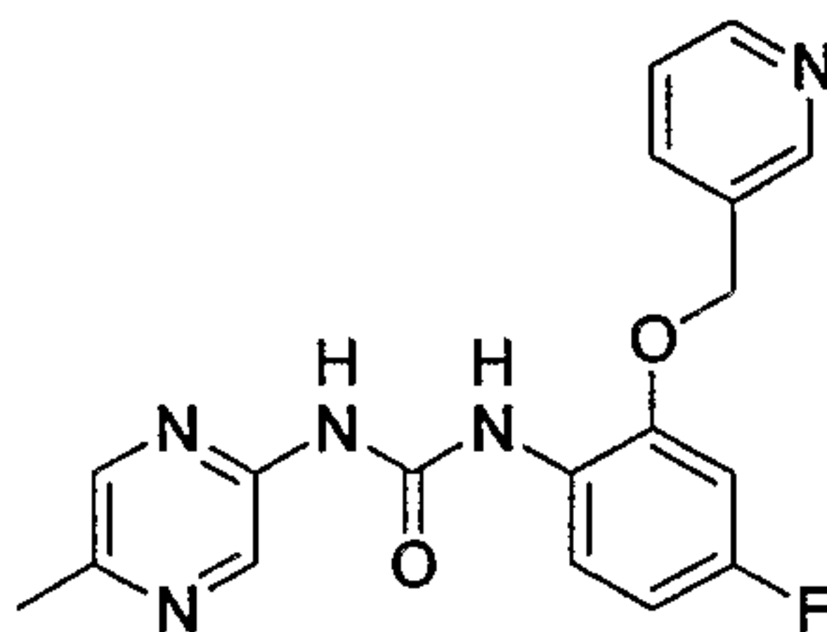
1-[4-Fluoro-2-(pyridin-3-ylmethoxy)-phenyl]-3-(5-methyl-pyrazin-2-yl)-urea
