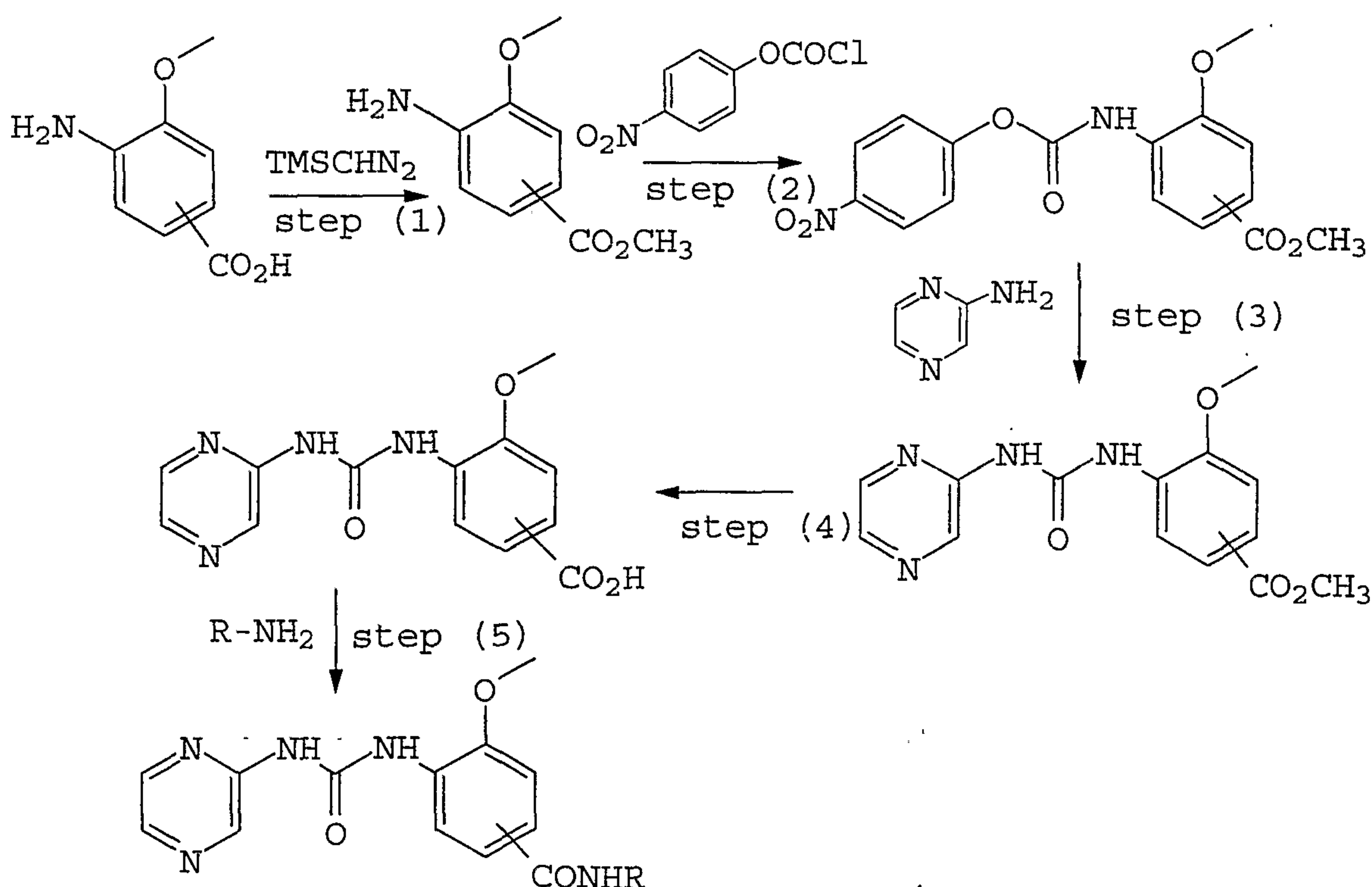
General Scheme 2
