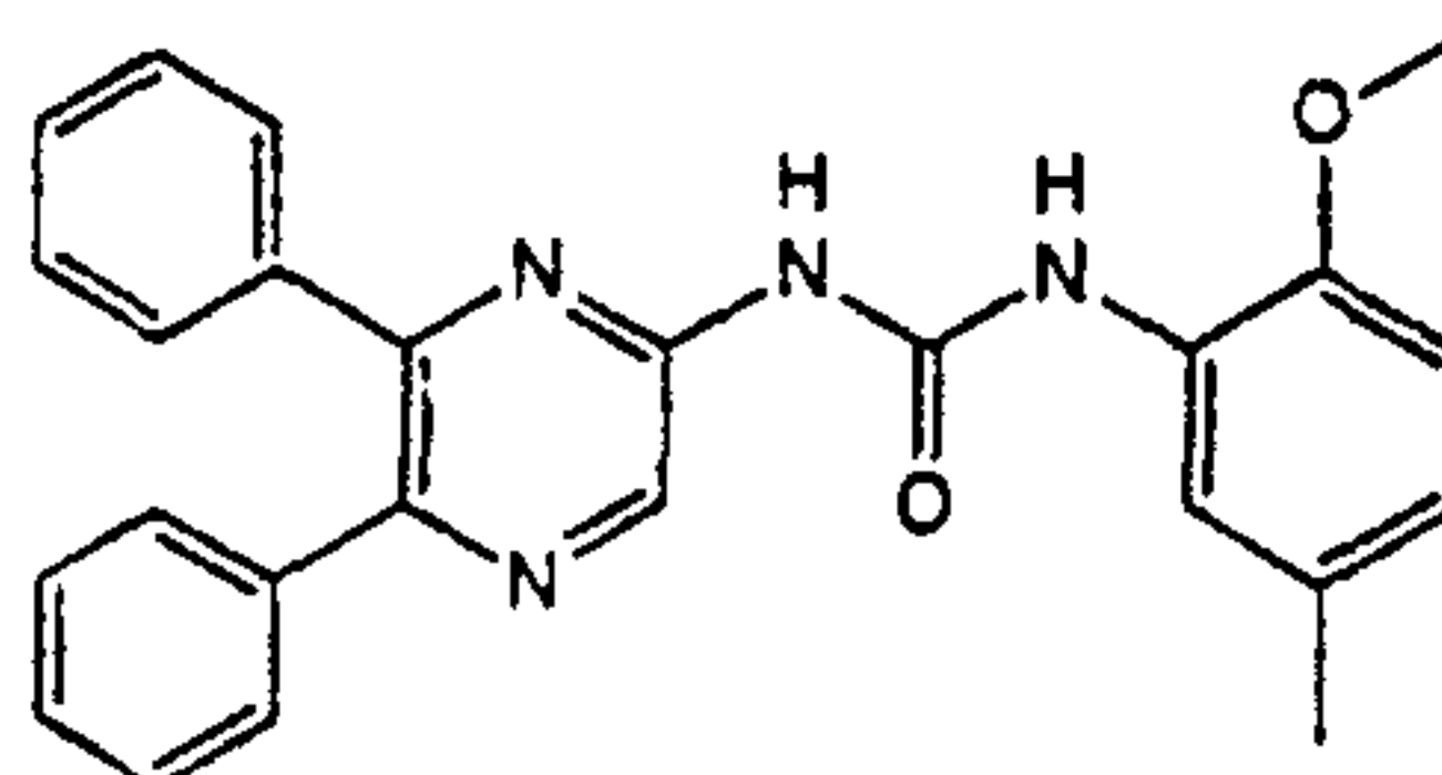
1-(5,6-Diphenyl-pyrazin-2-yl)-3-(2-methoxy-5-methyl-phenyl)-urea
