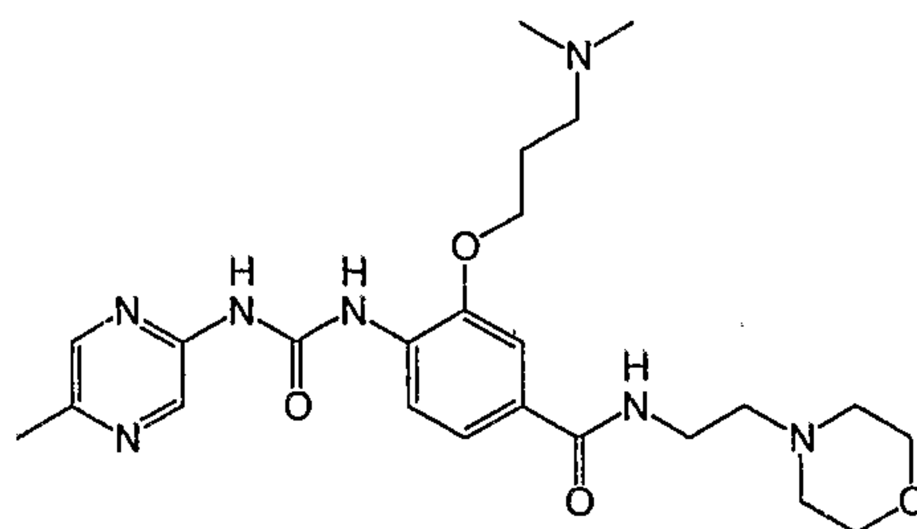
3-(3-Dimethylamino-propoxy)-4-[3-(5-methyl-pyrazin-2-yl)-ureido]-N-(2-morpholin-4-yl-ethyl)-benzamide
