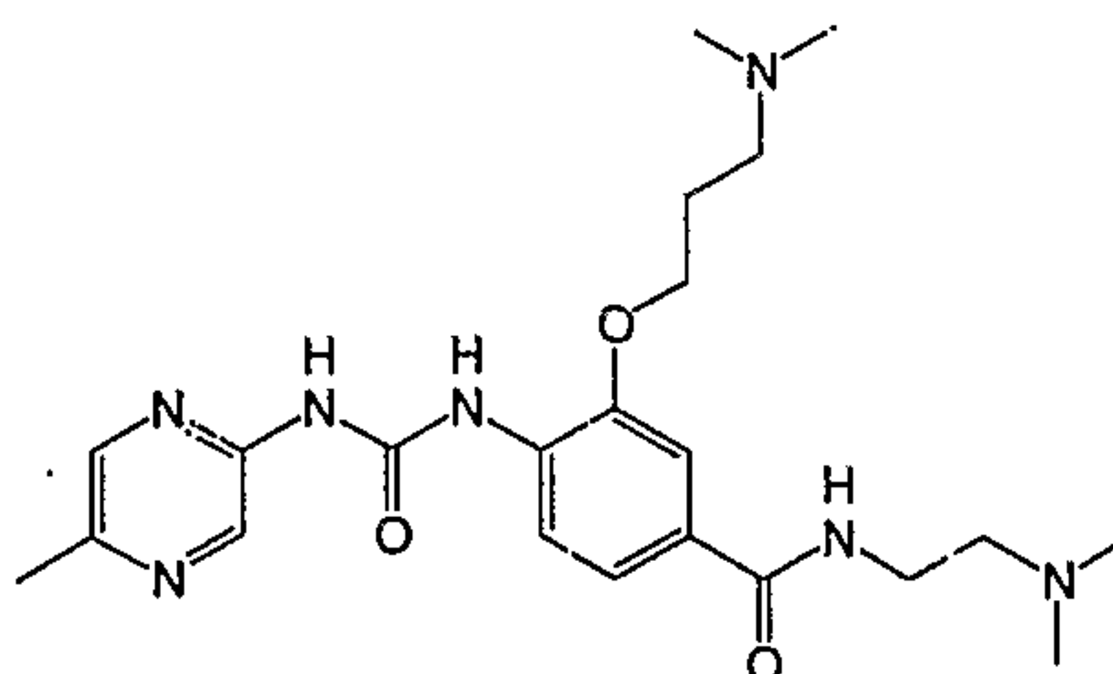
N-(2-Dimethylamino-ethyl)-3-(3-dimethylamino-propoxy)-4-[3-(5-methyl-pyrazin-2-yl)-ureido]-benzamide
