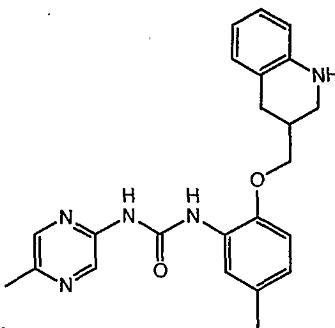
1-(5-Methyl-pyrazin-2-yl)-3-[5-methyl-2-(1,2,3,4-tetrahydro-quinolin-3-ylmethoxy)-phenyl]-urea
