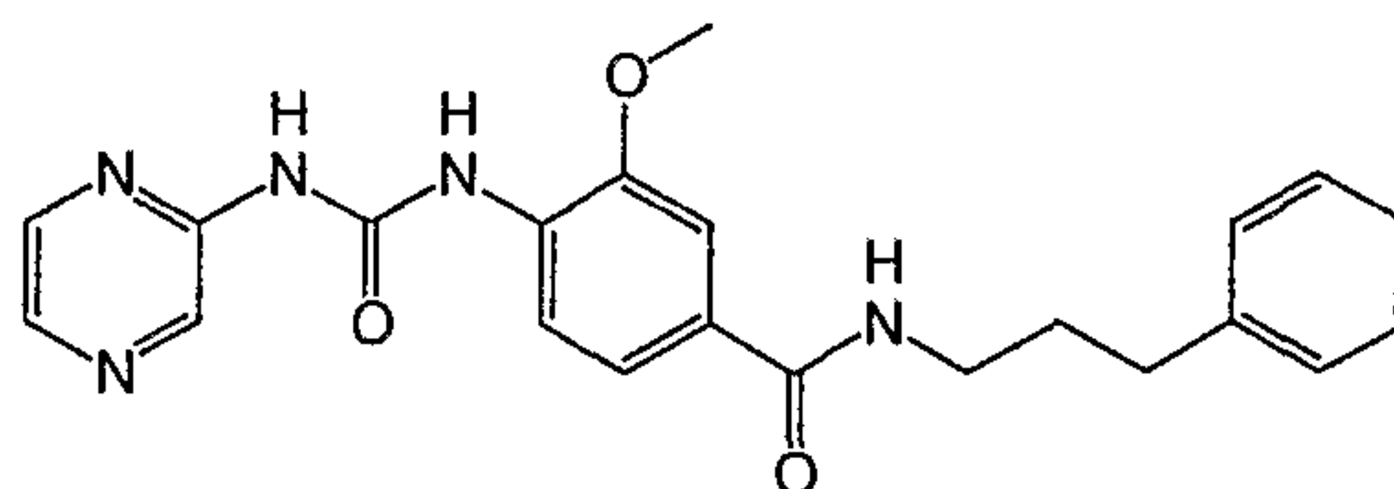
3-Methoxy-N-(3-phenyl-propyl)-4-(3-pyrazin-2-yl-ureido)-benzamide
