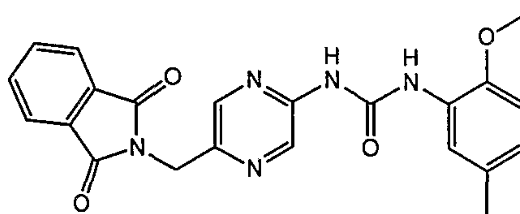
1-[5-(1,3-Dioxo-1,3-dihydro-isoindol-2-ylmethyl)-pyrazin-2-yl]-3-(2-methoxy-5-methyl-phenyl)-urea
