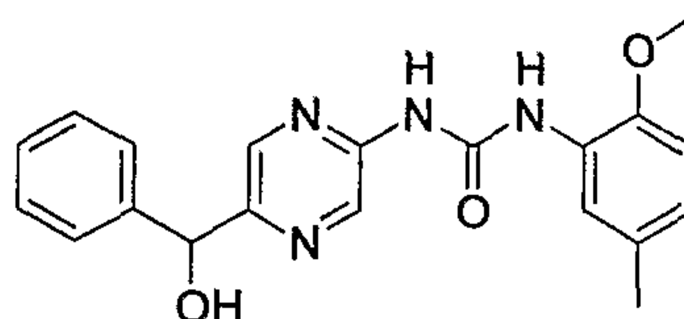
1-[5-(Hydroxy-phenyl-methyl)-pyrazin-2-yl]-3-(2-methoxy-5-methyl-phenyl)-urea
