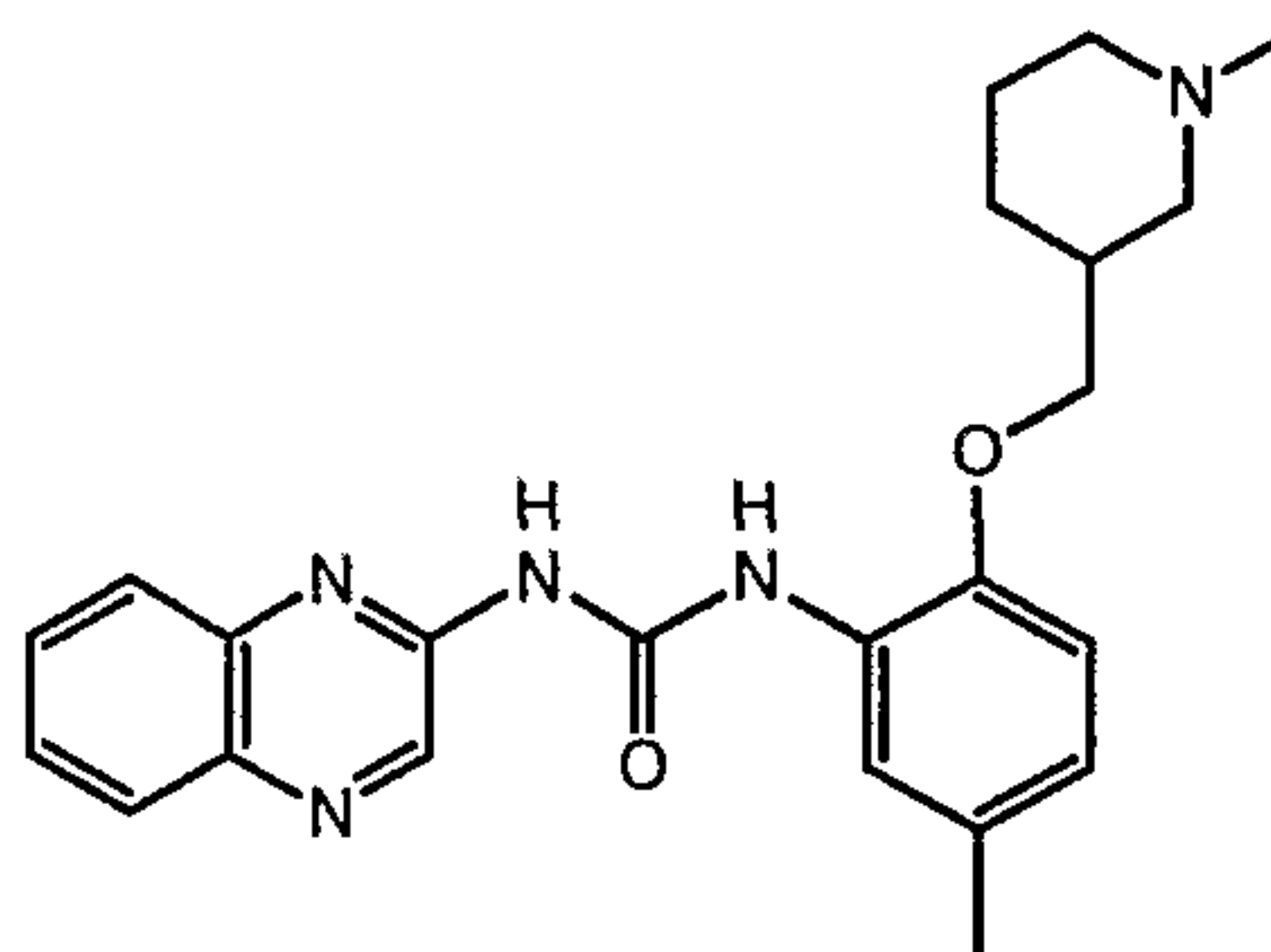
1-[5-Methyl-2-(1-methyl-piperidin-3-ylmethoxy)-phenyl]-3-quinoxalin-2-yl-urea
