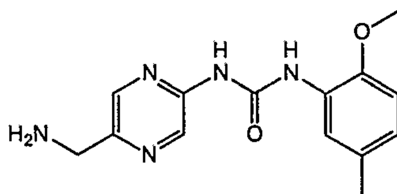
1-(5-Aminomethyl-pyrazin-2-yl)-3-(2-methoxy-5-methyl-phenyl)-urea
