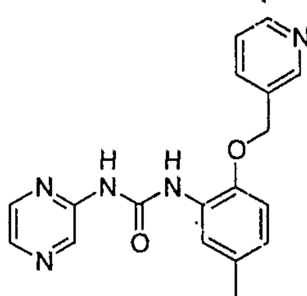
1-[5-Methyl-2-(pyridin-3-ylmethoxy)-phenyl]-3-pyrazin-2-yl-urea
