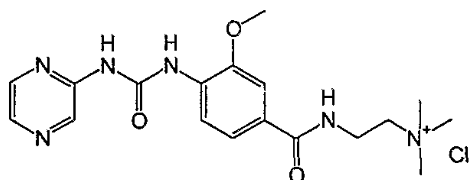
{2-[3-Methoxy-4-(3-pyrazin-2-yl-ureido)-benzoylamino]-ethyl}-trimethyl-ammonium chloride
