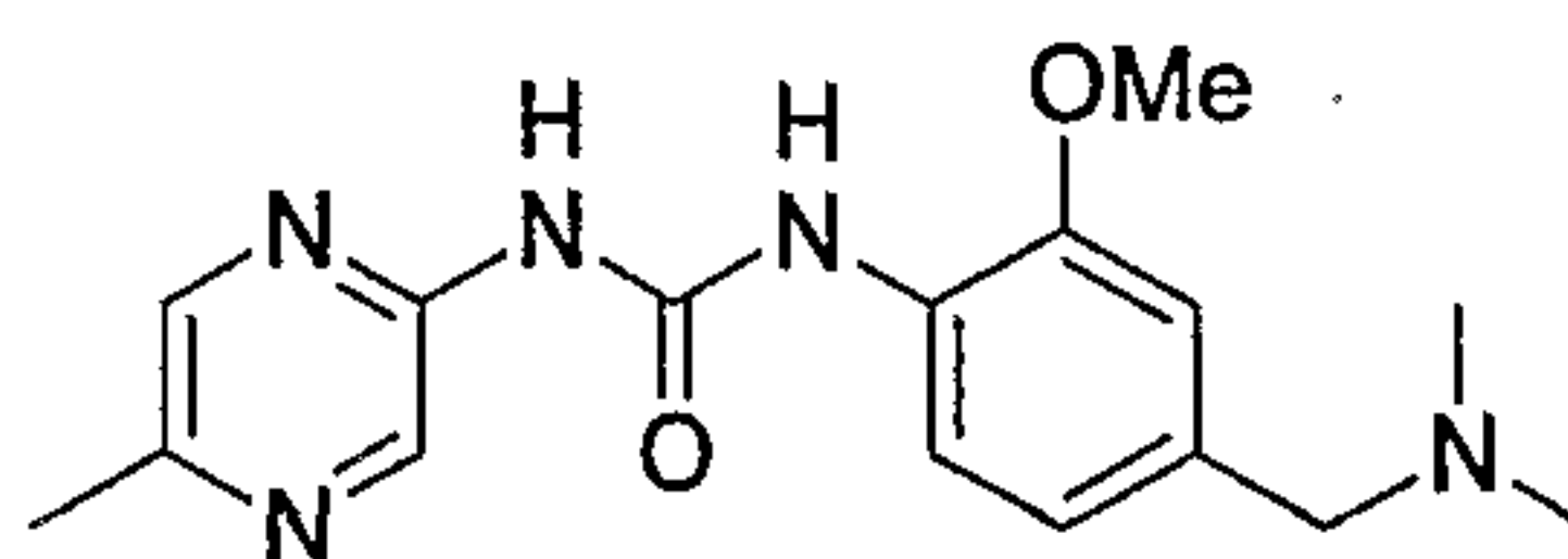
1-(4-Dimethylaminomethyl-2-methoxy-phenyl)-3-(5-methyl-pyrazin-2-yl)-urea
