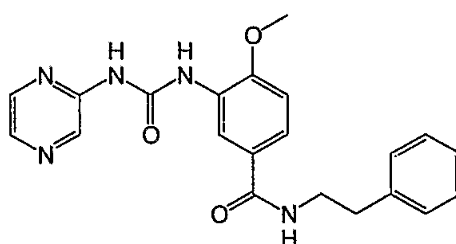
4-Methoxy-N-phenethyl-3-(3-pyrazin-2-yl-ureido)-benzamide
