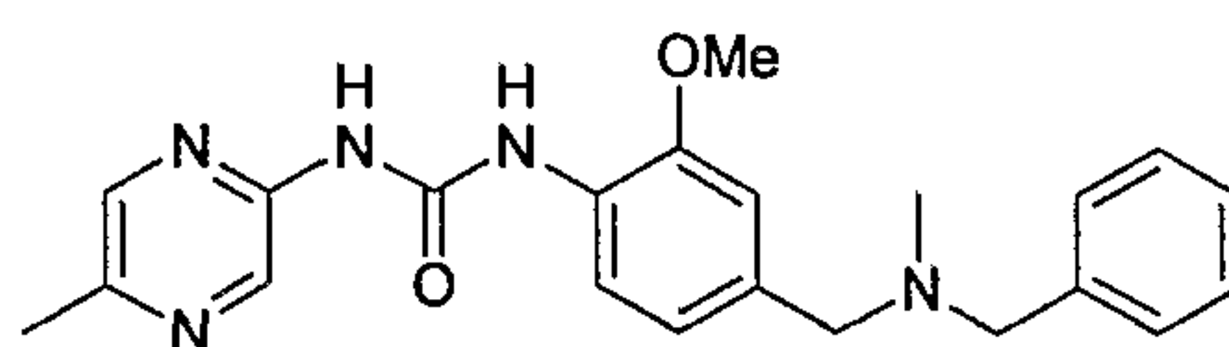
1-{4-[(Benzyl-methyl-amino)-methyl]-2-methoxy-phenyl}-3-(5-methyl-pyrazin-2-yl)-urea
