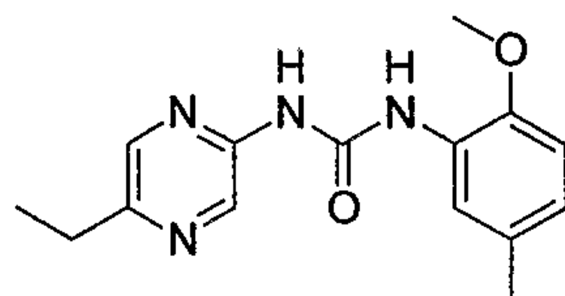
1-(5-Ethyl-pyrazin-2-yl)-3-(2-methoxy-5-methyl-phenyl)-urea
