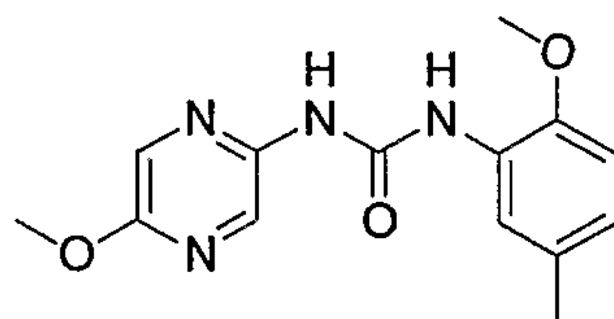
1-(2-Methoxy-5-methyl-phenyl)-3-(5-methoxy-pyrazin-2-yl)-urea
