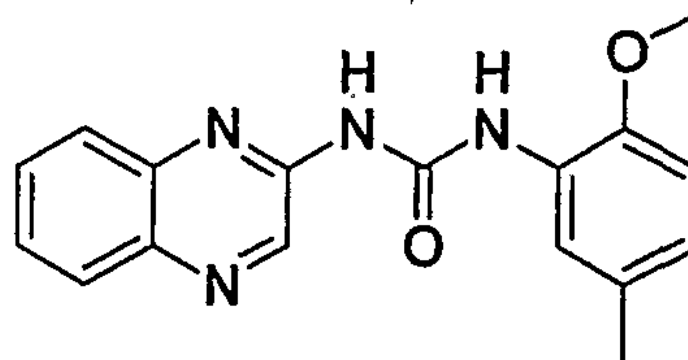
1-(2-Methoxy-5-methyl-phenyl)-3-quinoxalin-2-yl-urea
