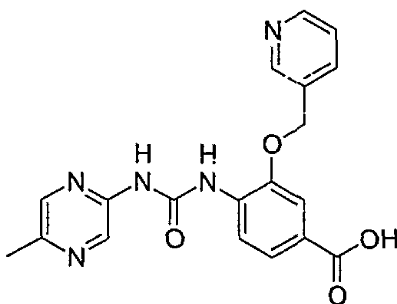
4-[3-(5-Methyl-pyrazin-2-yl)-ureido]-3-(pyridin-3-ylmethoxy)-benzoic acid
