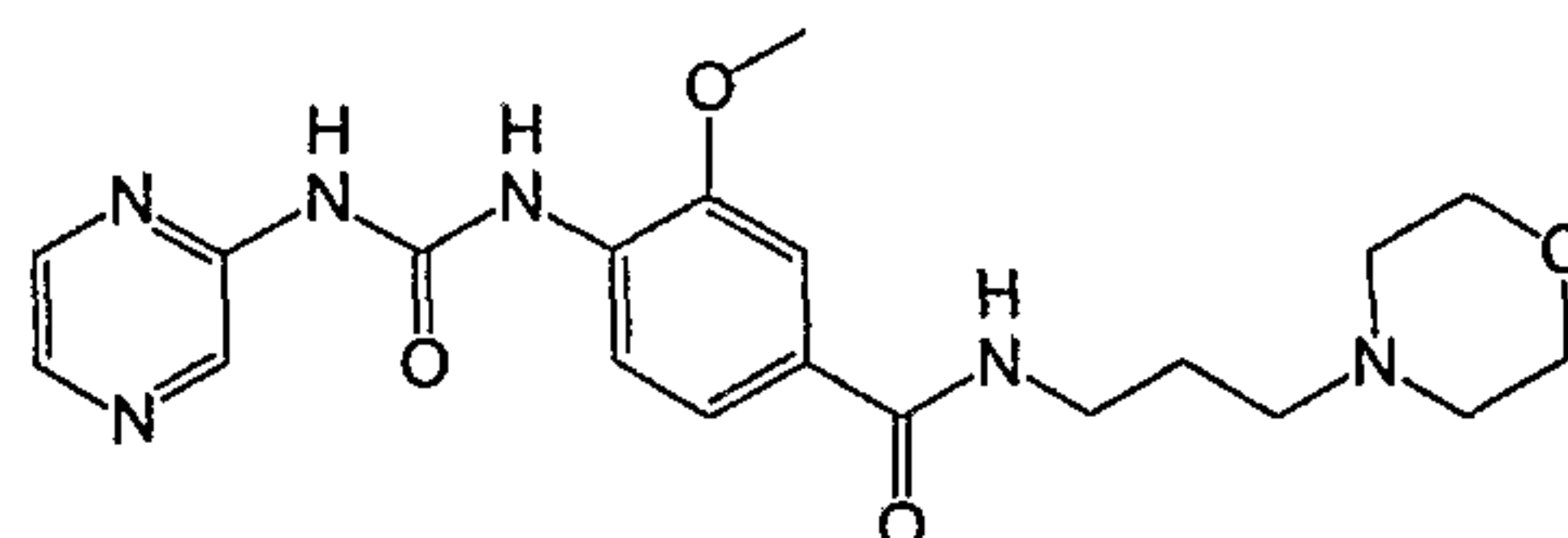
3-Methoxy-N-(3-morpholin-4-yl-propyl)-4-(3-pyrazin-2-yl-ureido)-benzamide
