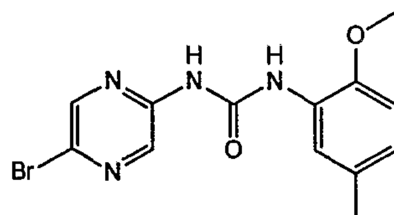
1-(5-Bromo-pyrazin-2-yl)-3-(2-methoxy-5-methyl-phenyl)-urea
