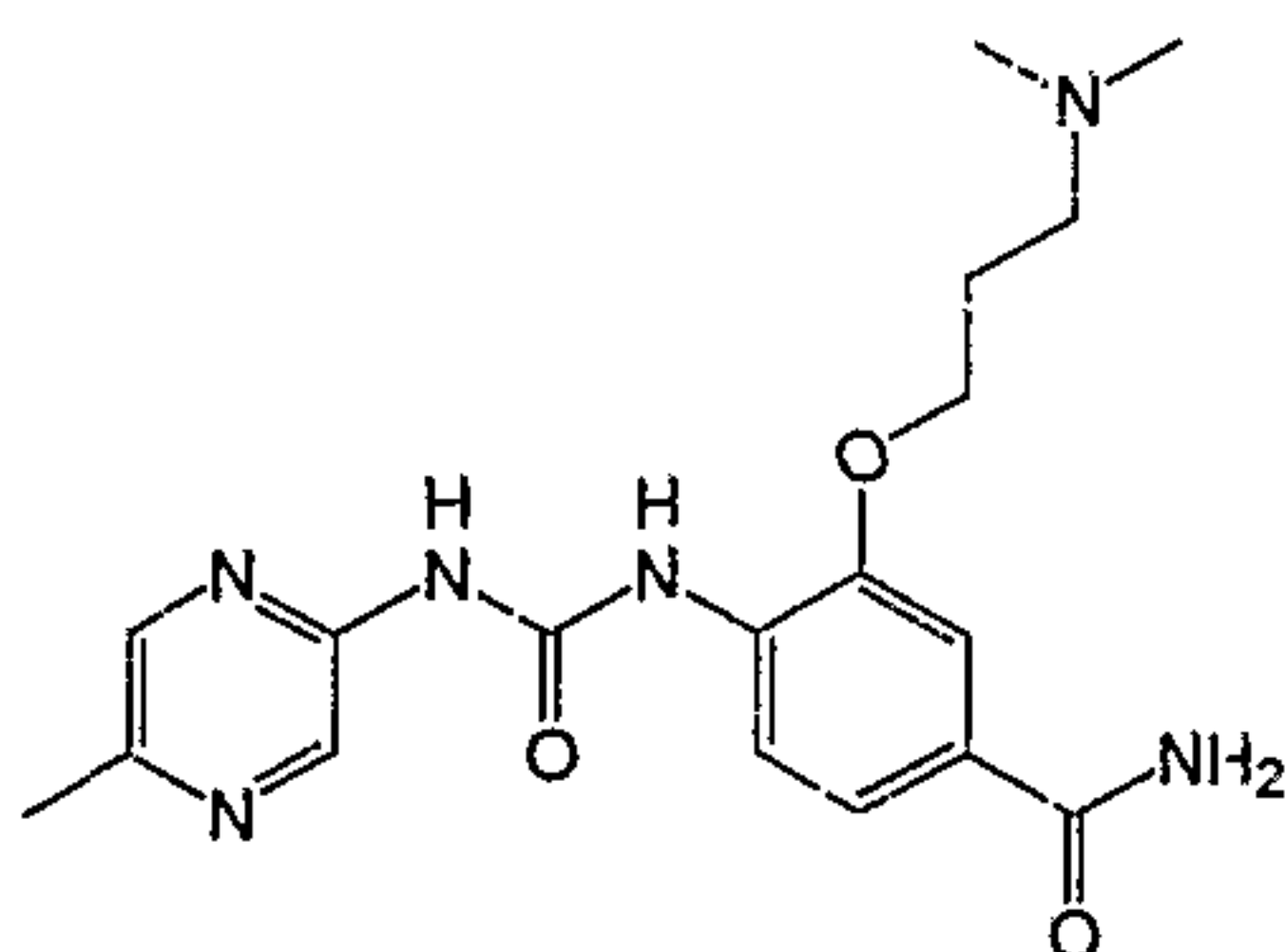
3-(3-Dimethylamino-propoxy)-4-[3-(5-methyl-pyrazin-2-yl)-ureido]-benzamide
