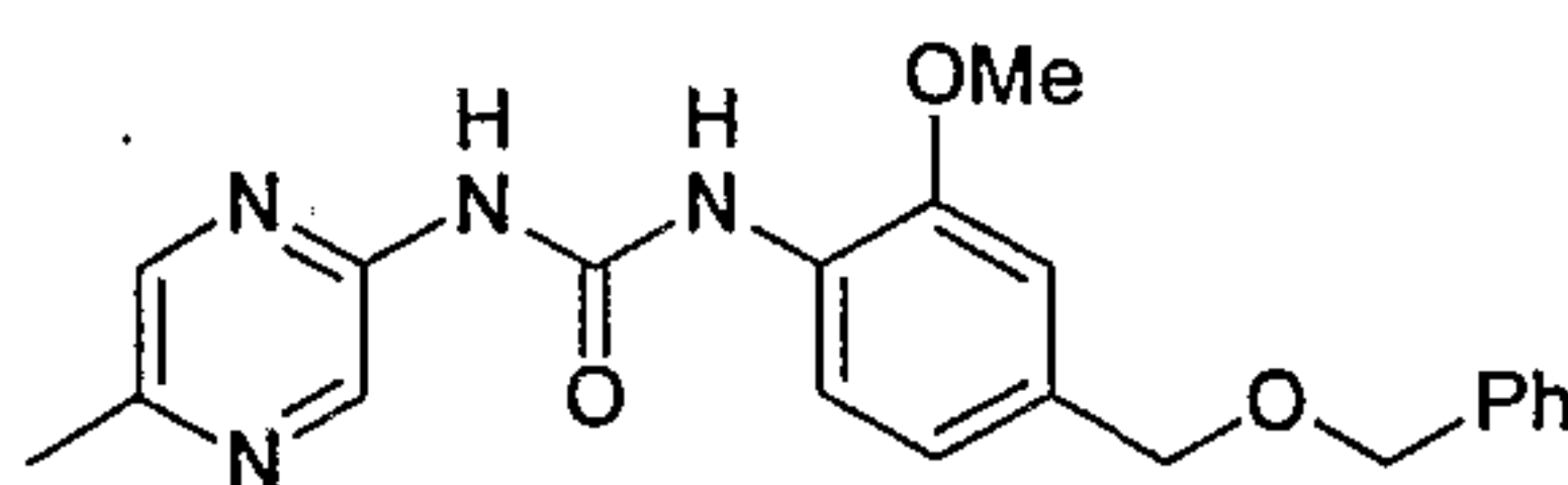
1-(4-Benzyloxymethyl-2-methoxy-phenyl)-3-(5-methyl-pyrazin-2-yl)-urea
