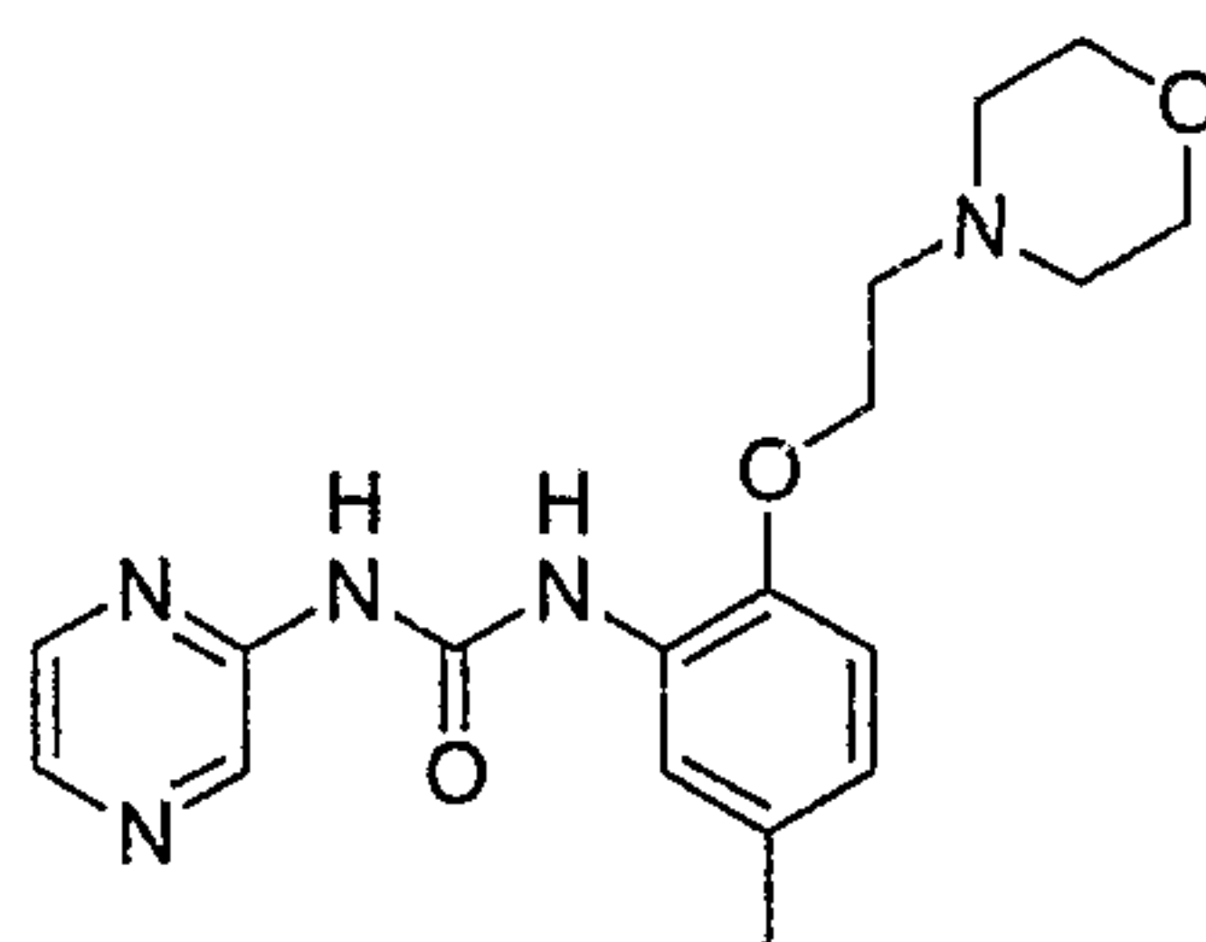
1-[5-Methyl-2-(2-morpholin-4-yl-ethoxy)-phenyl]-3-pyrazin-2-yl-urea
