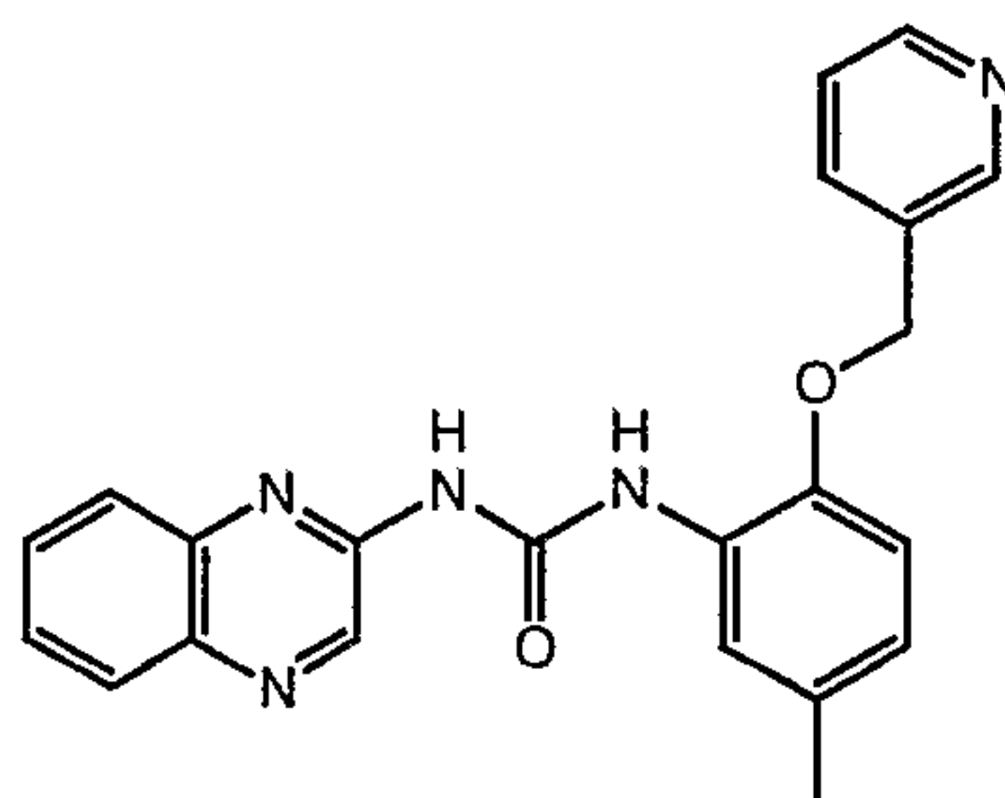
1-[5-Methyl-2-(pyridin-3-ylmethoxy)-phenyl]-3-quinoxalin-2-yl-urea
