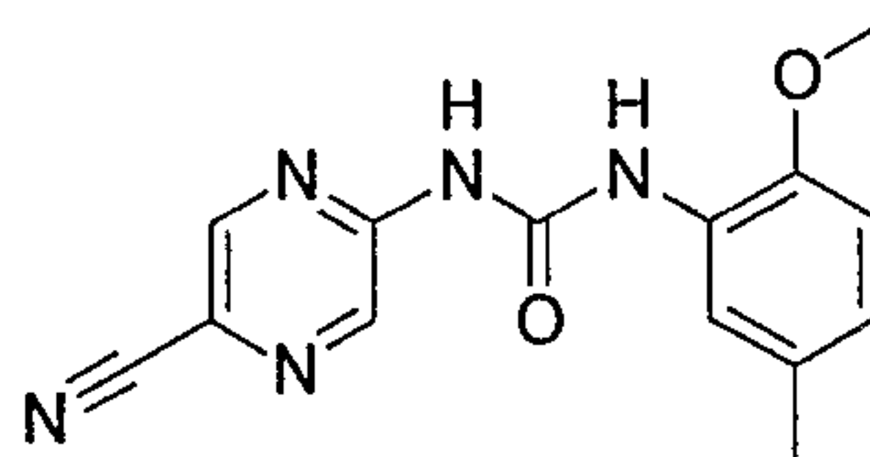
1-(5-Cyano-pyrazin-2-yl)-3-(2-methoxy-5-methyl-phenyl)-urea
