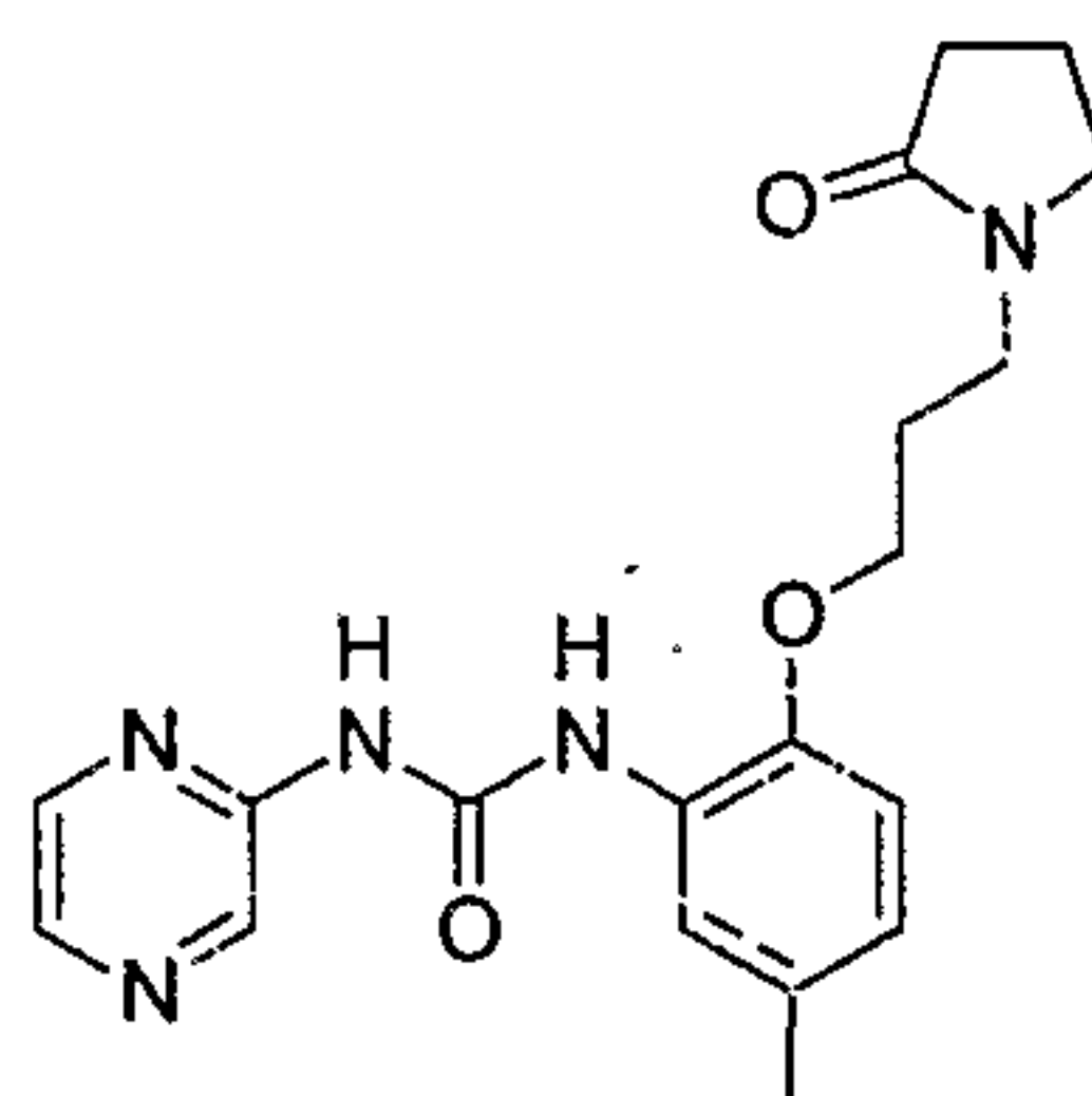
1-[5-Methyl-2-[3-(2-oxo-pyrrolidin-1-yl)-propoxy]-phenyl]-3-pyrazin-2-yl-urea
