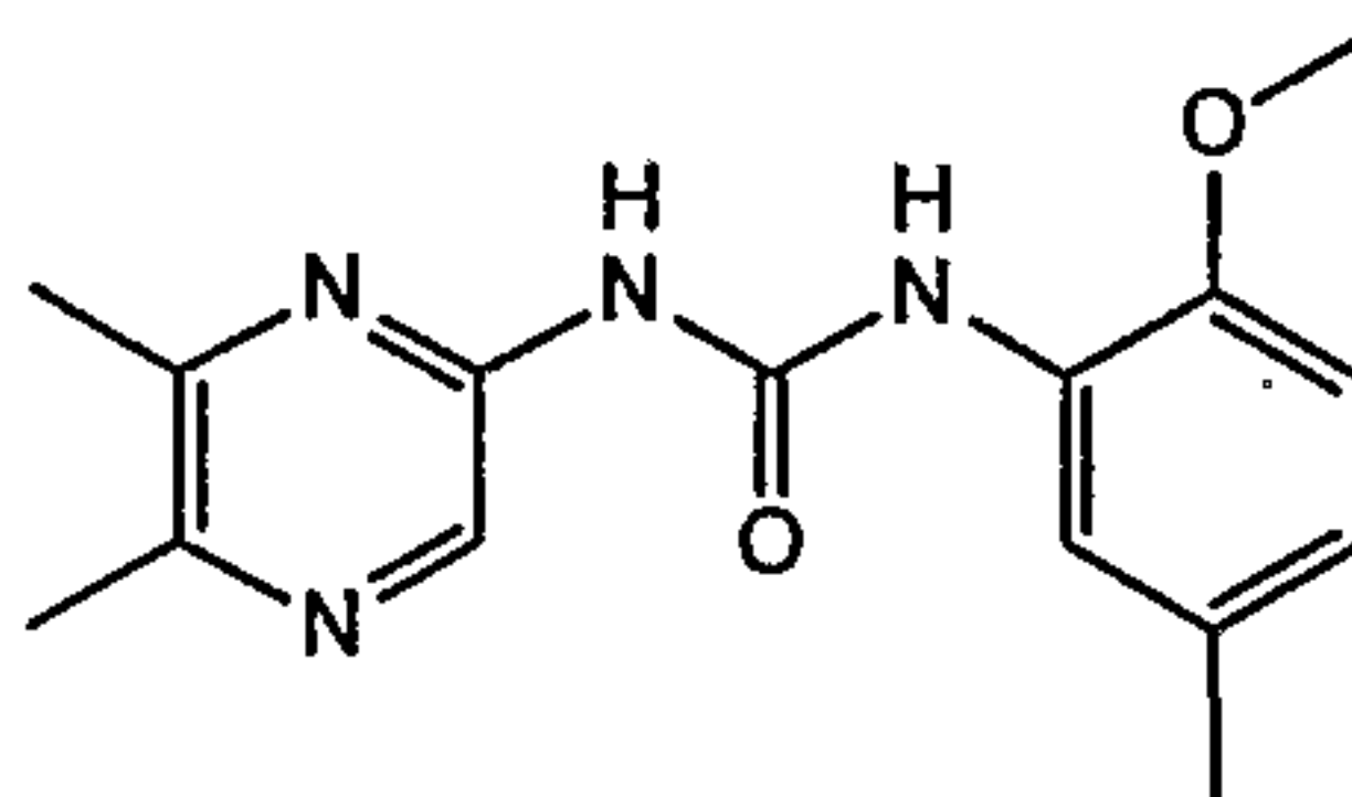
1-(5,6-Dimethyl-pyrazin-2-yl)-3-(2-methoxy-5-methyl-phenyl)-urea
