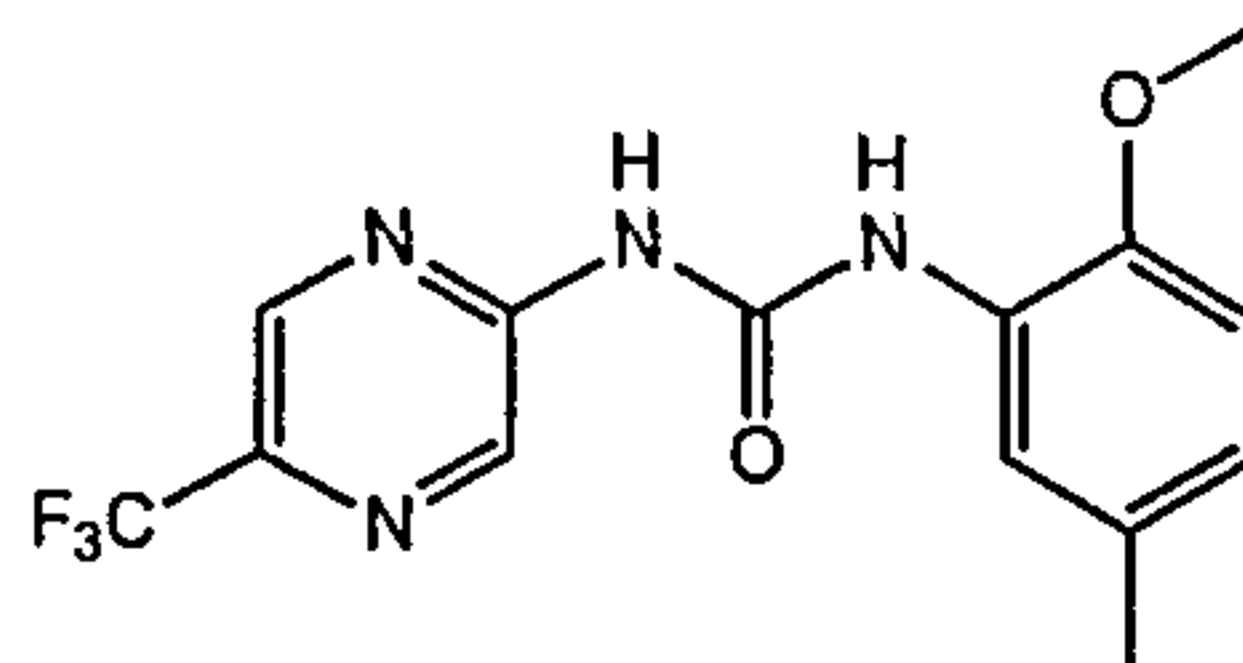
1-(2-Methoxy-5-methyl-phenyl)-3-(5-trifluoromethyl-pyrazin-2-yl)-urea
