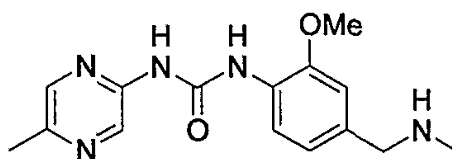
1-(2-Methoxy-4-methylaminomethyl-phenyl)-3-(5-methyl-pyrazin-2-yl)-urea
