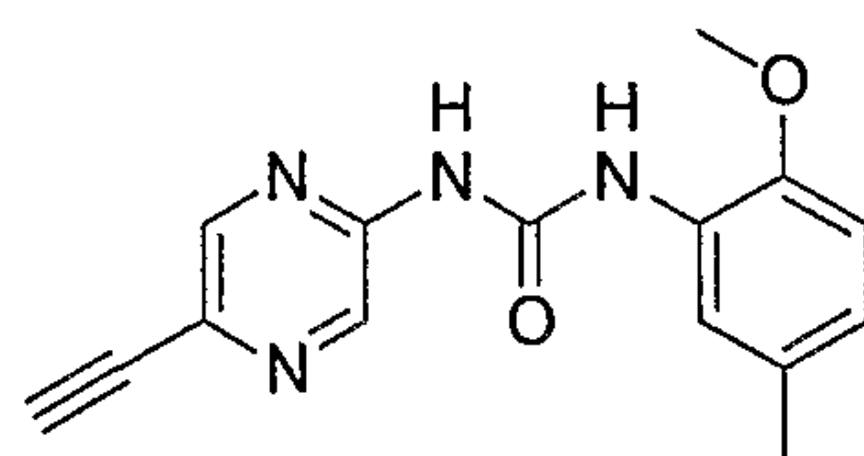
1-(5-Ethynyl-pyrazin-2-yl)-3-(2-methoxy-5-methyl-phenyl)-urea
