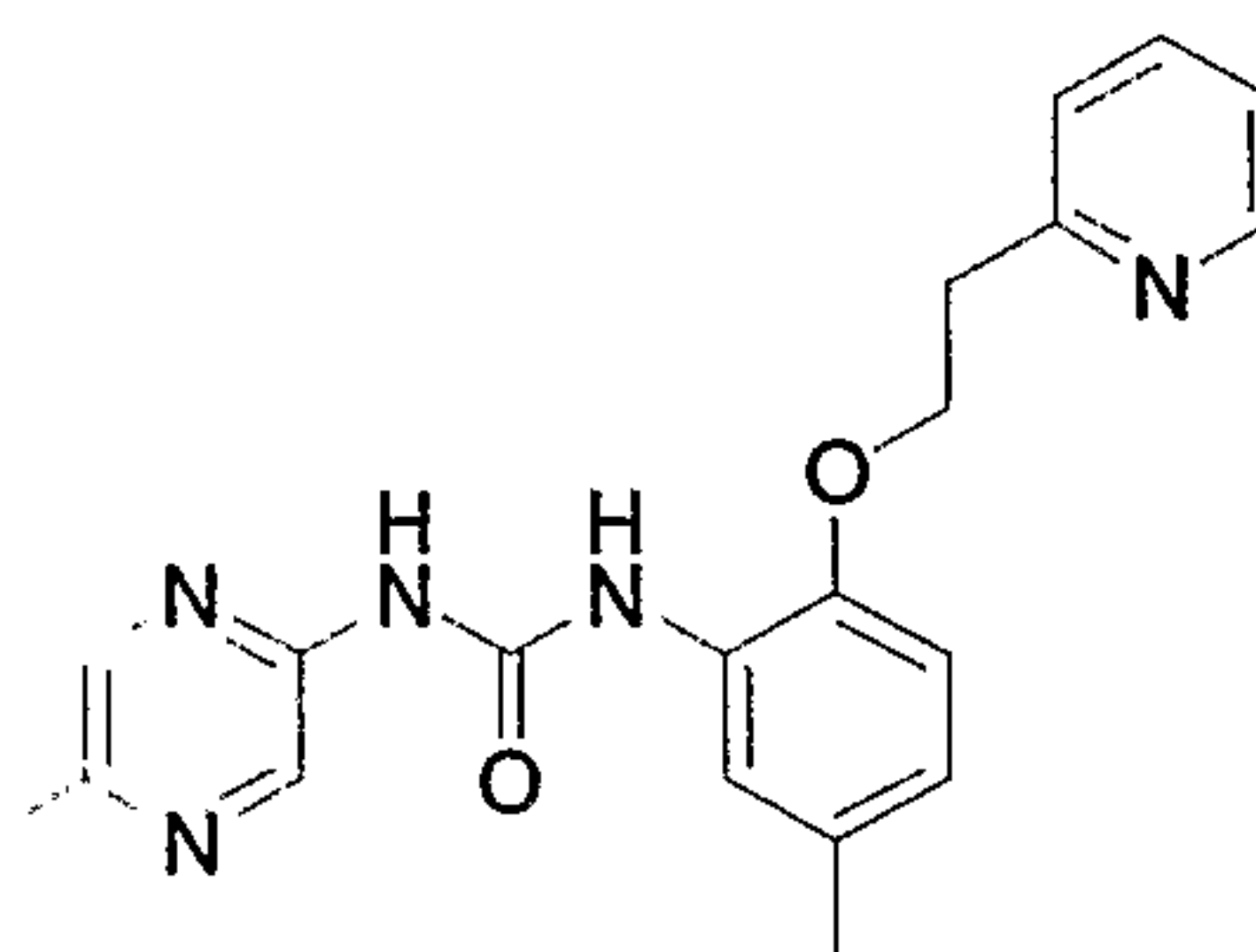
1-(5-Methyl-pyrazin-2-yl)-3-[5-methyl-2-(2-pyridin-2-yl-ethoxy)-phenyl]-urea
