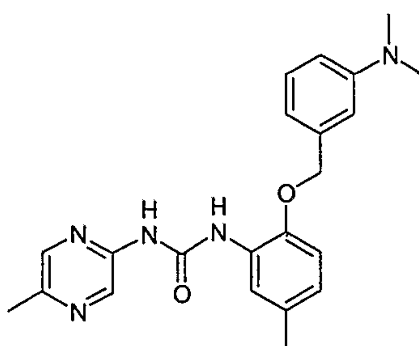
1-[2-(3-Dimethylamino-benzyloxy)-5-methyl-phenyl]-3-(5-methyl-pyrazin-2-yl)-urea
