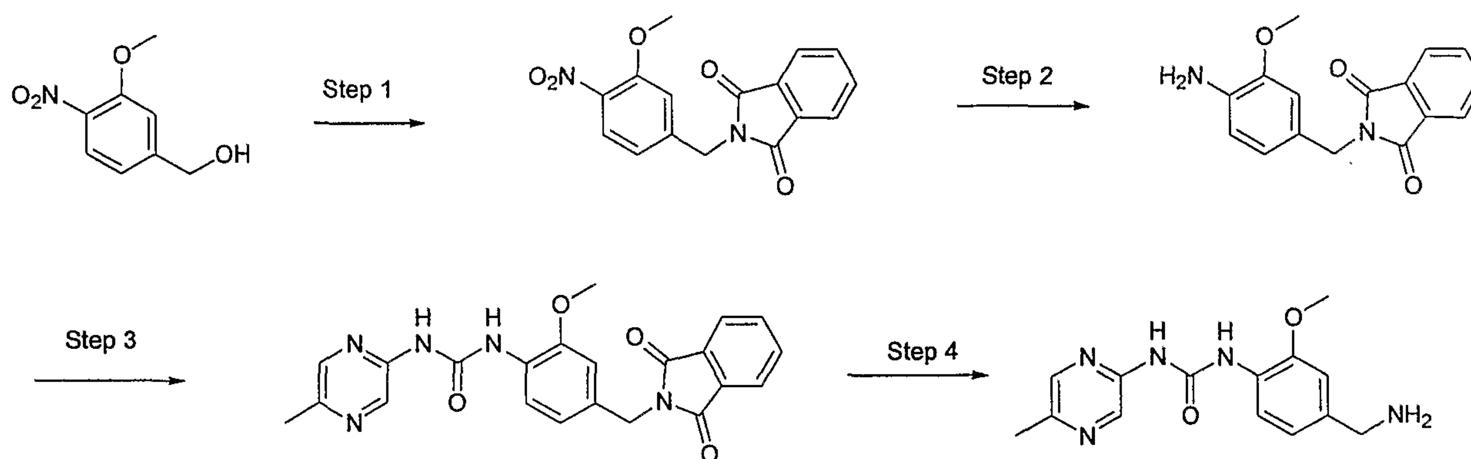
1-(4-Aminomethyl-2-methoxy-phenyl)-3-(5-methyl-pyrazin-2-yl)-urea
