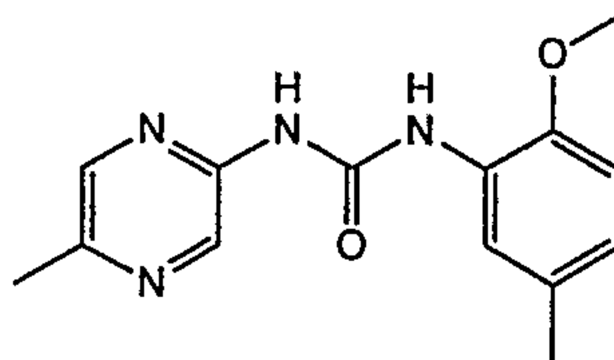
1-(2-Methoxy-5-methyl-phenyl)-3-(5-methyl-pyrazin-2-yl)-urea
