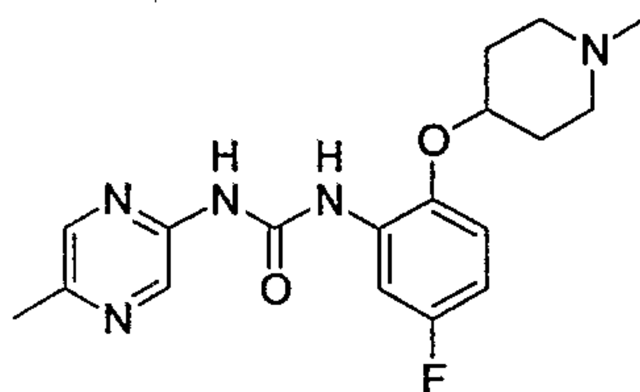
1-[5-Fluoro-2-(1-methyl-piperidin-4-yloxy)-phenyl]-3-(5-methyl-pyrazin-2-yl)-urea
