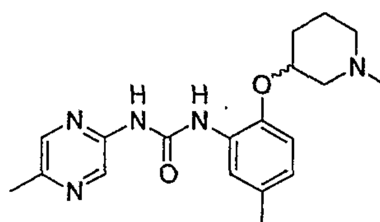
1-[5-Methyl-2-(1-methyl-piperidin-3-yloxy)-phenyl]-3-(5-methyl-pyrazin-2-yl)-urea
