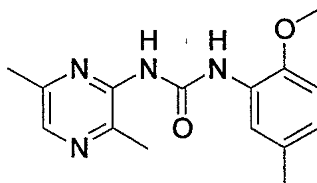
1-(3,6-Dimethyl-pyrazin-2-yl)-3-(2-methoxy-5-methyl-phenyl)-urea
