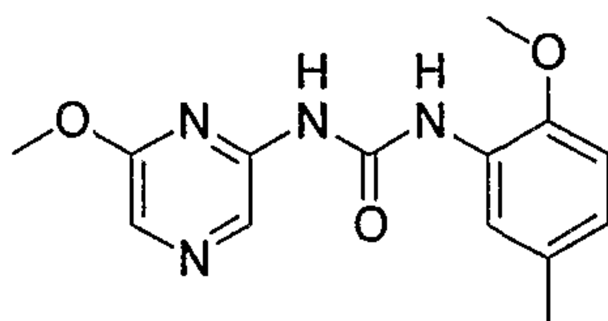
1-(2-Methoxy-5-methyl-phenyl)-3-(6-methoxy-pyrazin-2-yl)-urea
