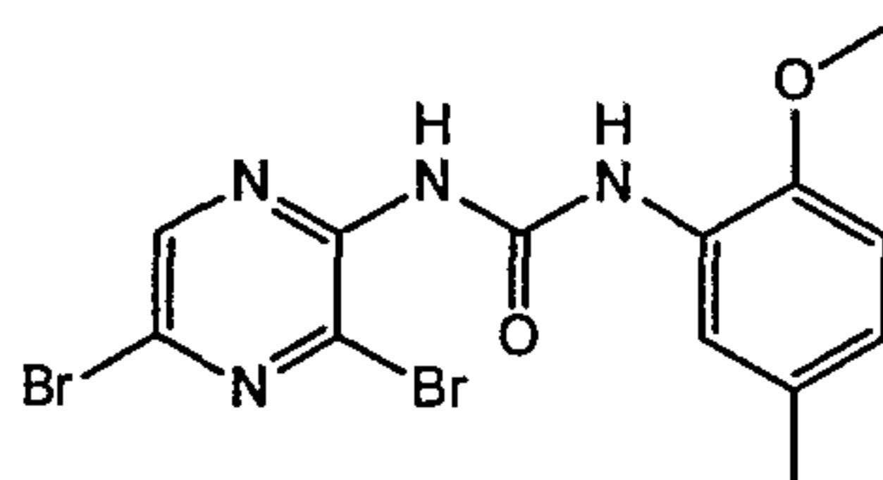
1-(3,5-Dibromo-pyrazin-2-yl)-3-(2-methoxy-5-methyl-phenyl)-urea
