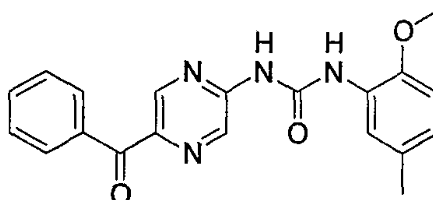
1-(5-Benzoyl-pyrazin-2-yl)-3-(2-methoxy-5-methyl-phenyl)-urea
