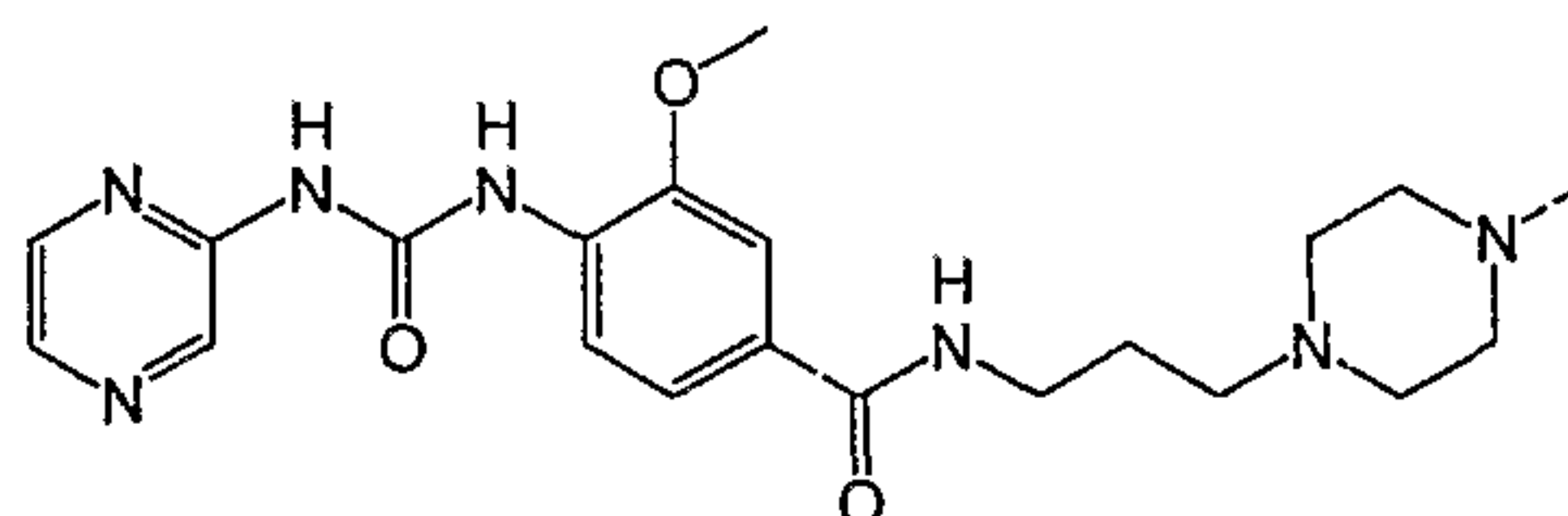
3-Methoxy-N-[3-(4-methyl-piperazin-1-yl)-propyl]-4-(3-pyrazin-2-yl-ureido)-benzamide
