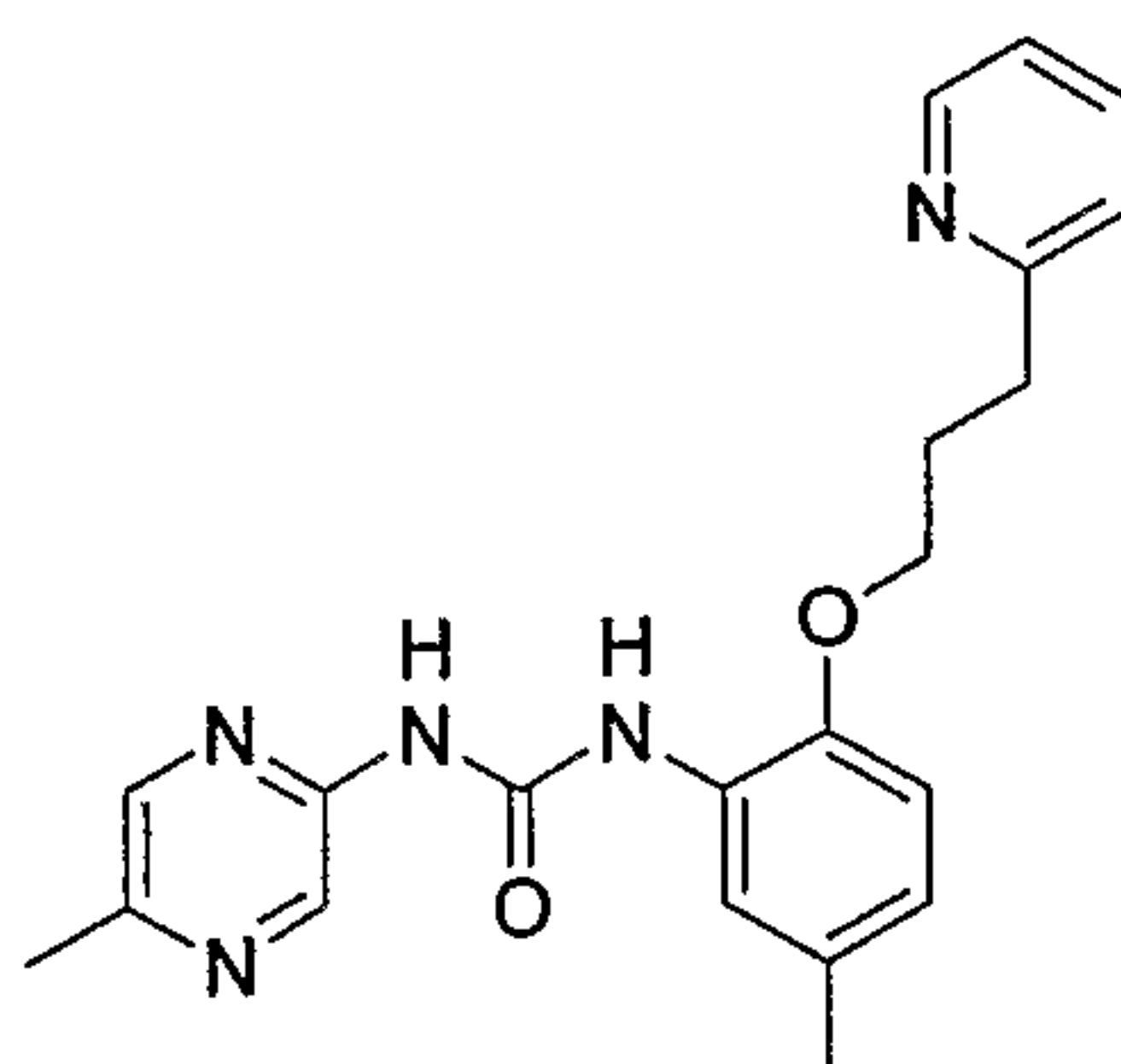
1-(5-Methyl-pyrazin-2-yl)-3-[5-methyl-2-(3-pyridin-2-yl-propoxy)-phenyl]-urea
