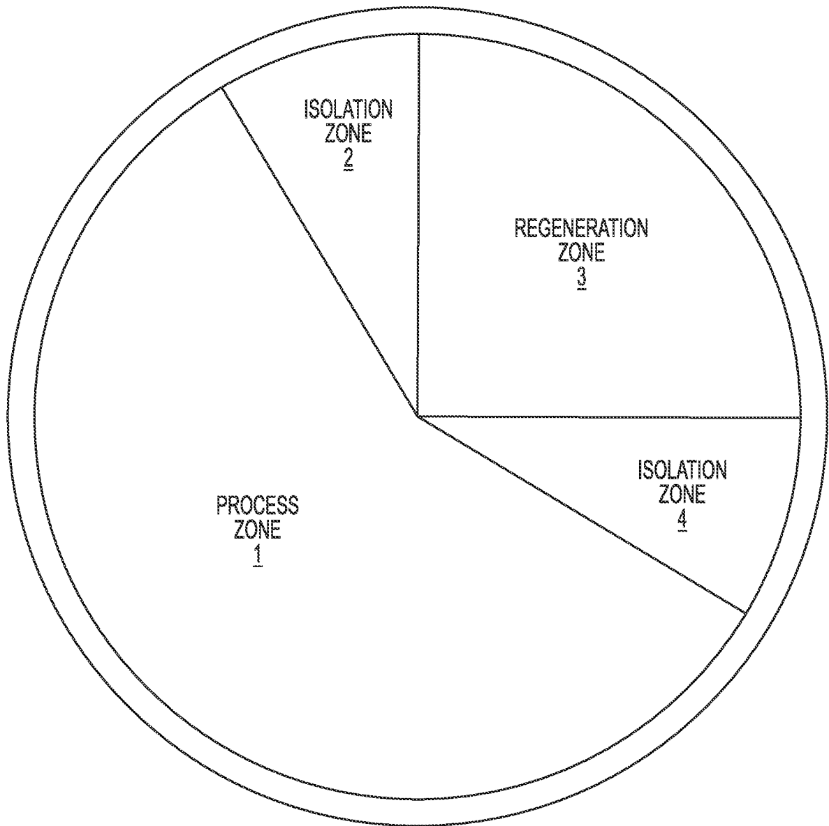
FIG. 6 (PRIOR ART)
