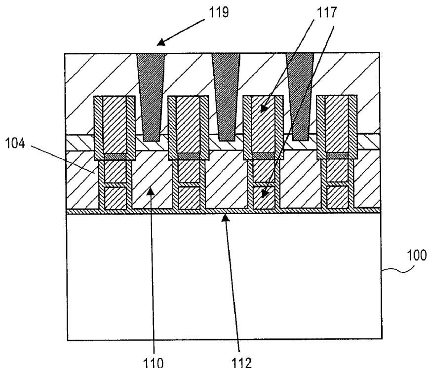
(a) NMOS
